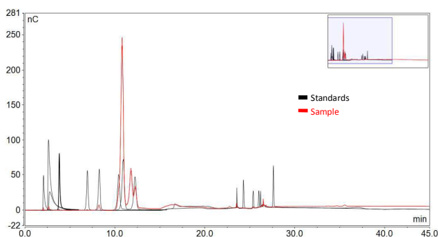
Fig. 3: Overlay of chromatograms from different standards and the spruce wood hydrolyzate. The spruce wood was hydrolyzed with a two-step acid hydrolysis. The obtained liquid was analyzed using the HPAEC-PAD method described here.
