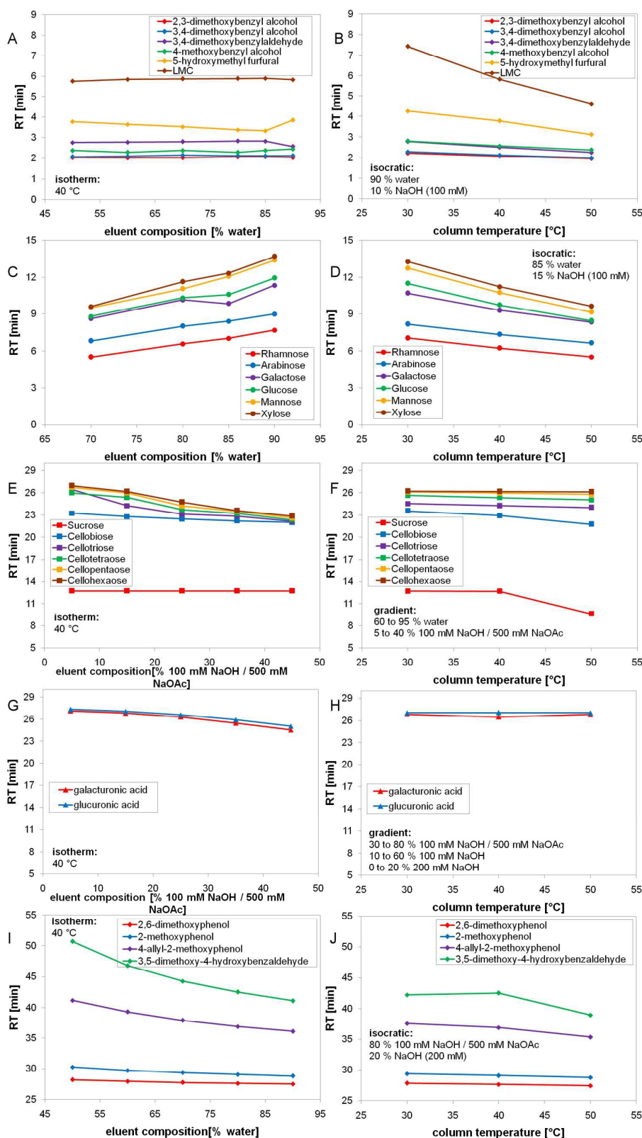
Fig. 1: Effect of eluent composition (A, C, E, G, I) and column temperature (B, D, F, H, J) on the retention time of acid-soluble biomass compound groups. The influence of the retention time for acid-soluble lignin compounds (A, B, I and J), monosaccharides (C and D), soluble oligosaccharides (E and F) and uronic acids (G and H) was investigated for both column temperature (in the range of 30–50 °C) and the eluent composition (water, sodium hydroxide and sodium acetate).
