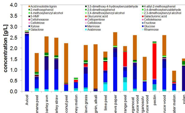
Fig. 4: Concentration of soluble compounds and acid insoluble lignin in the acid hydrolyzates of diverse biomasses. Concentration quantification of the specific soluble compounds was performed according to the developed HPAEC-PAD method. The theoretical maximum of concentration is 3 g biomass/L + the specifically added amount of water used for each polysaccharide hydrolysis step. For detailed information see tables S-1 and S-2.
