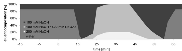
Fig. 2: HPAEC-PAD gradient. Gradient of four eluents (100 mM NaOH, 100 mM and 500 mM NaOAc, 200 mM NaOH and water) for the simultaneous determination of mono- and oligosaccharides, 5-HMF, uronic acids and acid-soluble lignin compounds.
