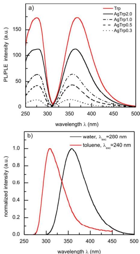
Figure 4. (a) Photoluminescence emission ( \lambda_{\text{exc}}=280 nm) and excitation ( \lambda_{\text{em}}=360 nm) spectra of 0.1 mM Trp aqueous solution (red line) and AgTrp colloids. (b) Normalized photoluminescence spectra of AgTrp2.0 colloids in water (black line) and toluene (red line).
