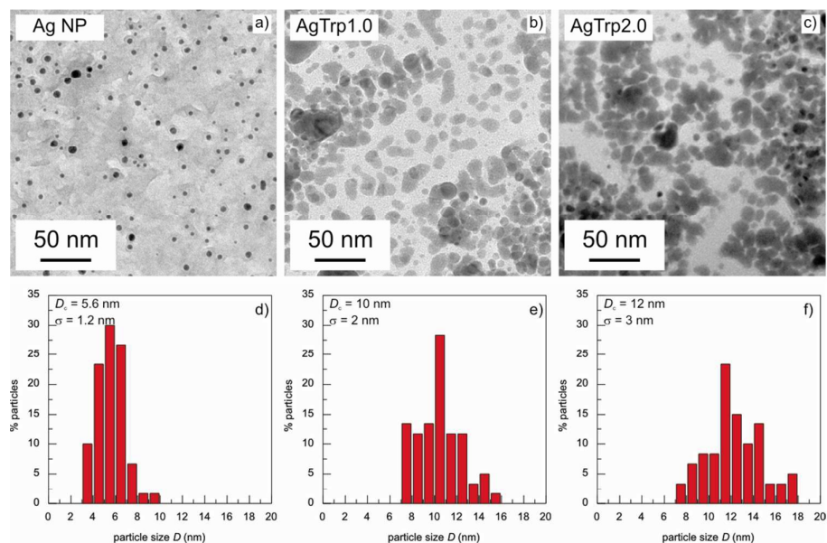
Figure 1. TEM images (a, b, c) and corresponding particle size distribution (d, e, f) of AgNP, AgTrp1.0 and AgTrp2.0 samples.
