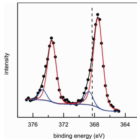
Figure 5. High resolution x-ray photoelectron spectra of Ag3d levels of the AgTrp1.0 sample. A vertical dashed line corresponds to the reference value of bulk silver. 35
