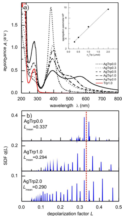
Figure 3. (a) UV-vis absorption spectra of AgTrp colloids and. The dependence of the aggregation parameter A_p on the amount of the amino acid in the colloid is given in the inset. (b) Spectral density functions for the absorption spectra of AgTrp colloids. Red dotted line presents the L=1/3 value that corresponds to spherical particles.
