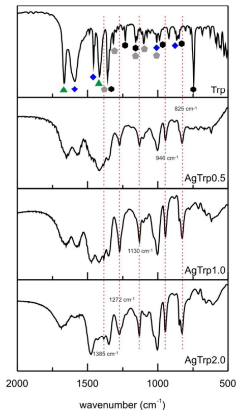
Figure 2. FTIR spectra of tryptophan and tryptophan functionalized silver nanoparticles. The symbols designate vibration modes pertaining to carboxyl (triangle), \alpha -amine (diamond), pyrrole (pentagon) and benzene (hexagon).
