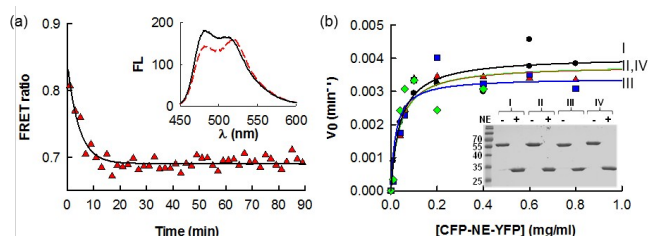
Fig. 2. (a) Decrease of FRET ratio as a function of time upon NE addition. The data were fit to a single exponential equation. Inset: emission spectra of sensor protein 3 after a 30 min incubation in the presence (red dashed line) or absence (continuous line) of NE. (b) Initial velocity of the NE-catalyzed reaction was measured as a function of the biosensor concentration in PBS buffer, pH 6.2 at room temperature (● = biosensor I, ▲ = biosensor II, ◆ = biosensor III, ■ = biosensor IV). Data were fit to the Michael-Menten equation. Inset: SDS-PAGE of the four biosensors before (-) and after (+) incubation with neutrophil elastase. Molecular weight markers are reported in kDa.
