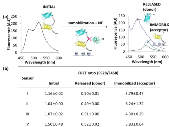
Fig. 3 (a) Fluorescence spectra of the NE-biosensor I before immobilization to a nickel coated plate (left), and after treatment with neutrophil elastase (right), and corresponding FRET ratio values (b). The immobilization was carried out in PBS pH 6.3 and elution was performed at a 100 mM imidazole concentration. All spectra were recorded with the proteins in solutions. The immobilized and released biosensor protein after treatment with NE where excited at 428 nm (purple and green curves, respectively), and the latter also at 485 nm (blue curve).
