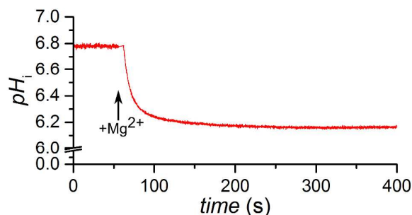
Fig. 4 pH-gradient generated by reconstituted H + -ATPase. The H + -pump activity trace for proteoliposomes from Fig. 3A was converted into pH i units (pH measured by fluorophores on the inside membrane monolayer only) as described in Supporting information.
