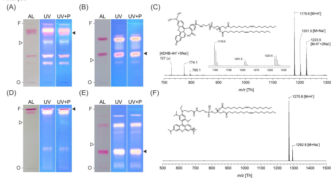
Fig. 1 Purification of lipid-conjugated pH-sensors. SNARF ® -1 carboxylic acid, acetate, NHS ester (upper panel, A-C) or pHrodo Red NHS ester (lower panel, D-F) was reacted with DOPE and the resulting derivatives were extracted and resolved by alkaline TLC (A and D, respectively). After extraction of the indicated region (filled arrowhead in A and D), the samples were resolved by acidic TLC (B and E, respectively), and the indicated region (filled arrowhead in B, resp. E) was extracted as final product. See Experimental for the composition of the used solvent systems. Chromatograms shown were dried completely before photographing under ambient light (AL) or UV light before (UV) and after staining with primuline (UV+P). The position of non-reacted DOPE is indicated by an open arrowhead. O, origin; F, solvent front, of the chromatograms. The final products were analysed by MALDI MS (C and F, positive ion mode). For lipid-conjugated SNARF (C), the annotated peaks correspond to the proton ( m/z 1179.6), the sodium ( m/z 1201.5), and H^+ + 2 Na^+ ( m/z 1223.5) adducts (insets: chemical structure of SNARF-DOPE and expanded section of the chromatogram). The characteristic matrix peak is indicated by an asterisk. For lipid-conjugated pHrodo (F), the annotated peaks correspond to the proton and the sodium adducts ( m/z 1270.8 and m/z 1292.8, respectively) (inset: chemical structure of pHrodo-DOPE; for pHrodo the chemical structure proposed by Ogawa 24 was used).
