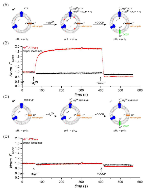
Fig. 3 Monitoring H + pumping by reconstituted H + -ATPase using lipid-conjugated pHrodo. (A) Illustration of the transport assay on proteoliposomes with reconstituted H + -ATPase. Addition of Mg 2+ to ATP-containing buffer initiated ATP hydrolysis and H + pumping into the vesicle lumen. Valinomycin was always present to mediate K + exchange and prevent the build-up of a transmembrane electrical potential. After reaching saturation conditions the H + gradient was disrupted by the addition of CCCP. Breaks in the traces denote intervals omitted for comprehensiveness. (B) Fluorescence changes for proteoliposomes (red) compared to empty liposomes (black) in the presence of ATP and Mg 2+ . For quantification of the changes in the vesicular pH see Supporting information, Fig. S6. (C) Illustration of a control experiment carried out in presence of AMP-PNP, a non-hydrolysable analogue of ATP. (D) Fluorescence changes for proteoliposomes (red) compared to empty liposomes (black) in the presence of AMP-PNP and Mg 2+ . For clarity, ATP/ATP-analogue additions were omitted in panel (B) and (D).
