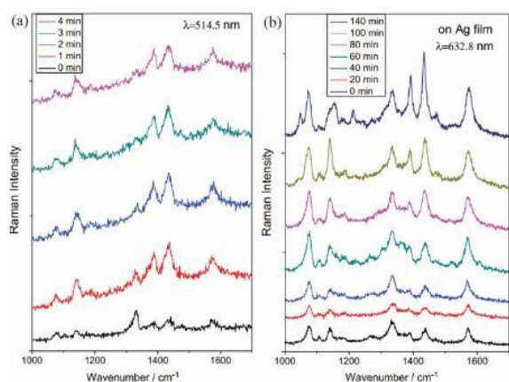
Fig. 3. Time dependent SERS measurement of pNTP adsorbed on Ag nanoparticles on Cu and Ag films, respectively. (a) on Cu film at 514 nm, and (b) on Ag film at 632.8 nm. The peak at 1332\text{ cm}^{-1} is attributed to the \text{NO}_2 vibration of pNTP and the peaks at 1140 , 1387 and 1432\text{ cm}^{-1} are attributed to \text{N}=\text{N} vibrations of DMAB. Adapted from ref. 47.
