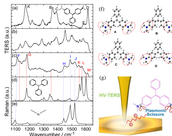
Fig. 12. Time dependent resonant TERS spectra of MG, (a) initial spectrum, (b) intermediate spectrum (20 minutes after continuous laser irradiation), (c) final spectrum (40 minutes after continuous laser irradiation), (d) and (e) simulated Raman spectra of MG fragments. (f) Vibrational modes of MG (corresponding to bands A-D in spectrum (a)) as calculated by density functional theory. (g) Sketch of proposed plasmonic scissors in resonant TERS. Adapted from ref. 75.
