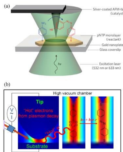
Fig. 8. Schematic of the plasmon catalyzed reaction of pNTP in TERS. (a) a monolayer pNTP adsorbed on gold nanoplate on glass was catalyzed to DMAB by TERS based on an AFM system. 73 (b) same plasmonic catalysis in HV-TERS based on a STM system. 74 Adapted from ref. 73 and 74.
