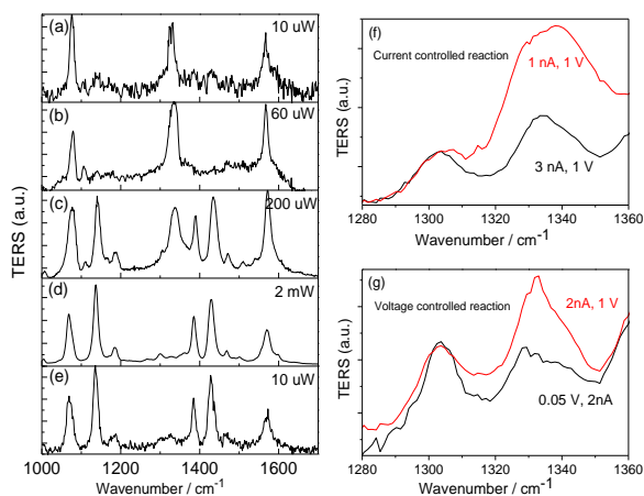
Fig. 9. Laser intensity and gap distance dependent TERS spectra. Laser intensity controlled plasmon catalyzed reaction of pNTP to DMAB at a power of (a) 10, (b) 60, (c) 200, (d) 2000 \mu\text{W} , and back to (e) 10 \mu\text{W} ; peak of pNTP at 1332 \text{cm}^{-1} can decrease when increasing the tunnelling current (f) or decreasing the bias voltage (g). Adapted from ref. 74
