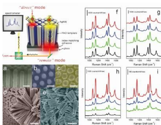
Fig. 6. Remote plasmonic catalysis by a silver nanowire array of PATP to DMAB. Left: scheme of the remote SERS sensor system (top), cross-section (a) and top views (b-e), and the scale bar is 100 nm in a-c, and 1 \mu\text{m} in d and e. Right: averaged SERS spectra by direct excitation (f and g) and remote excitation (h and i); (f and g) Gap of 11 nm with nanowire length of 920 nm (red). Image courtesy of Prof. Moskovits, adapted from ref. 44.
