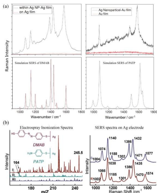
Fig. 4. Reaction of PATP to DMAB confirmed by SERS, surface mass spectrometry and theoretical calculations. (a) SERS spectra of PATP from nanoparticles on Ag and Au films, which agrees well
