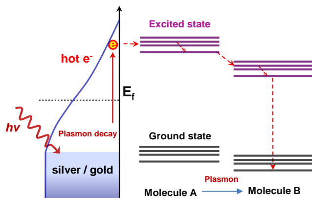
Fig. 1. Sketch of the plasmonic catalysis mechanism. Laser excitation of silver or gold nanostructures, generates hot electrons. Due to a plasmon decay the electrons can be transferred to an excited state of molecule A, from there a catalyzed reaction can be initiated to result in the final product, molecule B. Adapted from ref. 26.
