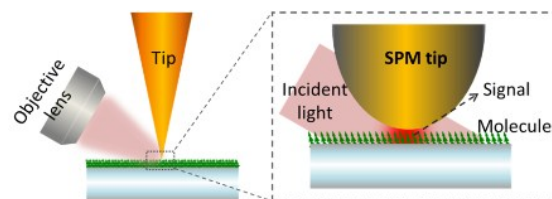
Fig. 7. Schematic TERS side-illumination setup. A long working distance objective links a Raman system (not shown) and focuses on the plasmonic tip; the enhanced signals originate predominantly from molecules in closest vicinity to the tip apex, which provides the high spatial-resolution analysis. Adapted from ref. 79.
