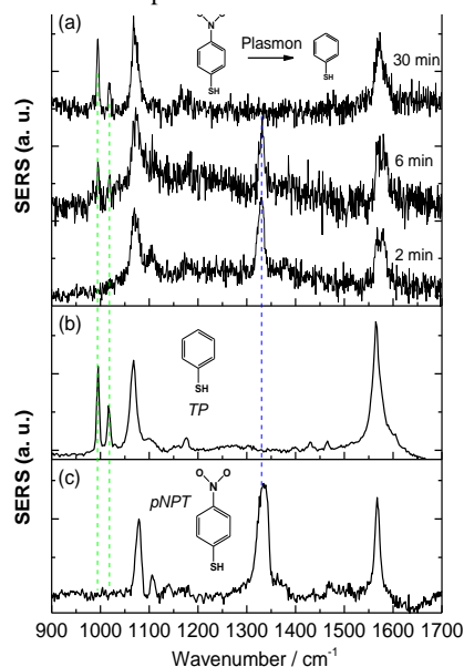
Fig. 13. Comparison of SERS spectra of pNTP and TP with spectra recorded during the experiment by a single gold dimer. (a) time dependent SERS spectra of reacted pNTP at 3 mW at 632.8 nm after 2, 6 and 30 min irradiation. Normal SERS spectra and corresponding molecular structures of TP and pNTP are shown in (b) and (c), respectively. Adapted from ref. 26.
