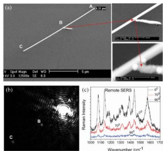
Fig. 5. Remote controlled plasmonic catalysis on a single silver nanowire. (a) SEM images of the remote system of Ag nanowire and nanoparticles, (b) the bright field optical image of PSPs propagating along the Ag nanowire if the incident polarization is parallel to the nanowire axis, (c) polarization angle dependent Re-SERS spectra, which collected at point B in the image of (a). Adapted from ref. 45.
