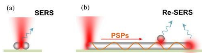
Fig. 2. Sketch of SERS and Re-SERS in an Ag nanoparticle-nanowire system. (a) Conventional SERS, the Raman signal is directly obtained from the nanoparticles. (b) Re-SERS signals are collected at the junction or end of a nanowire induced by the PSPs propagated along the nanowire when excited at the opposite end.
