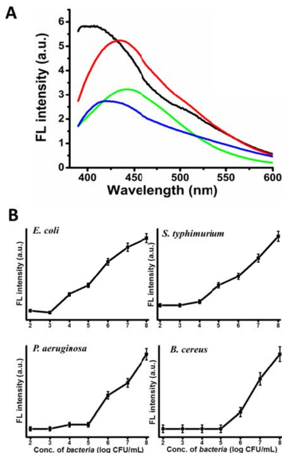
Fig. 4: A: Fluorescence emission spectra (excitation 350 nm) of bacterial cells labelled with the amphiphilic CDs. The spectra were recorded after incubating 10^8 bacterial cells in each case with the same concentration of amphiphilic CDs (1 mg/mL). Significant differences in fluorescence shifts and intensities are apparent among the bacterial strains: E. coli (black spectrum), S. typhimurium (red), P. aeruginosa (green), and B. cereus (blue). B: Detection sensitivity of amphiphilic carbon dot labeling assay. Graphs depicting the fluorescence signals (excitation at 350 nm) recorded in solutions containing different bacterial concentrations.
