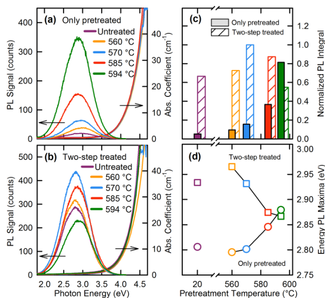
Figure 3. Steady-state 5 eV-excited PL spectra (left axis) and optical absorption (right axis) of 7.5Li 2 O-2.5Na 2 O-20Ga 2 O 3 -45GeO 2 -25SiO 2 before (a) and after (b) treatment of nanocrystallization at the exothermic peak extremum temperature T_c for 30 min, either in samples pretreated for 18 h at 560 °C, 570 °C, 585 °C, 594 °C, or not pretreated. (c) Dependence of PL intensity (from integration of spectra in (a) and (b)) on nucleation pretreatment temperature. (d) Dependence of PL band maximum (from spectra in (a) and (b)) on nucleation pretreatment temperature. Lines in (d) are guides for the eyes.
