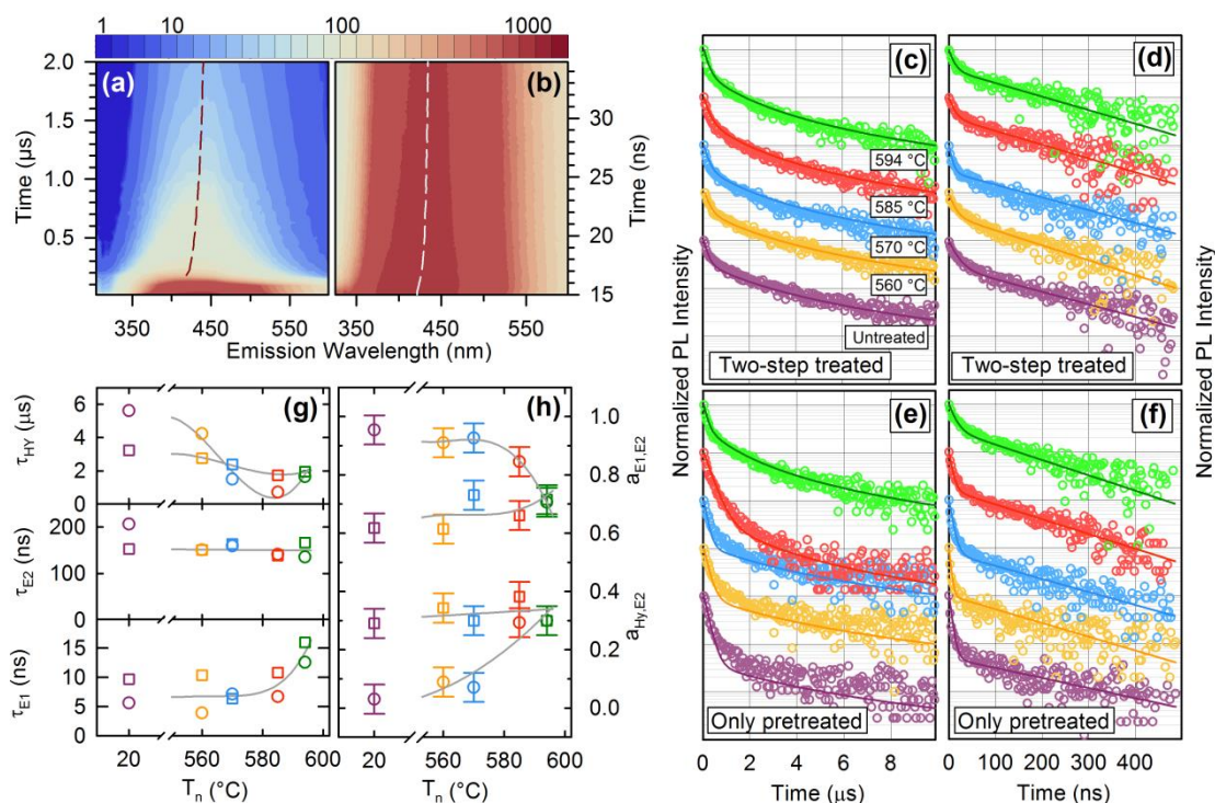
Figure 4. Representative time-resolved PL spectra excited at 250 nm in the (a) microsecond and (b) nanosecond domain of two-step treated 7.5Li 2 O-2.5Na 2 O-20Ga 2 O 3 -45GeO 2 -25SiO 2 sample pre-treated at 570 °C for 18 h. Dashed lines show PL band maximum shift vs. time. (c) Semi-log plot of PL decay curves (vertically shifted for clarity) in the \mu\text{s} domain (measured at 450 nm with excitation at 250 nm) and fitting curves, calculated according to Eq. 1, in nanocrystallized samples (after 30 min crystallization treatment at T_c ) either without (curve 1) or after nucleation treatment at the indicated temperatures. (d) PL decay curves in the ns domain of the same samples in (c) and fitting curves with Eq. 2. (e) PL decay curves in the ns and (f) \mu\text{s} domain in samples not subjected to crystallization treatment (labels as in (c) and (d) as regards nucleation pre-treatment). (g) Time decay constants of hyperbolic component ( \tau_{\text{HY}} ) and fast and slow exponentials ( \tau_{\text{E1}} and \tau_{\text{E2}} , respectively) from the fit of the decay curves in two-step treated (squares) and only-pretreated (circles) samples. (h) multiplicative factors in the fitting decay functions in Eqs. 1 and 2. Curves in (g) and (h) are guides for the eyes.
