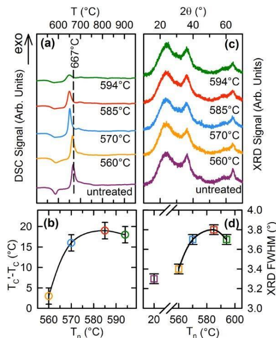
Figure 1. (a) DSC curves (vertically shifted for clarity) of glass with composition 7.5\text{Li}_2\text{O}-2.5\text{Na}_2\text{O}-20\text{Ga}_2\text{O}_3-45\text{GeO}_2-25\text{SiO}_2 before (untreated) and after nucleation pre-treatment at the indicated temperatures for 18 h. (b) Shift of the exothermic DSC peak maximum temperature T_c in pretreated samples (with respect to T_c of untreated sample) vs. nucleation pretreatment temperature T_n . (c) XRD patterns of the same samples (vertical order as in (a)) after subsequent treatment for 30 min at the exothermic peak temperature. (d) FWHM of \gamma\text{-Ga}_2\text{O}_3 XRD reflection at 36.3^\circ vs. nucleation pretreatment temperature T_n . Curves in (b) and (d) are guides for the eyes.
