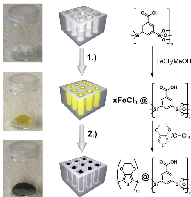
Figure 1. Two-step synthesis of PEDOT@UKON-2a: 1.) Infiltration of FeCl 3 into the mesopores; 2.) Polymerization of (3,4-ethylenedioxythiophene) inside the mesopores.
