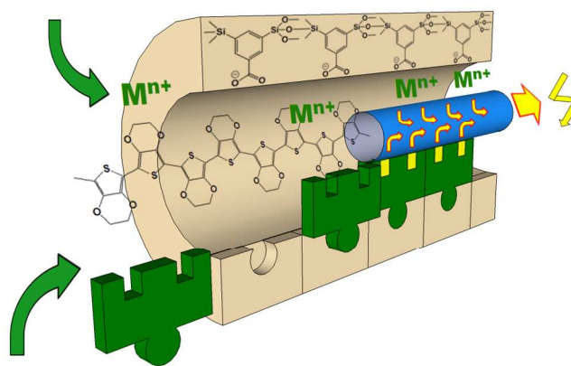
Scheme 1. Shown is one individual pore of a PMO material comprising benzoic acid in the pore walls (UKON-2a). 24 The -\text{COO}^- group can coordinate to various metal cations \text{M}^{n+} . 28 The conducting polymer PEDOT will be prepared inside the pores and it is expected that this enables electronic communication between the pore-walls and the conducting polymer.
