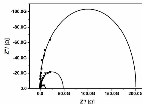
Figure 7. Impedance spectra (experimental data points and fit curve) for PEDOT@UKON2a treated at pH = 0 (dots), 2 (triangles) and 7 (squares).
