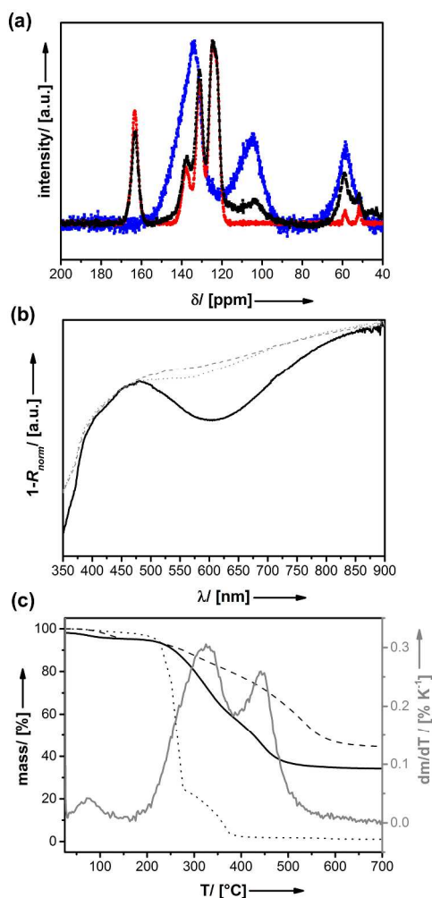
Figure 3. (a) 13 C solid-state NMR data of UKON-2a (red graph) and PEDOT (blue graph) as references and PEDOT@UKON-2a (black graph). (b) UV/VIS data of PEDOT@UKON-2a (black line), pure PEDOT (grey dotted line) and pure PEDOT obtained by dissolving PEDOT@UKON-2a (grey dashed line). (c) TGA data of UKON-2a (black dashed line), PEDOT (black dots) as references, PEDOT@UKON-2a (black line) and first derivative of the TGA data of PEDOT@UKON-2a (grey line).
