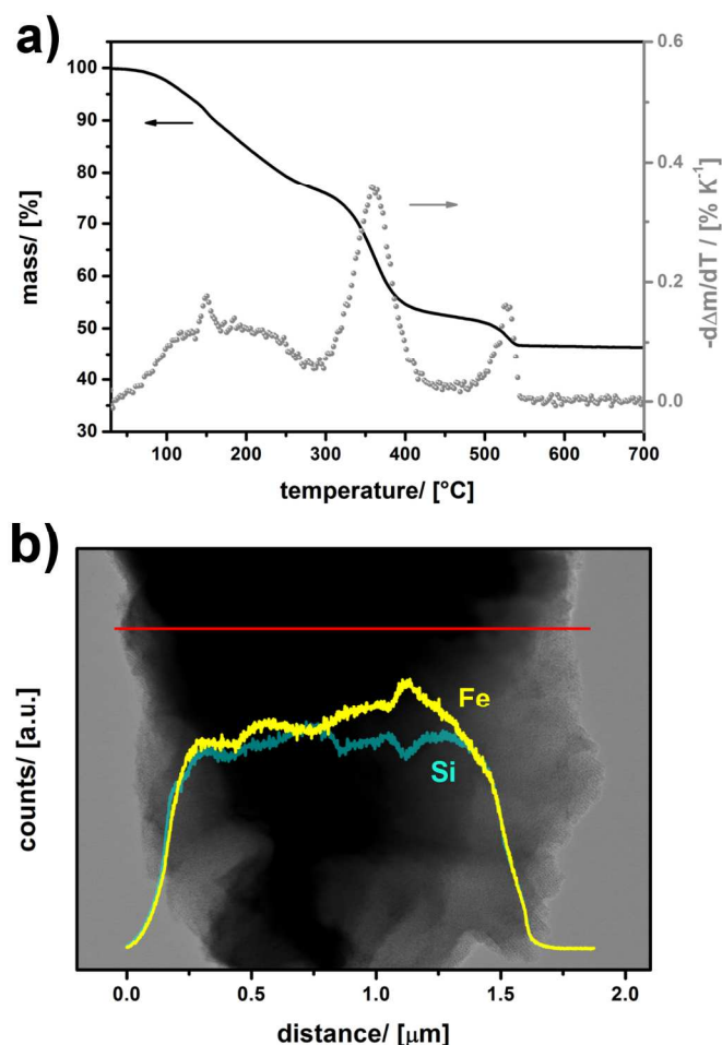
Figure 2. a) TGA data of FeCl 3 @UKON2a (black line) and differentiation of the TGA curve (grey dots). b) HR-TEM EDX-linescan data of FeCl 3 @UKON-2a.
