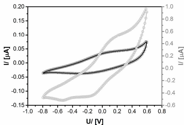
Figure 6. CV data of PEDOT@UKON2a (black) in comparison to Ru@PEDOTUKON2a (grey).
