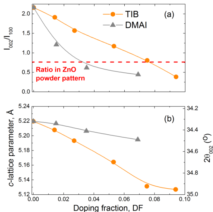
Fig. 7 (a) Intensity ratio I_{002}/I_{100} for the (002) and (100) peaks measured by XRD on the ZnO:X (X = Al, B) films reflecting the change in texture from \langle 002 \rangle to \langle 001 \rangle and (b) c -lattice parameter of the ZnO wurtzite unit cell and the corresponding 2\theta_{002} position of peak (002) as a function of the doping fraction in the ZnO:X (X = Al, B). The films were deposited at 150 °C on glass substrates. The c -lattice parameter of wurtzite ZnO crystal is 5.207 Å. 6
