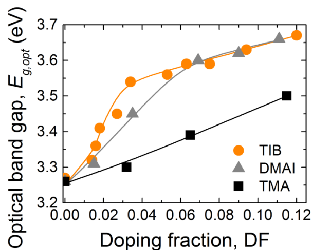
Fig. 11 Optical band gap ( E_{g,opt} ) as a function of DF for ZnO:X (X=Al, B). TIB was used as a B source while DMAI and TMA were used as Al sources. The films were deposited on SiO 2 substrates at 150 °C.
