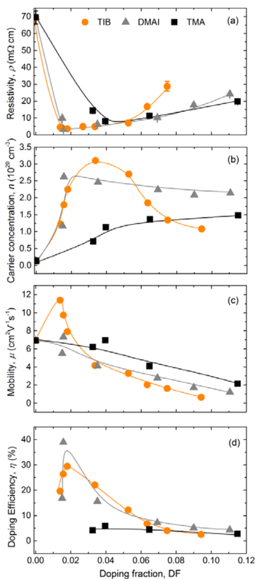
Fig. 4 Resistivity, \rho (a), carrier concentration, n (b), mobility, \mu (c) and doping efficiency \eta (d) of the ZnO:X ( X = \text{Al}, \text{B} ) films as a function of the doping fraction (DF) measured by XPS. TIB was used as a B source while DMAI and TMA were used as Al sources. All films had a thickness of 45 \pm 5 \text{ nm} and
