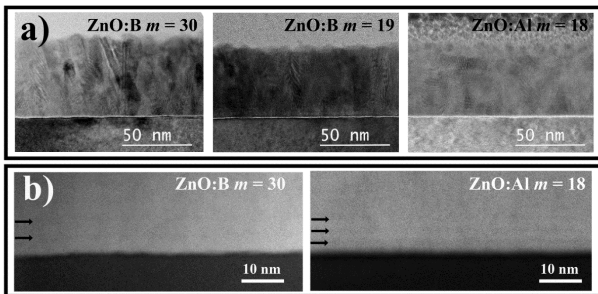
Fig. 8 Transmission electron microscopy images: a) bright-field (BF) TEM of two ZnO:B films ( m = 30 and m = 19 ) and a ZnO:Al film ( m = 18 ); and b) high-angle annular dark field (HAADF) STEM images of ZnO:B ( m = 30 ) and ZnO:Al ( m = 18 ). The B- and Al- doped layers are indicated by arrows.
