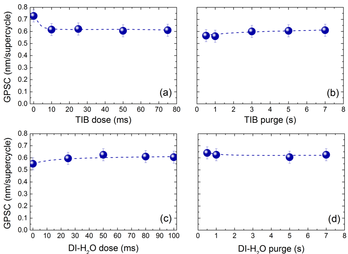
Fig. 2 Saturation curves of the ZnO:B process ( m = 4 ) at 150 \text{ }^\circ\text{C} . (a) TIB precursor dose, (b) TIB precursor purge, (c) DI- \text{H}_2\text{O} dose, and (d) DI- \text{H}_2\text{O} purge. The growth per supercycle (GPSC) for each condition was averaged over 10 supercycles. The ZnO standard conditions are specified elsewhere (50 ms DEZ dose, 5 s purge, 20 ms \text{H}_2\text{O} dose, 6 s purge) 35 and the process saturated at a GPC of 0.2 \text{ nm/cycle} for an intrinsic ZnO film deposited at 150 \text{ }^\circ\text{C} .
