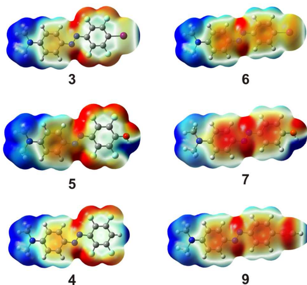
Fig. 2 Plots of the electrostatic potential of compounds 3 , 6 (top), 5 , 7 (mid) and 4 , 9 (bottom), computed at PBE0/6-311++G(d,p) level in vacuo . Potentials are mapped on the respective isosurfaces (0.001 a.u.) of electron density. Values of electrostatic potential range from -0.03 (red) to 0.03 (blue) a.u. Atom color scheme: C, gray; H, light gray; N, dark blue; O, red; F, sky blue, I, magenta.
