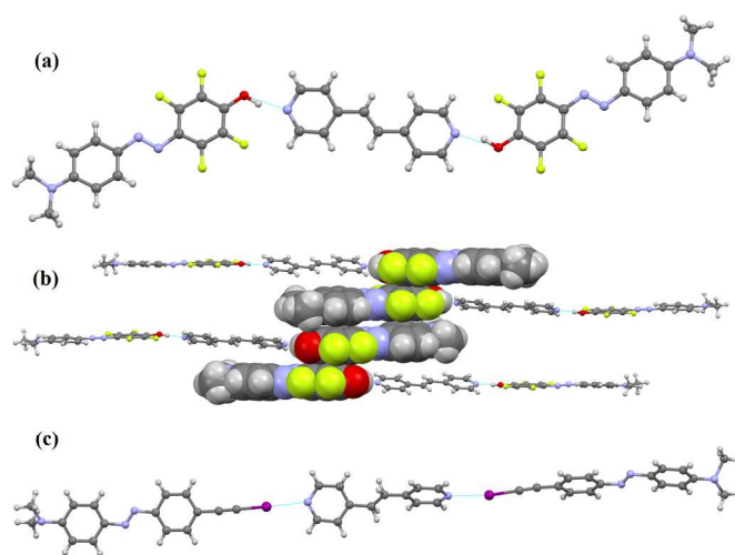
Fig. 3 (a) Ball-and-stick representation of a 10 ·( 5 ) 2 hydrogen-bonded trimer. The diazo-molecule is disordered by rotation of 180° around the O···N (amino) axis and only one of the two models is shown. (b) View along the crystallographic b -axis of four 10 ·( 5 ) 2 trimers. Four molecules of compound 5 , giving strong quadrupolar interactions, are shown in spacefill style. (c) Ball-and-stick representation of a 10 ·( 8 ) 2 halogen-bonded trimer. Both halogen-bond donor and acceptor are heavily disordered over two positions and here only one of the two models is represented. Hydrogen and halogen bonds are pictured as blue dotted lines. Colour code: carbon, grey; hydrogen, white; oxygen, red; nitrogen, blue, fluorine, green and iodine, purple.
