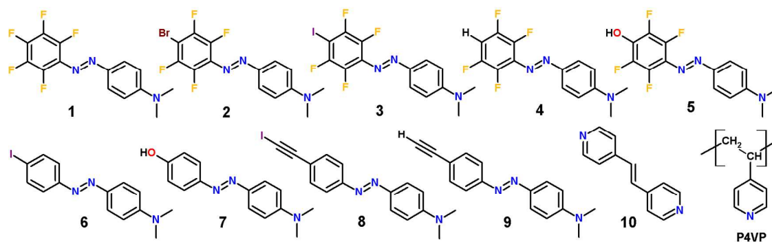
Fig. 1 Chemical structures of fluorinated azobenzene modules 1-5 , hydrogenated azobenzene modules 6-9 , model dipyridyl compound 10 used in the co-crystallization studies, and poly(4-vinyl pyridine) (P4VP), that was used as the polymer matrix for the azobenzene dyes.
