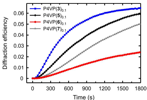
Fig. 5 Kinetics of the first-order diffraction efficiency upon the grating inscription process for P4VP( n ) 0.1 , where n = 3 (I is para to the azo group), 5 (OH is in para position), 6 (I is in para position on a non-fluorinated ring), and 7 (OH is in para position on a non-fluorinated ring).
