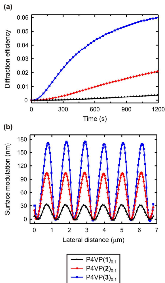
Fig. 4 (a) Kinetics of the first-order diffraction efficiency upon the grating inscription process, and (b) AFM surface profiles of the gratings for P4VP( n ) 0.1 , where n = 1 ( F is para to the azo group), 2 ( Br is para to the azo group), and 3 ( I is para to the azo group).
