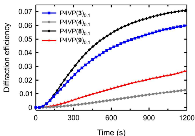
Fig. 6 Time evolution of the first-order diffraction efficiency upon SRG inscription process for P4VP( n ) 0.1 , where n = 3 (I is in para position), 4 (H is in para position), 8 (iodoacetylene is in para position), and 9 (acetylene is in para position).
