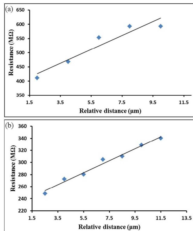
Fig. 6 (a) Plot of the calculated resistance of a DNA-templated Rh nanowires prepared by chemical reduction as a function of relative distance. Each i-V measurement carried out to calculate the distance-dependent resistance, was performed at a deflection setpoint value of 0.5V. (b) Resistance of electrochemically prepared DNA/Rh nanowires as a function of relative distance at deflection setpoint of 0.5V.
