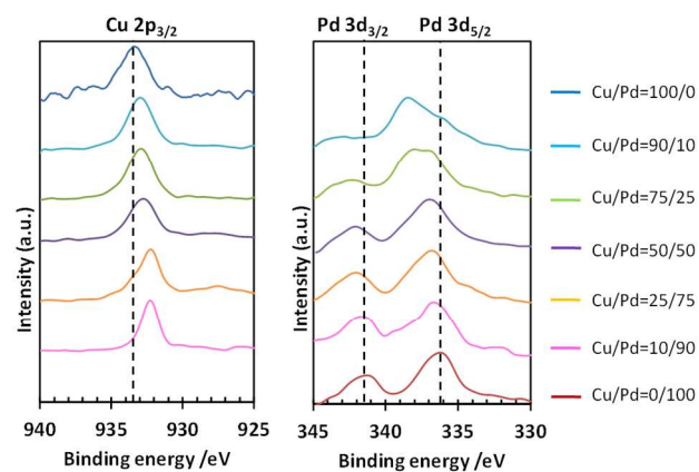
Figure 3. XPS core level spectra for Cu 2p_{3/2} and Pd 3d areas of Cu-Pd NPs with input feeding ratios for Pd increasing from top to bottom. Dashed lines mark the binding energy for (left) Cu 2p_{3/2} of Cu NPs (at 933.5 eV) and (right) Pd 3d_{5/2} and Pd 3d_{3/2} (336.2 and 341.4 eV, respectively) of Pd NPs.
