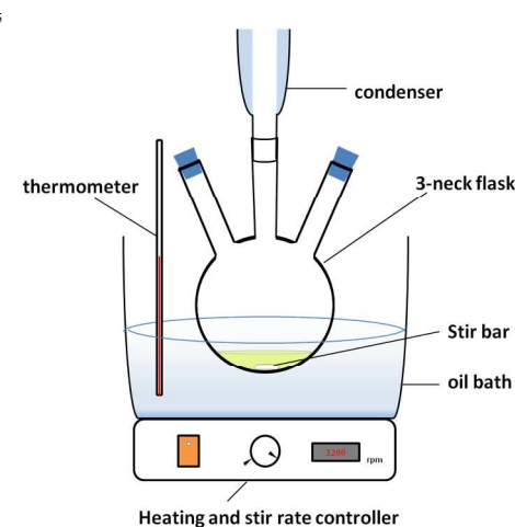
Figure 1. Experimental setup for synthesis of Cu-Pd NPs.
