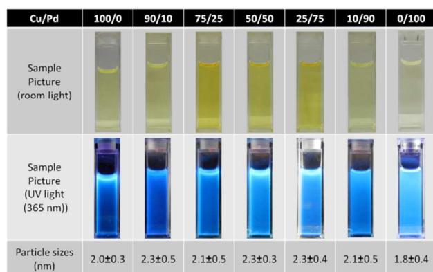
Figure 6. Photograph of Cu-Pd alloy NPs for various molar feeding ratios under room light (upper row) and under UV light of 365 nm (lower row).
