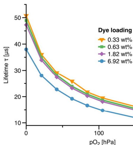
Figure 5. Calibration plots (at 25 °C) for oxygen sensors based on PtTPTBPBr 4 grafted to polystyrene ( 6a ) for varying amount of the immobilised indicator.
