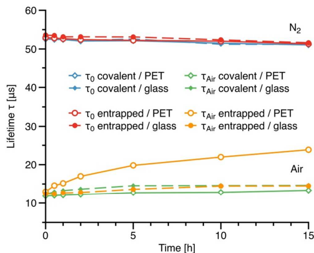
Figure 7. Influence of autoclavation (135 °C) on the luminescence decay times (at nitrogen and air saturation, measured at 25 °C) of the oxygen sensors based on 6b and on PtTPTBPBr 4 physically entrapped in polystyrene. Two different supports (PET and glass) are compared. The same sensor foils were autoclaved repeatedly throughout the whole experiment.
