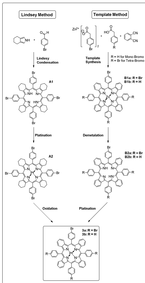
Figure 1. Synthetic approaches towards reactive bromo-modified Pt(II)-benzoporphyrins – commonly used Lindsey Condensation (left) and a modified Template-Method (right). Tetra-substituted porphyrin PtTPTBPr 4 was synthesized using both methods. Mono-substituted dye PtTPTBPr was prepared using template-method.
