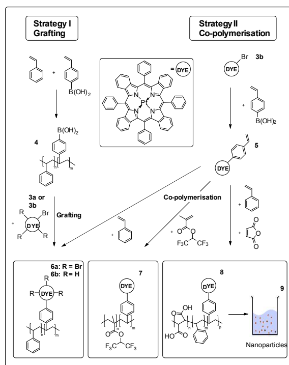
Figure 3. Two different strategies for covalent immobilisation of Pt(II)-benzoporphyrins based on C-C Suzuki-cross-coupling reaction. A co-polymer with boronic acid groups ( 4 ) can be used for covalent grafting of either using tetra- ( 3a ) or monobromo- ( 3b ) substituted benzoporphyrin. In the second strategy, the indicator is modified with styryl groups ( 5 ) and subsequent polymerisation with a variety of monomers is performed (styrene ( 6b ), 1,1,1,3,3,3-hexafluoroisopropylmethacrylate ( 7 ) or maleic anhydride and styrene ( 8 )). The latter can be used for the preparation of water dispersible nanoparticles ( 9 ).
