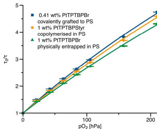
Figure 4. Stern-Volmer plots for polystyrene-based sensing materials at 25 °C. The fit is performed according to the eq. 1 (supporting information). The fit parameters are: f = 0.76 , K_{SV1} = 0.0298 \text{ hPa}^{-1} for covalently grafted PtTPTBPBr; f = 0.82 , K_{SV1} = 0.0249 \text{ hPa}^{-1} for copolymerised PtTPTBPStyr and f = 0.82 , K_{SV1} = 0.0228 \text{ hPa}^{-1} for physically entrapped PtTPTBPBr; K_{SV2} = 0.2K_{SV1} in all cases).
