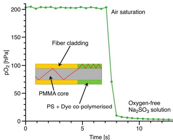
Figure 8. Cross-section and dynamic response of the fiber-optic oxygen sensor. The excitation light is coupled into a thin sensor layer coated onto the core of a PMMA fiber.
