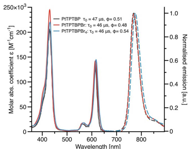
Figure 2. Absorption (in dichloromethane) and Emission spectra (in deoxygenated toluene) for the new Pt(II)-benzoporphyrin complexes.
