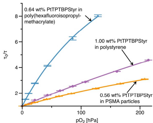
Figure 6. Stern-Volmer plots for sensing materials based on co-polymerised 5 at 25 °C. The fit parameters are: f = 0.90 , K_{SV1} = 0.110 \text{ hPa}^{-1} , K_{SV2} = 0.0041 \text{ hPa}^{-1} for poly(hexafluoroisopropylmethacrylate); f = 0.82 , K_{SV1} = 0.0249 \text{ hPa}^{-1} , K_{SV2} = 0.0050 \text{ hPa}^{-1} for polystyrene and f = 0.73 , K_{SV1} = 0.0183 \text{ hPa}^{-1} , K_{SV2} = 0.0050 \text{ hPa}^{-1} for PSMA particles.
