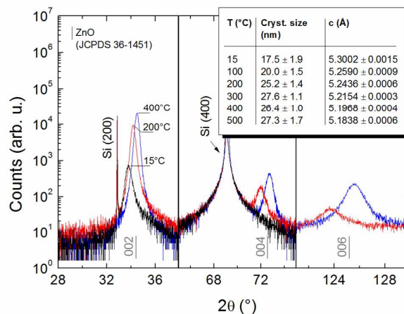
Fig. 1 – X-ray diffractograms of ZnO:Nd thin film deposited at different temperatures. The inset shows the crystallites' size and the lattice parameter along the growth direction for all deposition temperatures. No (006) peak has been observed for the sample grown at 15 °C and the relative data have been omitted for clarity.
