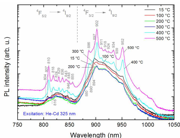
Fig. 2 – NIR PL emission spectra of ZnO:Nd thin films deposited at different temperatures and excited by the 325 nm line of a He-Cd laser. Two bands associated to radiative transitions between the ^4F_{5/2} and ^4F_{3/2} excited states to the ^4I_{9/2} fundamental state multiplet can be distinguished. The approximate position of the individual lines is also indicated.
