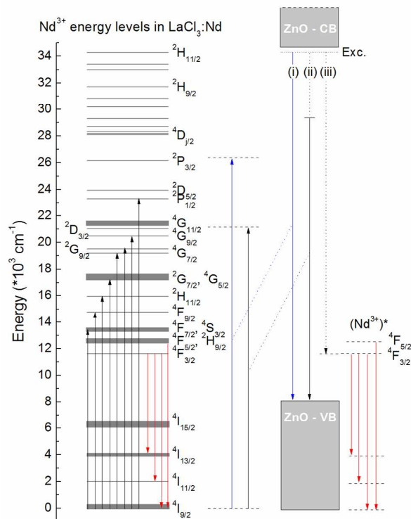
Fig. 8 - Observed radiative transitions of \text{Nd}^{3+} in ZnO and possible energy transfer mechanisms from the host. The energy levels of \text{Nd}^{3+} in \text{LaCl}_3 are reported for reference 18 .
