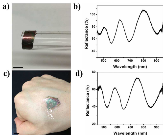
Fig. 6 A free-standing etalon transferred to (a) a glass tube, and (c) skin. (b,d) The reflectance spectra obtained from the devices. The scale bar is 0.5 cm.
