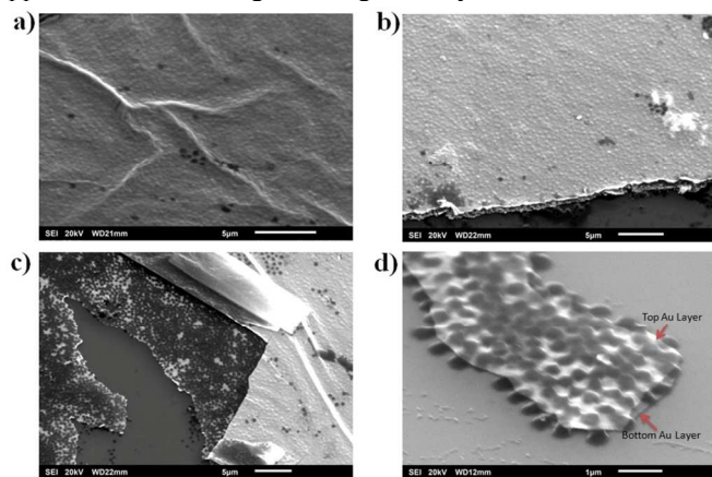
Fig. 4 SEM images of a free standing etalon from: (a,c) the top, (b,d) tilted 30^\circ . As can be seen in (a,b), the etalon structure remained intact after desorption from the solid substrate, and the microgels remained sandwiched between the two Au layers. As can be seen in (c), there are
