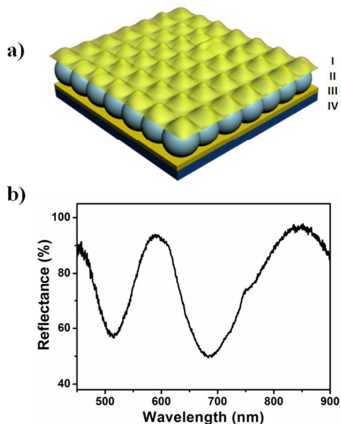
Fig. 1 a) Basic construct of a microgel-based etalon. (I) and (III) are 15 nm Au layers (a 2 nm Cr adhesion layer below the Au layer is not shown); (II) monolithic pNIPAm-co-AAc microgel layer; and (IV) glass substrate. b) Characteristic reflectance spectrum for a pNIPAm-co-AAc microgel-based etalon in water.
