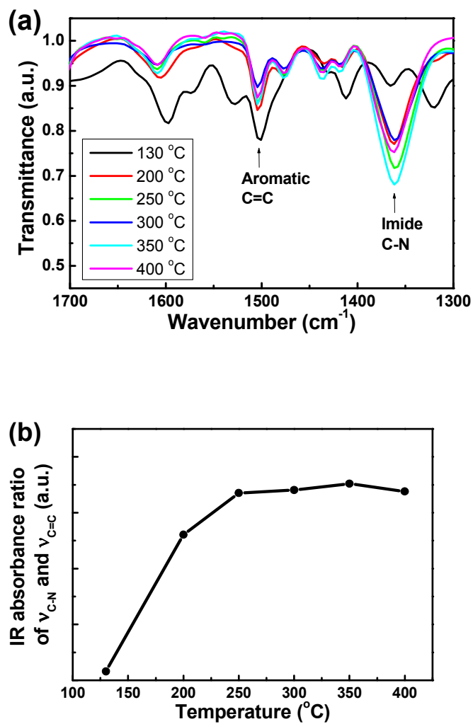
Fig. 2 Annealing temperature-dependent (a) IR spectrum and (b) \nu_{\text{C-N}} and \nu_{\text{C=C}} IR absorbance ratio of K-PIB films.
