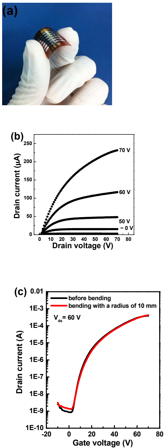
Fig. 8 (a) Photograph, (b) output characteristic ( I_{ds} vs. V_{ds} ) and (c) transfer characteristics ( I_{ds} vs. V_{gs} ) of the 350 °C-annealed flexible IZO TFT on a Kapton substrate.
