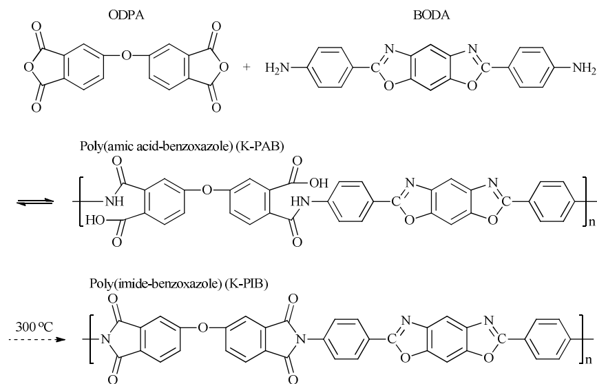
Scheme 1 Synthetic route to K-PIB gate insulator.
