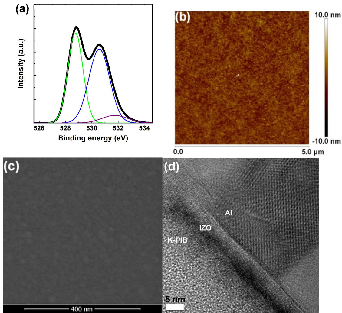
Fig. 5 (a) XPS spectrum, (b) AFM image ( 5\ \mu\text{m} \times 5\ \mu\text{m} ), (c) SEM image and (d) cross-sectioned TEM image of IZO layer on K-PIB film.
