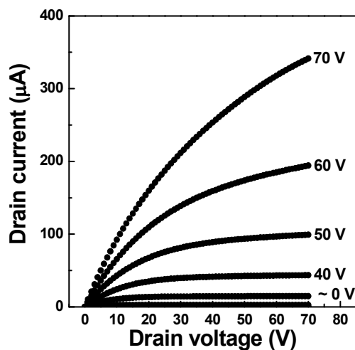
Fig. 7 Output characteristic ( I_{ds} vs. V_{ds} ) of the 350 °C-annealed IZO TFT.
