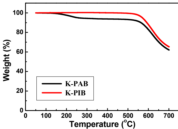
Fig. 1 TGA results of K-PAB and K-PIB.
