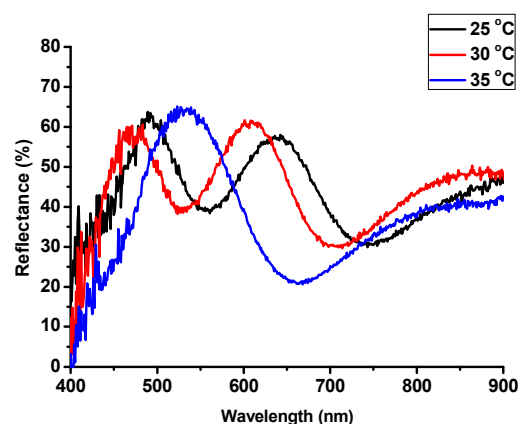
Figure 2. Reflectance spectra for a MG-1% etalon in water at the indicated temperatures.
