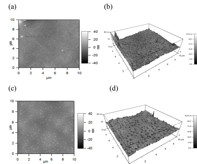
Figure 3. AFM images of microgel-1% etalon (a, b) before and (c, d) after UV stimulation. (a, c) 2-D and (b, d) 3-D images.
