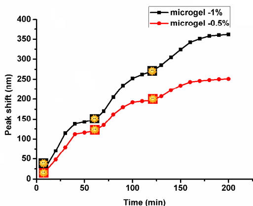
Figure 5. Peak shifts for the indicated microgel-based etalons as a function of time after sequential 2 min UV exposures (indicated by symbols).
