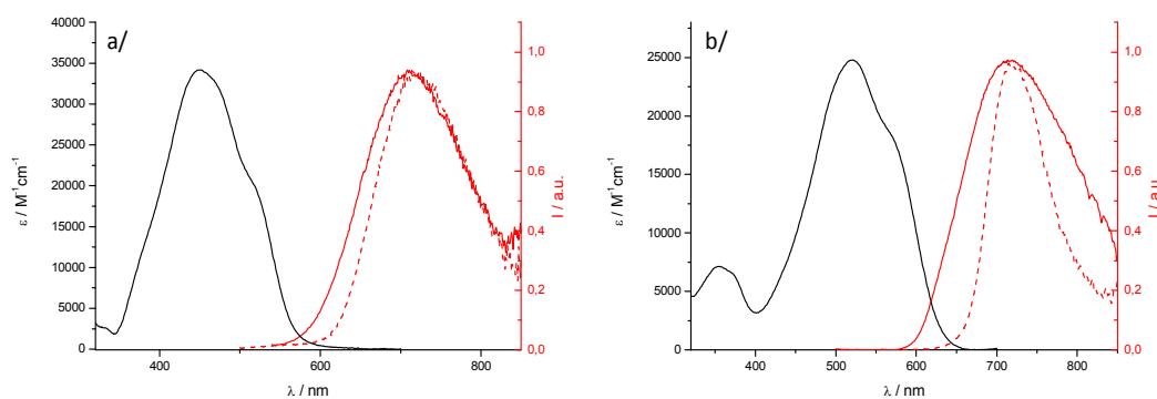
Figure 5. Electronic absorption of nanoparticles (—) and fluorescence emission spectra (—) of nanoparticles in water and powder samples (---) for a/ 1 and b/ 2 .
