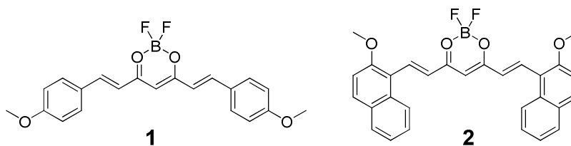
Chart 1. Chemical structure of the borondifluoride curcuminoids 1 and 2 .
