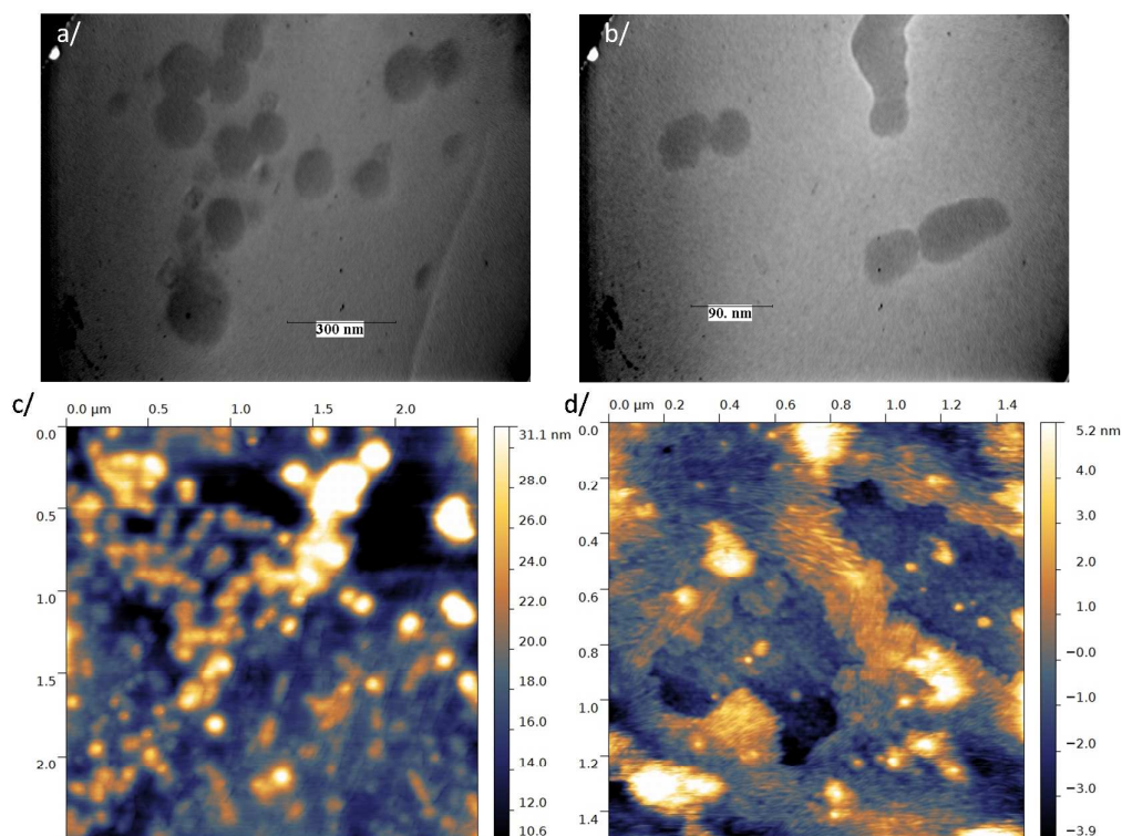
Figure 3. TEM images of the particles of a/ dye 1 and b/ dye 2 and tapping mode topographical AFM images of c/ dye 1 and d/ dye 2 .
