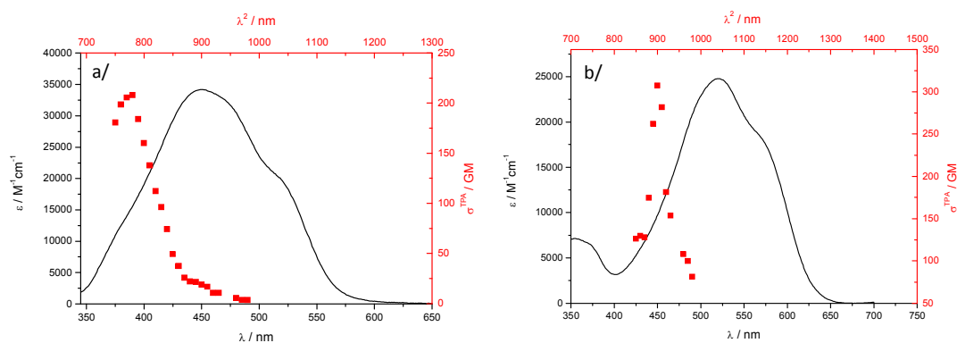
Figure 7. Two-photon excitation spectra (■, higher x-coordinate and —, right y-coordinate) and OPA absorption spectra (—, lower x-coordinate and —, left y-coordinate) of particles in water: a/ 1 and b/ 2 .
