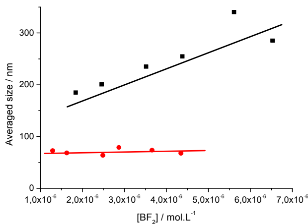
Figure 2. Variation of the averaged size determined by DLS for dye 1 (black) and dye 2 (red) as a function of the total dye concentration.
