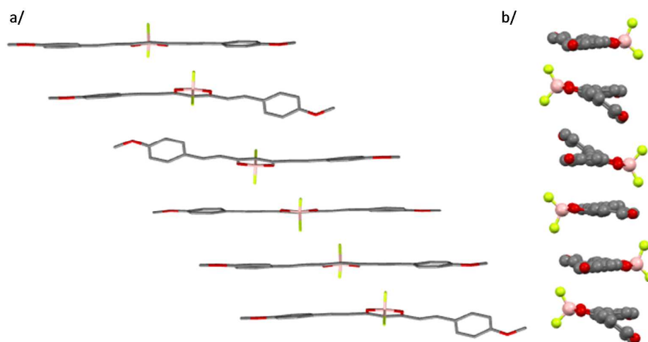
Figure 1. Crystal packing diagram of 1 down the c-axis direction (a), illustrating \pi - \pi stacking interactions, and the long molecular axis (b).
