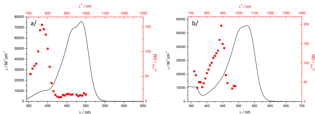
Figure 6. Two-photon excitation (■, higher x-coordinate and —, right y-coordinate), OPA spectra (—, lower x-coordinate and —, left y-coordinate) in DCM: a/ 1 and b/ 2 .
