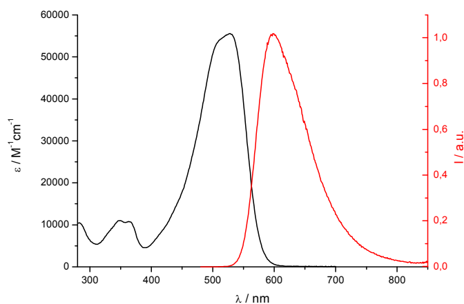
Figure 4. Electronic absorption (conc. \approx 10^{-5} \text{ M} , black) and corrected fluorescence emission (conc. \approx 10^{-6} \text{ M} , \lambda_{\text{exc}} at the absorption maximum, red) spectra of 2 in DCM.
