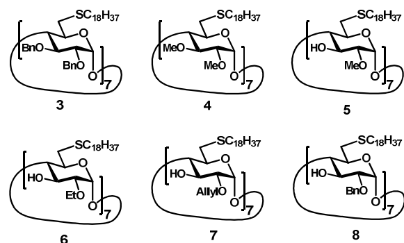
Figure 2. Thioalkylated CD targets 3-8 designed to study the structure-property relationship between hydrogen bonding and LC phase formation.
