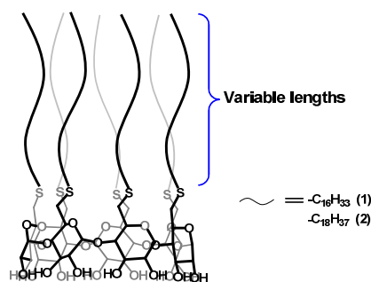
Figure 1. Schematic structures of previously synthesized \beta -CD derivatives exhibiting thermotropic LC properties
