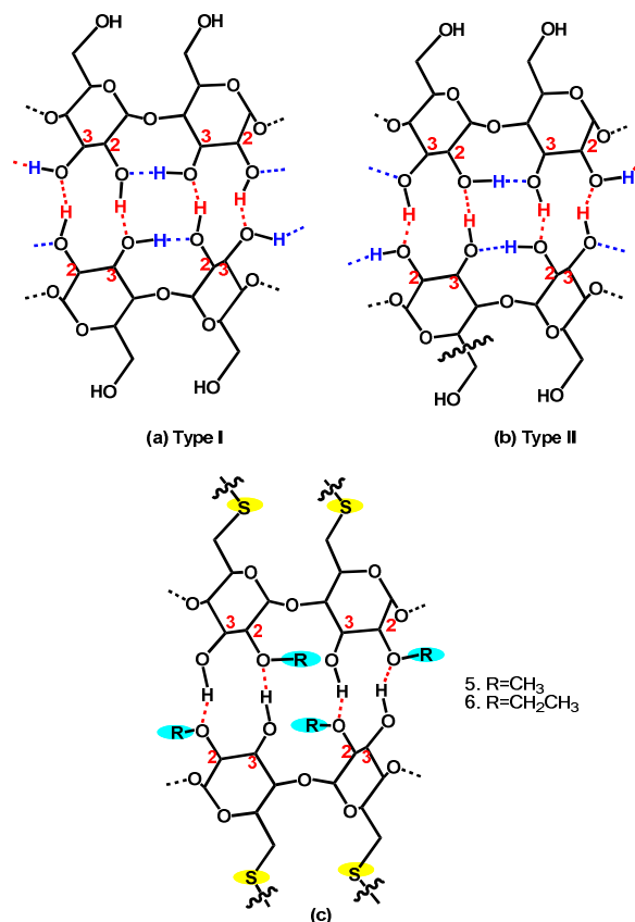
Figure 6. Possible hydrogen-bond networks established in natural CD dimers: (a) OH-2's as intermolecular hydrogen-bond donors while OH-3's act as intramolecular hydrogen bond acceptors, (b) OH-3's act as the intermolecular hydrogen-bond donors while OH-2's act as the intramolecular hydrogen-bond acceptors. (c) Proposed hydrogen-bond network established in dimer formed from compounds 5 and 6 .
