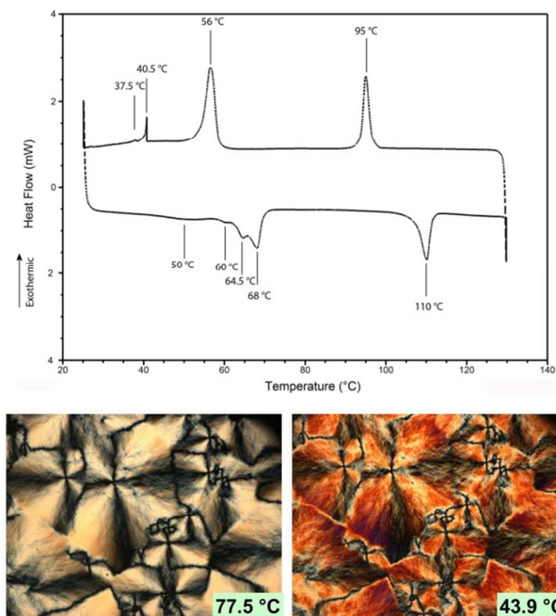
Figure 3. DSC thermogram of compound 5 (top) after heating compound 5 to clearing temperature and allowing it to cool to room temperature at 2 °C/minute and snapshots taken at 77.5 and 43.9 °C under POM.
