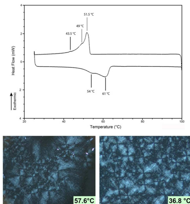
Figure 4. DSC thermogram of compound 6 (top) after heating compound 6 to clearing temperature and allowing it to cool to room temperature at 2 °C/minute and snapshots taken at 57.6 and 36.8 °C under POM.
