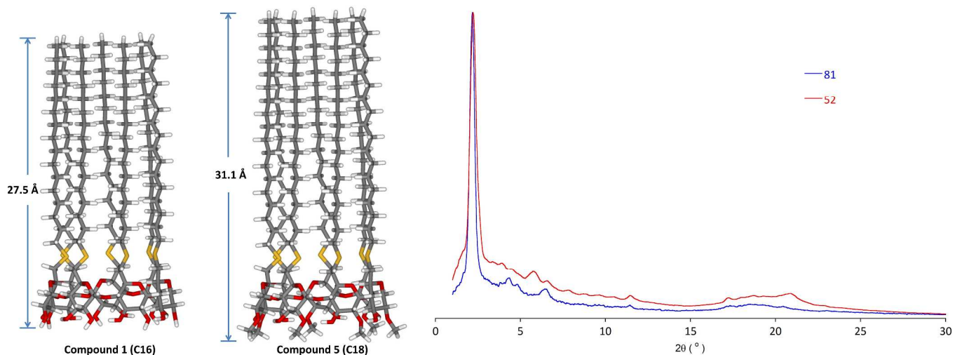
Figure 5. Left: molecular models show compounds 1 (C16) and 5 (C18) have respectively a dimension of 27.5 and 31.1 Å in the most extended conformation. Right: variable temperature XRD plots of compound 5 , recorded at 81, 52 °C.
