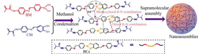
Scheme 1 Synthesis and supramolecular assembly of BCe.
