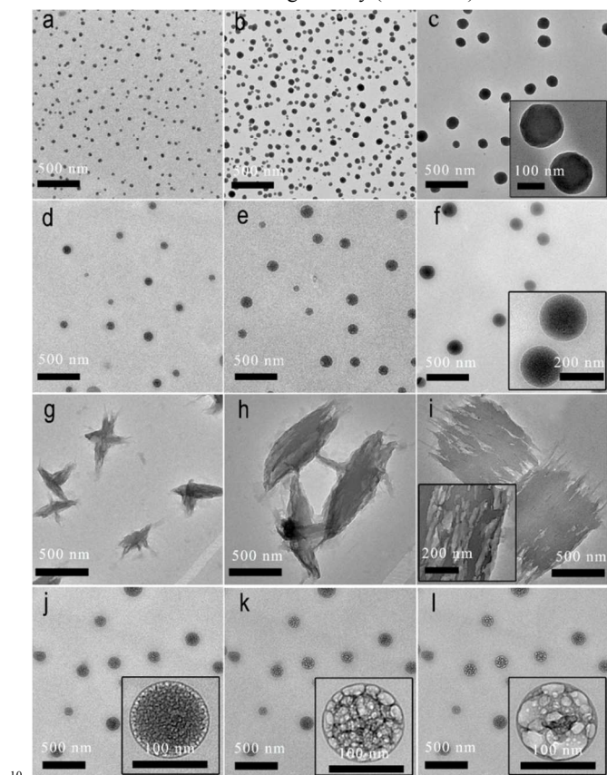
Fig. 1 TEM images of spherical nanoparticles prepared at -10\text{ }^{\circ}\text{C} with (a) 10.0, (b) 20.0 and (c) 40.0 mM of BM and CM. (d), (e) and (f) represent the typical TEM images of spherical supramolecular assemblies obtained at 0\text{ }^{\circ}\text{C} from 10.0, 20.0 and 40.0 mM of BM and CM, respectively. (g), (h) and (i) are the TEM images of layered structures formed by cooling the BCe methanol solution with 10.0, 20.0 and 40.0 mM concentrations from 25 to -10\text{ }^{\circ}\text{C} . (j), (k) and (l) show the morphologies of the spherical assemblies after electron beam irradiation for 30, 60, and 120 s, respectively; these nanospheres were prepared by using 20.0 mM of BM and CM at 0\text{ }^{\circ}\text{C} . The insets are the corresponding magnified TEM images.
