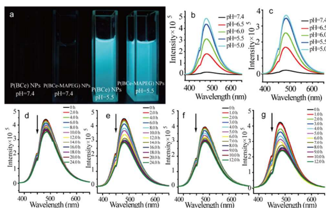
Fig. 5 (a) Photographs of P(BCe) and P(BCe-MAPEG) NPs in water with different pH values under UV irradiation (wavelength 360 nm). (b) and (c) are the effects of pH on the emission intensity of P(BCe) and P(BCe-MAPEG) NPs in water under an excitation wavelength of 360 nm. (d) and (e) are the emission evolutions of P(BCe-MAPEG) NPs in water solution with pH=5.5 and 5.0. (f) and (g) represent the emission evolutions of P(BCe-MAPEG) NPs in water solutions (pH=5.5) with 0.1 and 0.6 mM of D-glucose.
