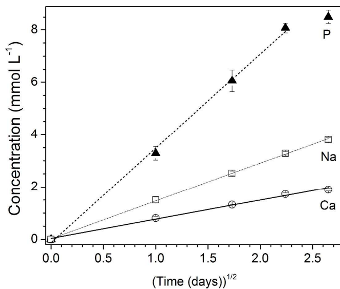
Figure 4: (a) Percentage of ions in solution at day 1 vs. P_2O_5 content in the glass. Line is linear regression; R^2 = 0.994 . (b) Ions released from glass CNP55 vs. the square root of time. Lines are linear regression; R^2 = 0.998 (P), 0.995 (Ca) and 0.999 (Na), respectively.
