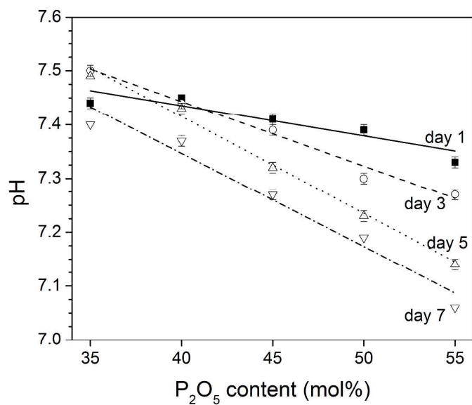
Figure 2: pH in Tris buffer solution: (a) pH vs. time and (b) pH vs. nominal P 2 O 5 content ( \pm SD). (Straight lines are linear regression; for coefficients of determination refer to the text.)
