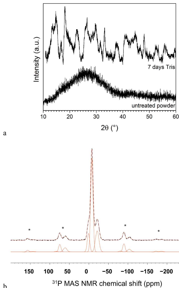
Figure 6: (a) XRD patterns of CNP50 glass powder before (bottom) and after (top) immersion in Tris buffer for 7 days, (b) ^{31}\text{P} MAS NMR spectrum (dashed black curve) together with the result of a deconvolution (red curve) into three Gaussian lines (lower red curves) at +1.1 ppm (12% of total signal), -7.6 ppm (64%) and -21.2 ppm (24%). For the calculation, spinning sidebands (marked by asterisks) were taken into account.
