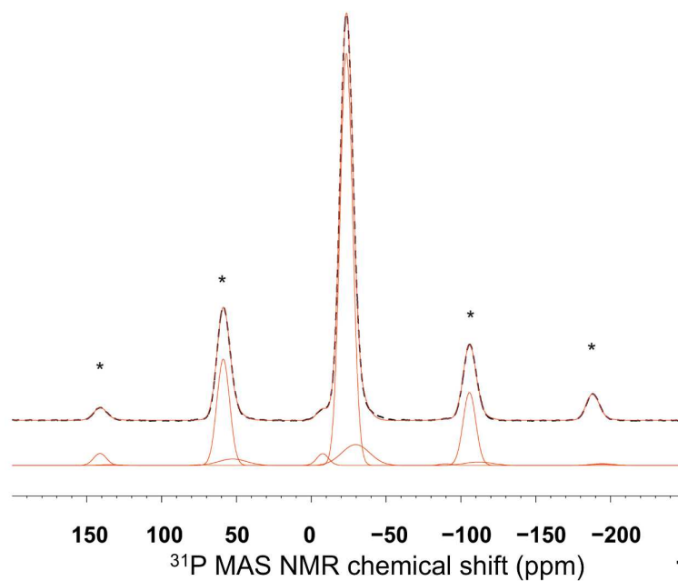
Figure 1: ^{31}\text{P} MAS NMR spectrum of glass CNP50 (dashed black curve) together with the result of a deconvolution (red curve) into three Gaussian lines (lower red curves) at -7.6 ppm (2% of total signal), -23.5 ppm (87%) and -29.7 ppm (11%). For the calculation, spinning sidebands (marked by asterisks) were taken into account.
