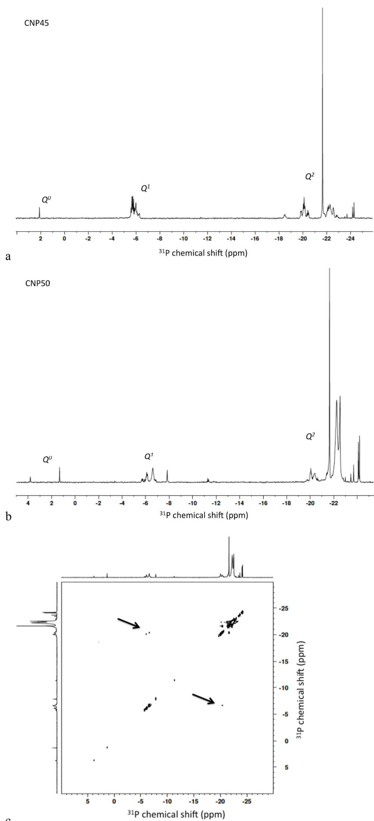
c Figure 5: ^{31}\text{P} NMR spectra of solutions of glasses (a) CNP45 and (b) CNP50 and (c) ^{31}\text{P} - ^{31}\text{P} TOCSY spectrum of solution of glass CNP50 at 24 h in Tris buffer (cross-peaks corresponding to coupling between ^{31}\text{P} nuclei in Q^1 and Q^2 groups highlighted by arrows).
