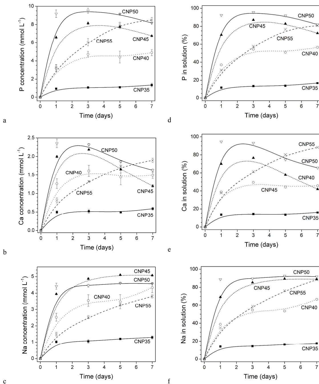
Figure 3: Ionic concentrations in Tris buffer solution: (a-c) concentrations in \text{mmol L}^{-1} ( \pm SD) and (d-f) percentage of ions in solution vs. time (for error bars refer to figures a-c). (Lines are visual guides only.)
