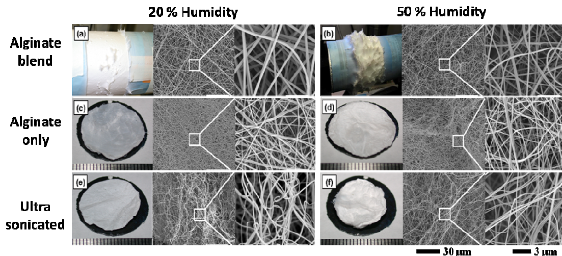
Figure 1. Photographs and SEM photomicrographs of the top surface of electrospun (a-b) alginate/PEO/Pluronic F127 blended nanofibers, (c-d) alginate only nanofibers following PEO-Pluronic F127 extraction, and (e-f) ultra-sonicated alginate-only nanofibers fabricated at 20% and 50% humidity conditions.
