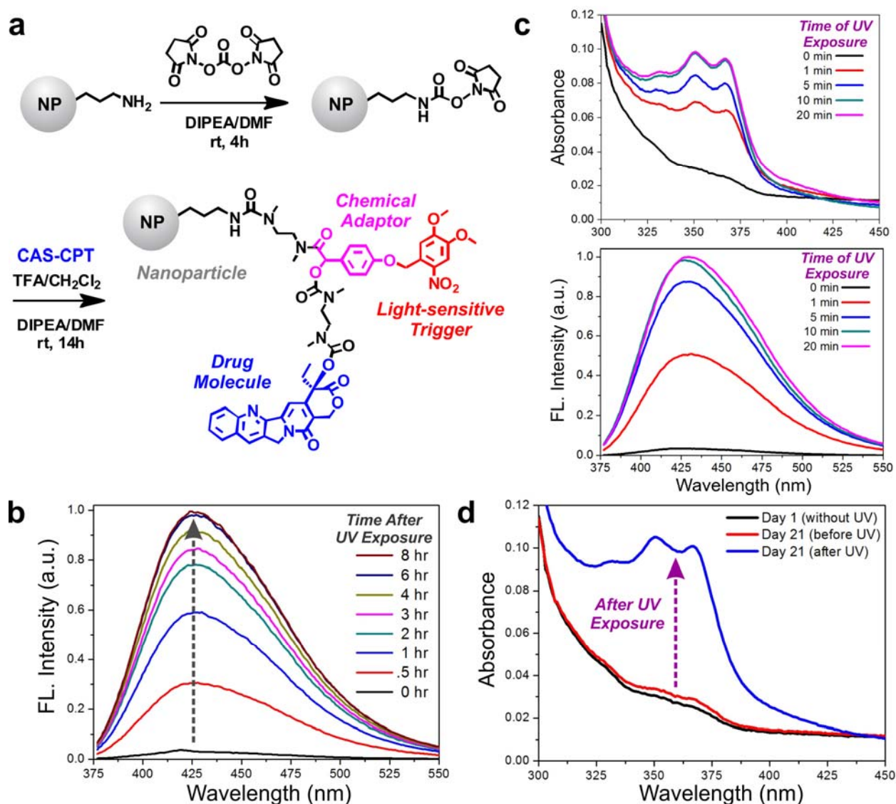
Fig. 3. The CAS-CPT conjugated nanoparticle constructs show excellent stability and photo-triggered release. (a) Scheme for conjugation of CAS-CPT on silica NPs. (b) Release of CPT monitored over time after 10 mins of UV light exposure (365 nm, 2.5 mW/cm 2 ) using fluorescence spectroscopy. (c) Release of CPT measured after varying times of UV light exposure (0 – 20 mins). Measurements were acquired 24 hrs after UV exposure, using absorption spectroscopy ( top ) and fluorescence spectroscopy ( bottom , \lambda_{\text{ex}} = 368 nm). (d) Absorbance spectra measured over 21 days in the absence of UV exposure ( black & red ), followed by 10-min UV irradiation after 21 days ( blue ).
