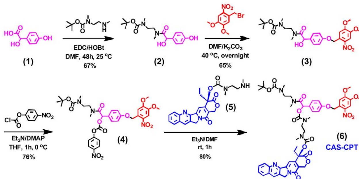
Fig. 2. Synthesis of the chemical adaptor system (CAS) bound with camptothecin (CPT). The core of the CAS (4-hydroxymandelic acid) was covalently attached with the phototrigger group (4,5-dimethoxy-2-nitrobenzyl) and the anticancer drug (CPT).
