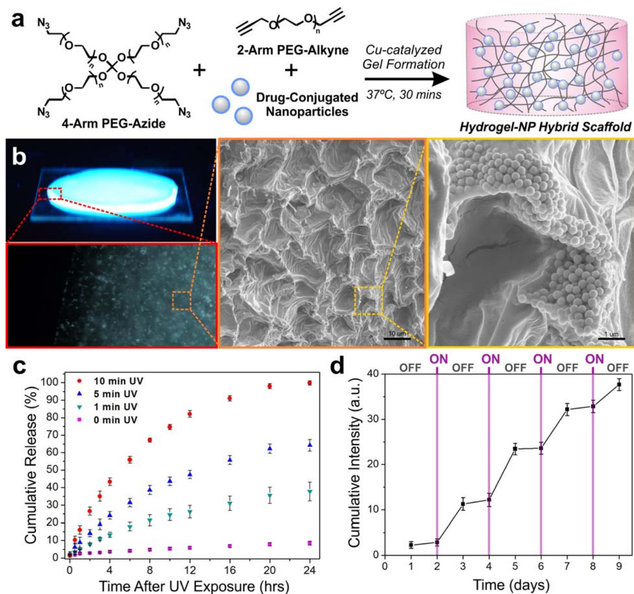
Fig. 4. Hydrogel-NP hybrid scaffolds enable the controlled and on-demand release of drugs. (a) Scheme for encapsulation of drug-conjugated NPs within PEG-based hydrogels formed using copper-catalyzed Click chemistry. (b) Fluorescence and SEM images of NPs distributed throughout the hydrogel matrix. (c) The cumulative release of CPT from hydrogel-NP hybrid scaffolds ( n = 3 ) after varying times of UV light exposure (365 nm, 2.5 mW/cm 2 ), measured over 24 hrs after photo-irradiation. (d) Cumulative CPT release from the hydrogel-NP hybrid scaffolds ( n = 3 ) with cycles of OFF (48 hr) and ON (30-seconds UV light).
