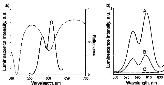
Figure 6. a) Luminescence spectra of Eu(III) complex labeled streptavidin captured on a biotin-functionalized MC57/23 (solid line) overlaid with the corresponding reflectance spectrum (dashed line) of the microcavity and b) luminescence spectra of Eu(III) complex labeled streptavidin on A) MC57/23 in MES buffer, B) a single pSi layer in MES buffer, and C) biotin-functionalized surface without labeled streptavidin.
