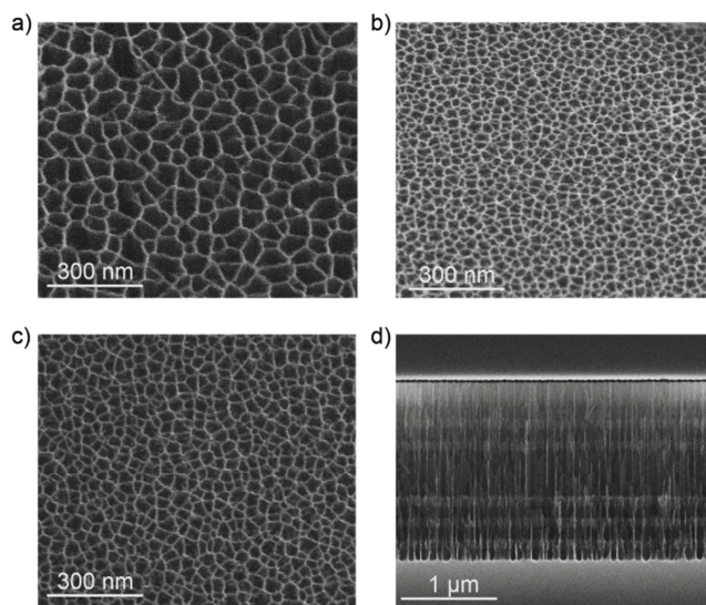
Figure 3. SEM images of a) top-view H surface, b) top-view L surface of sample MC57/14, c) top-view L surface of sample MC57/23 and d) cross-sectional view of the MC57/23.
