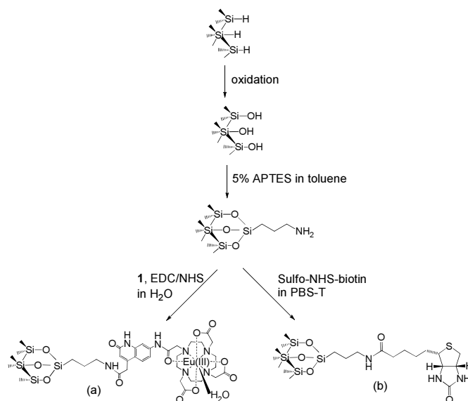
Scheme 1. Surface modifications of the pSi resulting in a) a surface with covalently attached complex 1 and b) a surface functionalized with biotin for streptavidin detection.
