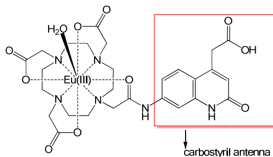
Figure 1. 1,4,7-Tris(carboxymethyl)-10-(4'-quinolineacetic acid, (7'-acetamide)-1',2'-dihydro-2'-oxo)-1,4,7,10-tetraazacyclododecane.Eu, 1.
