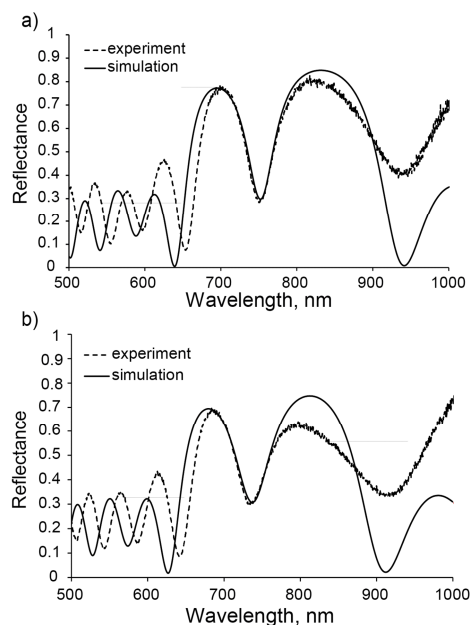
Figure 2. Best-fit of the simulated and experimentally obtained reflectance spectra of freshly etched a) MC57/14 and b) MC57/23. The experimental spectra were recorded at normal incidence.
