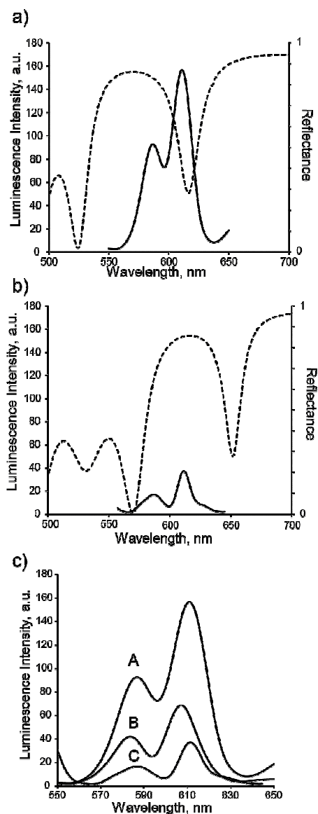
Figure 5. Luminescence measurement of Eu(III) complex 1 on pSi surfaces a) pSiMC with aligned resonance wavelength, b) pSiMC with non-aligned resonance wavelength and c) luminescence of Eu(III) complex 1 on a aligned microcavity (A), a single layer (B) and a non-aligned pSiMC (C). The dashed line show the simulated reflectance spectra of MC57/14 modified with complex 1 at 45° incidence.
