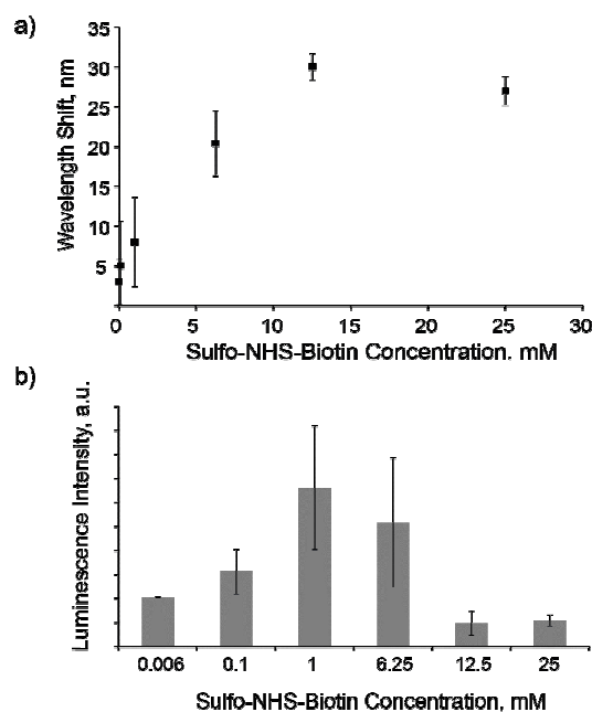
Figure 7. a) Shifts in resonance wavelength of the amine-functionalized MC57/23 microcavity after reaction with sulfo-NHS-biotin at various concentrations and b) measured luminescence intensity of the biotin-functionalized microcavities (using different sulfo-NHS-biotin concentrations during functionalization) at 614 nm upon incubation with labeled streptavidin (5 \mu M).
