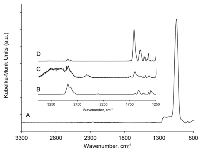
Figure 4. DRIFT spectra of modified pSi after a) oxidation, b) APTES modification, c) modified with complex 1 and d) modified with NHS-biotin.
