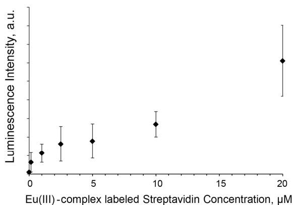
Figure 8. Luminescence intensity of Eu(III) complex labeled streptavidin captured on MC57/23 as a function of its concentration. n = 5 .
