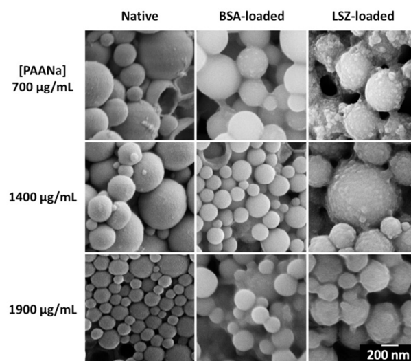
Figure 3. SEM micrographs of native, BSA and LSZ-loaded microcarriers as a function of PAANA concentration (700, 1400 and 1900 µg mL -1 ). [Ca^{2+}]=[CO_3^{2-}] was kept constant at 12 mM. Complexation time was set to 1 minute.
