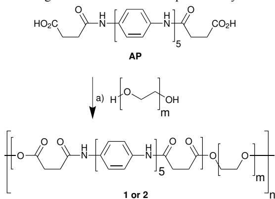
Scheme 1 Synthesis of electroactive polyesters 1 and 2 via the Steglich esterification. a) DCC, DMAP, NMP, 72 h, r.t.
