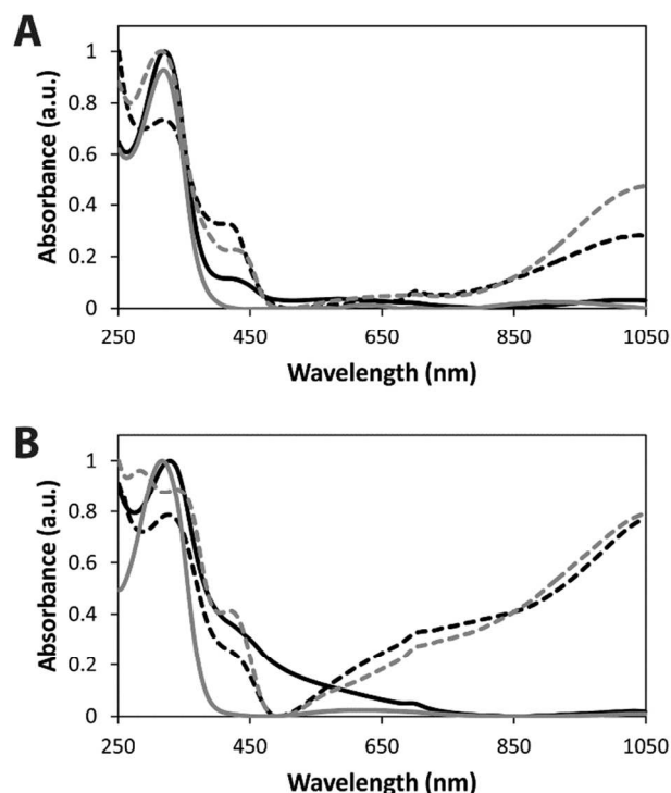
Fig. 2 UV-visible spectra of thin polyester films on quartz slides. A) Polyester 1 undoped, black line; polyester 1 doped with CSA, dashed black line; polyester 2 undoped, grey line; polyester 2 doped with CSA, dashed grey line; B) polyester 3 undoped, black line; polyester 3 doped with CSA, dashed black line; polyester 4 undoped, grey line; polyester 4 doped with CSA, dashed grey line.
