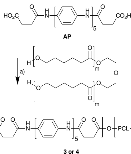
Scheme 2 Synthesis of electroactive polyesters 3 and 4 via the Steglich esterification. a) DCC, DMAP, NMP, 72 h, r.t.
