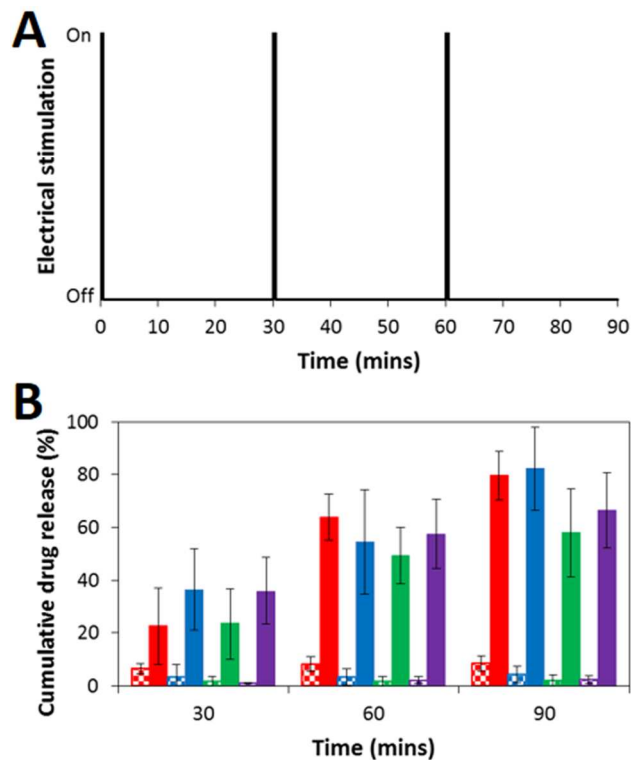
Fig. 4 Electrochemically-triggered drug delivery via a potential step. A) Electrical stimulation paradigm: 3 cycles of 0.5 minutes on, 29.5 minutes off. B) Release of DMP from films of 1-4 in PBS as determined by UV spectroscopy. DMP release with electrical stimulation (solid bars) or without electrical stimulation (checked bars). Polyester 1 , red. Polyester 2 , blue. Polyester 3 , green. Polyester 4 , purple.
