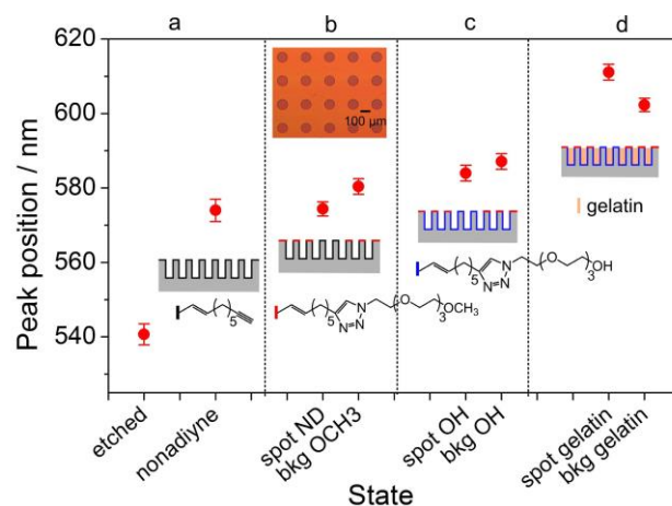
Fig. 3 Optical reflectivity from 100 data points after each step of modification on both spot and background regions of the patterned surface. The x-axis presents the state of the surface: 'etched'-freshly etched PSi; 'nonadiyne'-PSi after modification with nonadiyne (ND); 'spot ND'-spot regions with nonadiyne modified surface; 'bkg OCH 3 '-background regions with azido-EO 3 -OCH 3 modified surface; 'spot OH'-spot regions with azido-EO 3 -OH modified surface; 'bkg OH'-background regions with azido-EO 3 -OH modified surface; 'spot gelatin'-spot regions with gelatin modified surface; 'bkg gelatin'-background regions with gelatin modified surface; (a) The attachment of alkyne terminated monolayer resulted in 33 nm red shift of the peak position. (b) The attachment of azido-EO 3 -OCH 3 in the background regions in the first click reaction resulted in 6.4 nm red shift in the background regions, while the spot regions have no shift; insert on the top shows an optical microscopy image of the chemically patterned PSi surface after the first click reaction. (c) The attachment of azido-EO 3 -OH on the surface of spot regions and throughout the internal pore walls of the entire structure. There are 10 nm and 6.7 nm red shifts in the spot and background regions respectively. (d) The filling of gelatin into the pore structure leads to 27.1 nm and 15.2 nm red shifts on in the same spot and background regions.
