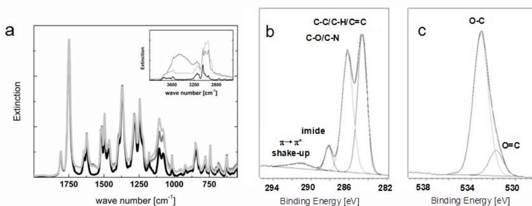
Figure 2. a) Comparison of FT-ATR-IR spectra of untreated PEI-O (black), hPG-OH functionalized (gray), and hPG-OMe (light gray). Representative XPS spectra of the C1s (b) and O1s (c) region scan in the XPS for the PEI membrane functionalized with hOG-OH, indicating a decrease of carbon content and an increase in oxygen content compared to unfunctionalized PEI.
