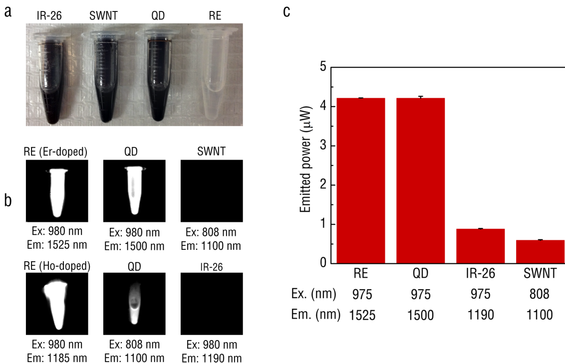
Fig. 7. A comparison of the performance of various IR-emitting fluorescent probes including IR-26 organic dye, PbS quantum dots, single walled carbon nanotubes and Ho- and Er-doped phosphors: (a) visual image without any excitation and (b) images of IR emissions captured by an InGaAs camera at optimal excitation wavelengths. (c) An integrating sphere was used to quantify the power output of the probes. 28 All materials were first dissolved in toluene at 20 mg ml -1 and excited by either 975 nm or 808 nm light at the exact same power (30 \mu W). Reprinted (adapted) with permission from Nature Communications. Copyright 2013 © Nature Publishing Group.
