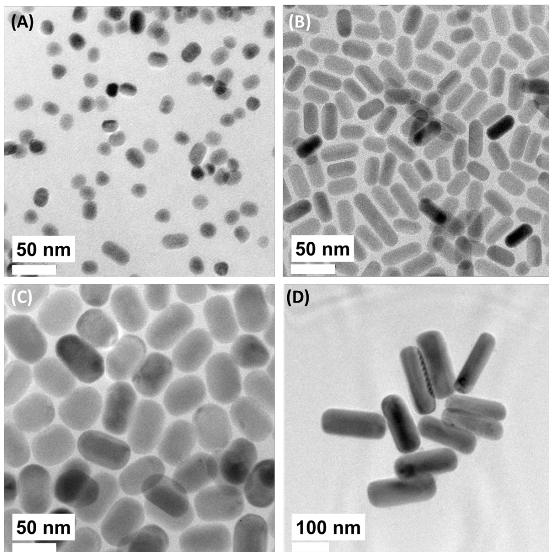
Fig. 3. Solvothermal synthesis of \beta - \text{NaYF}_4 :Yb,Er with different sizes and morphologies. (A) 14 nm \times 11 nm, (B) 23 nm \times 16 nm, (C) 53 nm \times 31 nm, and (D) 179 nm \times 63 nm. 42 Reprinted (adapted) with permission from The Journal of Physical Chemistry C. Copyright 2013 \copyright American Chemical Society.
