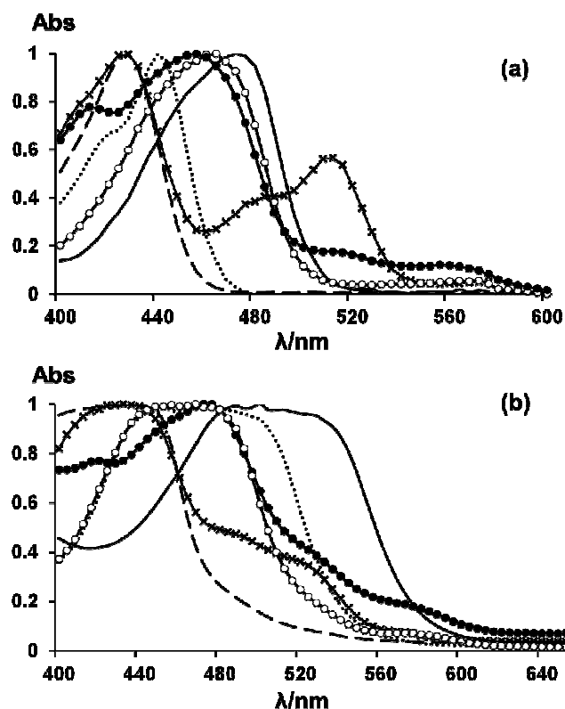
Fig. 4 UV-Vis spectra of selected dyes (a) in solution (1 \mu\text{M} ) and (b) adsorbed to \text{TiO}_2 films; (4) solid line, (5) dotted line, (7) long dashes, (8) open circles, (10) crosses, (11) filled circles.
