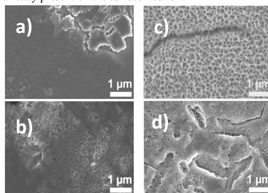
Fig. 1 SEM images of native titanium foil (a), passivated in HNO 3 (b), native foil etched in H 2 O 2 for 1 h at 95°C (c), or native foil etched in H 2 O 2 for 48 h at room temperature (d).
