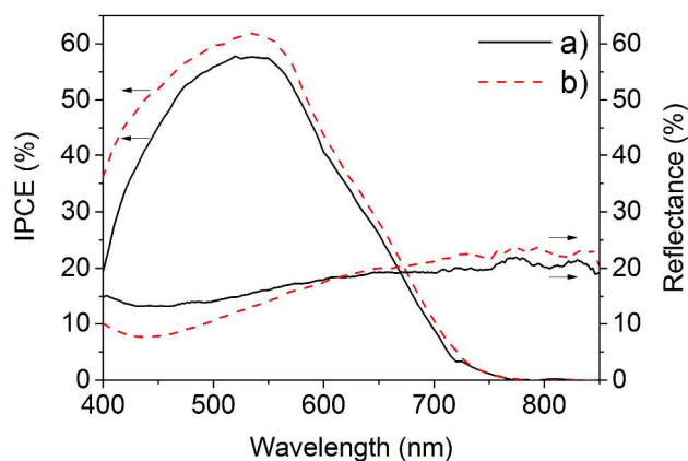
Fig. 5 Incident photon to current efficiency (IPCE) of DSSCs and reflectance of working electrode substrates of native (a), and in HNO 3 passivated (b), titanium foil of these foils.
