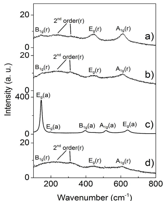
Fig. 3 Raman spectra of titanium foil after thermal annealing, native (a), passivated in \text{HNO}_3 (b), etched 1 h in \text{H}_2\text{O}_2 at 95^\circ\text{C} (c), or etched 48 h in \text{H}_2\text{O}_2 at room temperature (d). (c) and (d) were both performed after passivation in \text{HNO}_3 . The vibrational modes of either rutile (r) or anatase (a) were assigned according to references. 13-15
