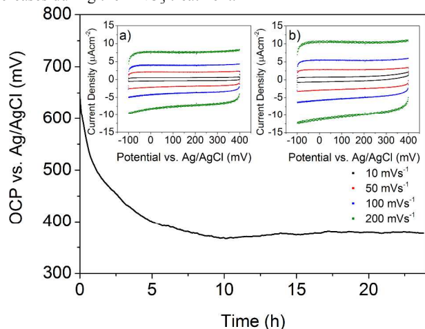
Fig. 2 Open circuit potential – time transient of titanium foil in HNO 3 measured for 24 h. Inserts: Cyclic voltammograms in 1 M Na 2 SO 4 solution at scan rates ranging from 10 to 200 mVs -1 of native Ti foil (a), and in HNO 3 passivated Ti foil (b).
