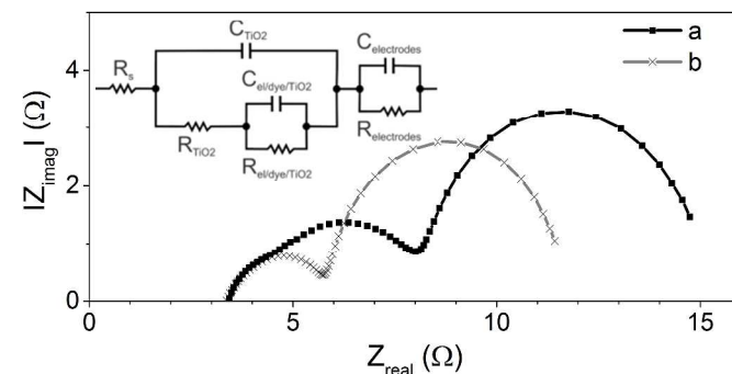
Fig. 4 Nyquist plots of DSSCs with titanium foil as working electrode substrate which was native (a) and passivated in \text{HNO}_3 (b). EIS data were obtained at V_{\text{OC}} and 100 \text{ mW cm}^{-2} simulated AM 1.5 sunlight illumination in a frequency range from 0.3 MHz to 2 Hz. The equivalent circuit diagram used for fitting the data is displayed in the inset.
