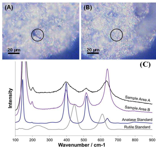
Fig. 5 Raman spectra (c) of two areas (sample area A Fig 5a, sample area B Fig 5b) of a titania coating produced in an Ar/H 2 plasma from a 12 nm feedstock, with reference spectra. 41,42 The circles on images A and B correspond to the analysed areas.
