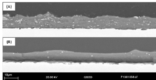
Fig. 10 The cross sections of SPS titania coatings produced in an Ar/H 2 plasma (a) and Ar plasma (b), respectively. Some damage was visible at the substrate coating interfaces. This damage can be said to have occurred during sectioning or metallographic grinding/polishing as there is no mounting epoxy in the void. Had the damage occurred during spraying, this void would be filled due to the use of vacuum impregnation during epoxy encapsulation before sample sectioning and mounting.
