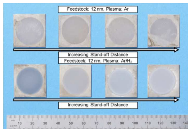
Fig. 3 Photograph showing 12 nm titania feedstock coatings produced by SPS in Ar and Ar/H 2 plasma conditions at the range of stand-off distances. Coatings are produced as circles due to their mounting in the water cooled jig.
