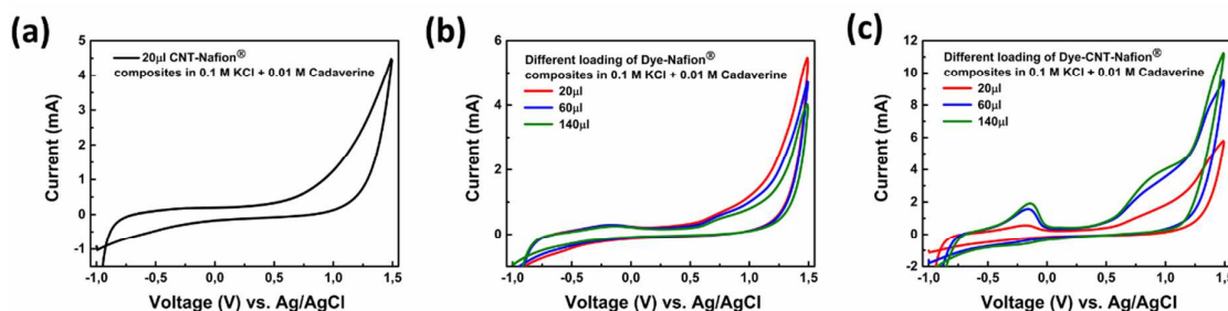
Figure 7 Cyclic voltammetry curves of (a) Nafion ® -CNT, (b) dye- -Nafion ® and (c) dye-Nafion-CNT composites in 0.1 M KCl electrolyte with the presence of 0.01 M cadaverine. The plots with different color compare the performance of composites with different amounts deposited on the glassy carbon electrode. The cycling speed used was 50 mV/s and all the voltammograms shown are from the first cycle.
