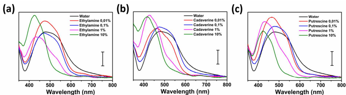
Figure 3 Absorption spectra of dye sensor upon immersion into (a) ethylamine, (b) cadaverine and (c) putrescine solution. Note: Due to the drift of calibration in the long measurement periods, the plotted curves were manually shifted vertically to set the intensity values equal at 800 nm. The vertical bars show 5% optical absorption.
