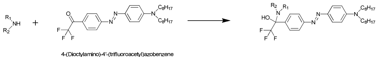
Scheme 1 Bonding reaction of 4-(Diocetylamino)-4'-(trifluoroacetyl)azobenzene and amine
