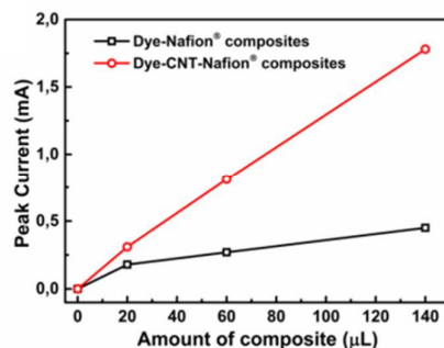
Figure 8 Comparison of peak current corresponding to the electrooxidation of cadaverine ( E_p \sim 0.8 V (vs. Ag/AgCl)) shown in Figures 7 (b) and (c) after the background subtraction.
