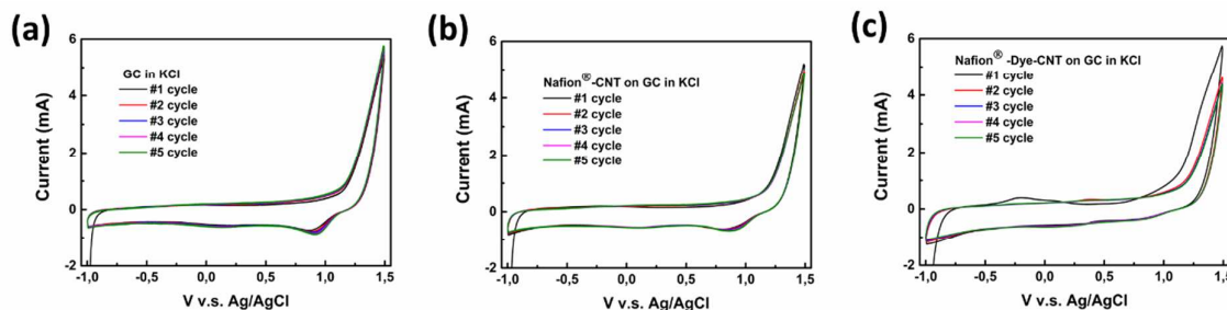
Figure 6 Cyclic voltammograms of (a) Glassy carbon (GC) electrode, (b) Nafion+CNT modified electrode and (c) Dye+Nafion+CNT modified electrode in 0.1 M KCl. Scan rate used was 50 mV/s for each measurement and the voltammogram shown is from the first cycle if not otherwise indicated.
