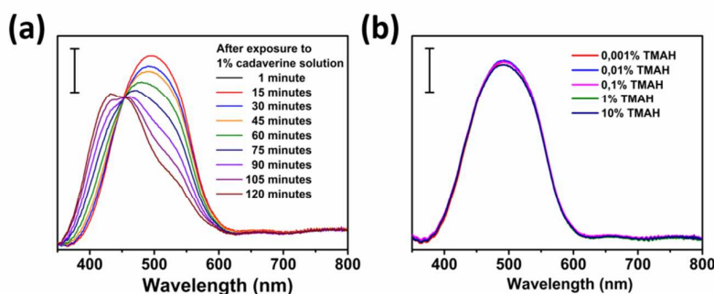
Figure 1 Absorption spectra of spin-coated thin film dye sensors (a) in the course of 2-hour exposure to the vapor of 1% cadaverine solution and (b) after two hours of exposure to the vapors of TMAH solutions having different concentrations. Note: Due to the drift of calibration in the long measurement periods, the plotted curves were manually shifted vertically to set the intensity values equal at 800 nm. The vertical bars show 5% optical absorption.
