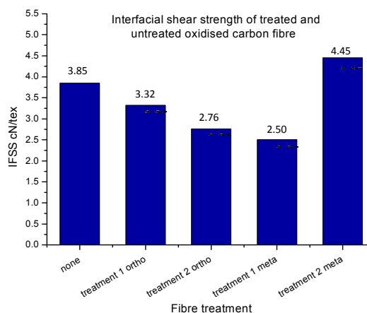
Figure 12 Interfacial shear strength of treated and untreated samples. From left to right: Control (oxidised and unsized fibre); Fibres functionalised with 14 treatment 1 only, Fibres functionalised with 14 treatment 2, Fibres
