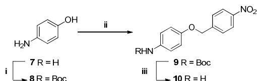
Scheme 1 Conditions (i) \text{Boc}_2\text{O} , \text{NaHCO}_3 , \text{NaCl} , \text{CH}_2\text{Cl}_2/\text{H}_2\text{O} , 50 °C, 2 h; (ii) 4-nitrobenzyl bromide, \text{KOH} , \text{NaI} , acetone, 55 °C, 16 h; (iii) \text{TFA} , \text{CH}_2\text{Cl}_2 , 12 h.
