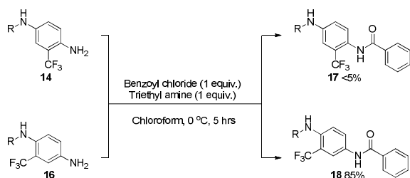
Scheme 6 Relative amine nucleophilicity of 14 vs 16 .
