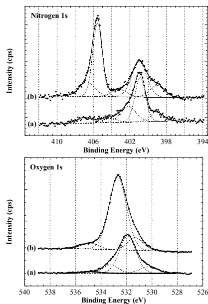
Figure 2 XPS N1s and O1s spectra, (a) untreated fibre and (b) analogue (A)
