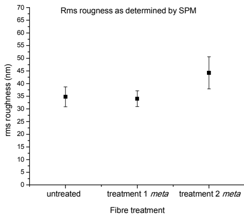
Figure 10 Calculated rms roughness for 1x1 \mu\text{m} images of control carbon fibres and fibres functionalised with 16 after treatments 1 and 2 (statistically significant data denoted *).
