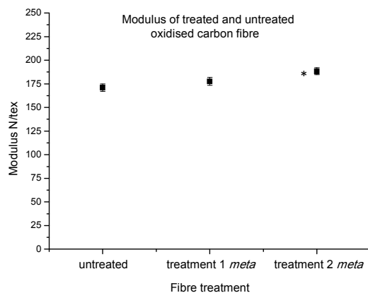
Figure 7 Average modulus control carbon fibres and fibres functionalised with 16 after treatments 1 and 2 (statistically significant data denoted *).
