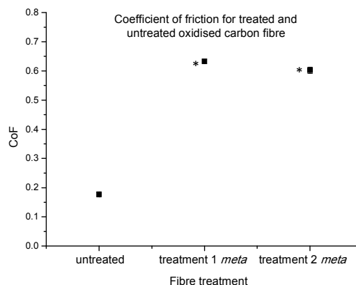
Figure 8 Average coefficient of friction control carbon fibres and fibres functionalised with 16 after treatments 1 and 2 (statistically significant data denoted *).
