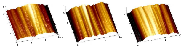
Figure 9 Representative height images for (a) untreated (oxidised and unsized) and treated samples ( 16 ), (b) treatment 1, (c) treatment 2
