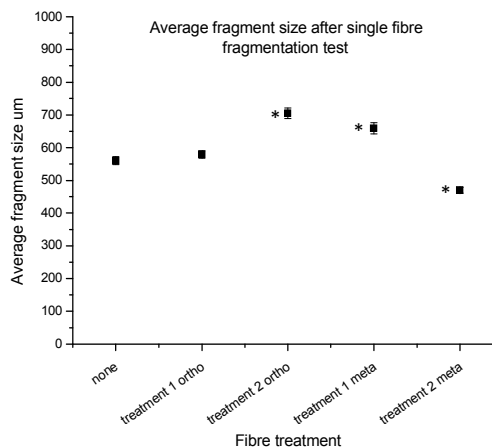
Figure 11 Average fragment size from SFFT, from left to right: Control (oxidised and unsized fibre); Fibres functionalised with 14 treatment 1 only, Fibres functionalised with 14 treatment 2, Fibres functionalised with 16 treatment 1 only, and Fibres functionalised with 16 treatment 2. Statistically significant results denoted by *
