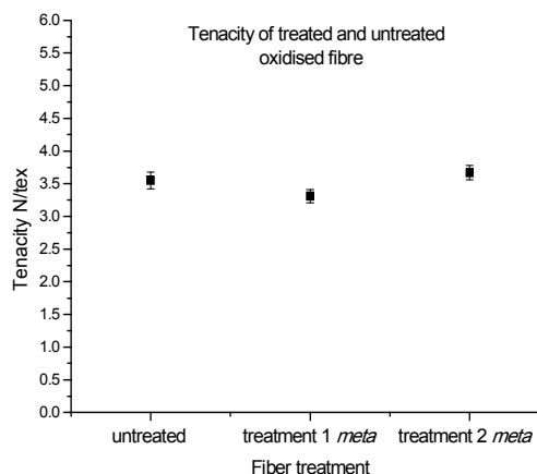
Figure 6 Tenacity of single fibres having undergone functionalisation with 16 .
