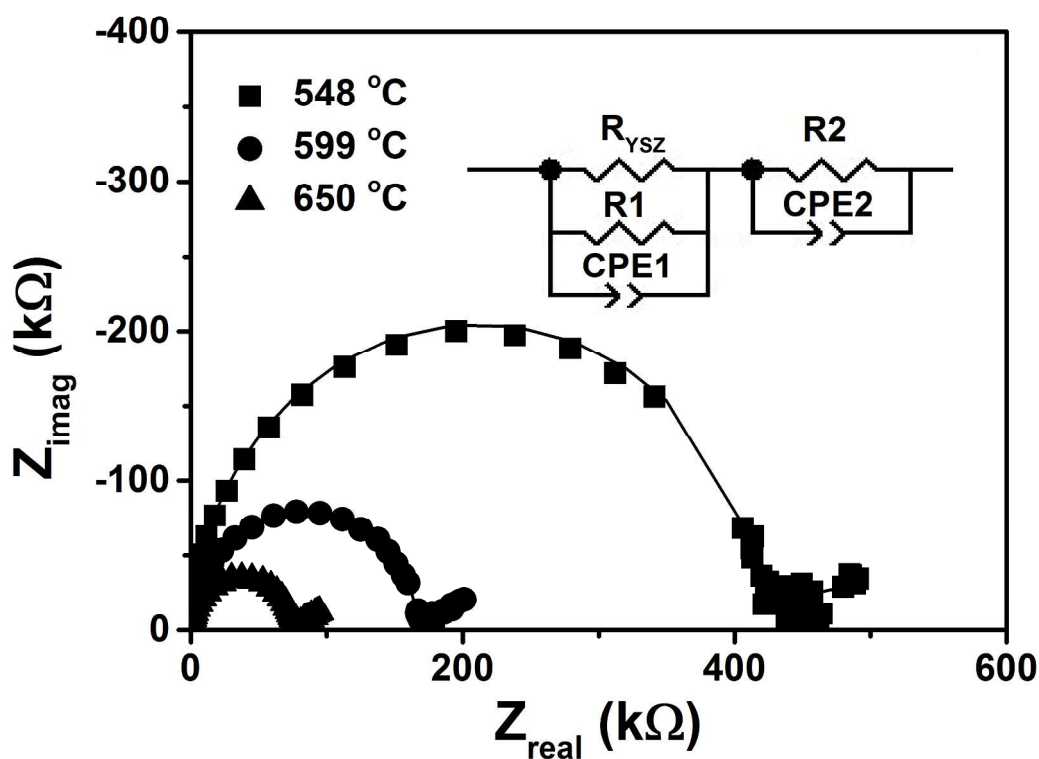
Figure 4. Impedance spectra measured in open air of YSZ/CZO45 multilayers with N=10 at the temperatures indicated. Also shown is the equivalent circuit used to fit the data ( R_{\text{YSZ}} was a fixed value at each temperature).
