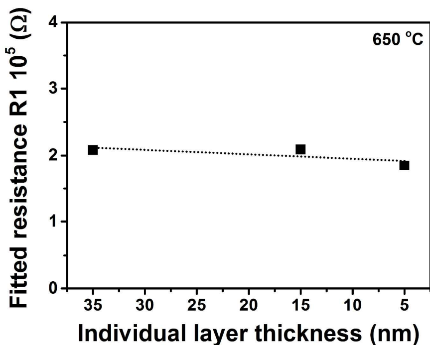
Figure 5. The fitted resistance R1 of YSZ/CZO30 multilayers as a function of the individual layer thickness at 650 °C.
