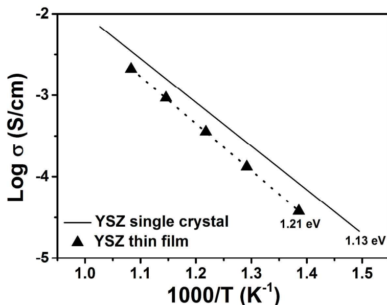
Figure 6. Comparison of electrical conductivity between a 105 nm-thick YSZ single-layer film and a roughly 500 \mu\text{m} -thick single crystal YSZ bulk sample.
