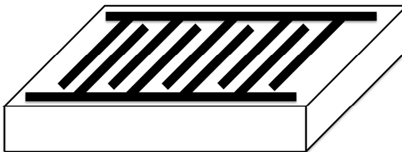
Figure 1. Platinum interdigitated electrode pattern deposited on the top surface of film for impedance measurement. The width and inter-space of the electrode fingers were both kept at 100 \mu\text{m} . The total perimeter length of the electrodes was \approx 115 mm.
