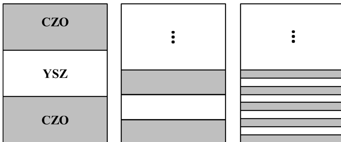
Figure 2. Schematic structure of the multilayer films composed of alternating layers of YSZ and CZO above the 5 nm-thick YSZ buffer layer.
