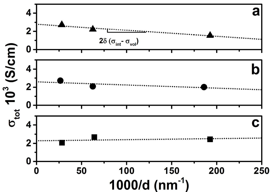
Figure 8. Conductivity isotherms at 650 °C of (a) YSZ/CeO 2 , (b) YSZ/CZO30, and (c) YSZ/CZO45 multilayers as a function of the reciprocal thickness of the YSZ layers, 1/d .
