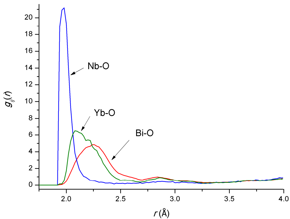
Fig. 7. M-O pair correlation functions g_{\text{M-O}}(r) for \text{Bi}_3\text{Nb}_{0.4}\text{Yb}_{0.6}\text{O}_{6.4} at room temperature, showing Bi-O (red) Nb-O (blue) and Yb-O (green) correlations.
