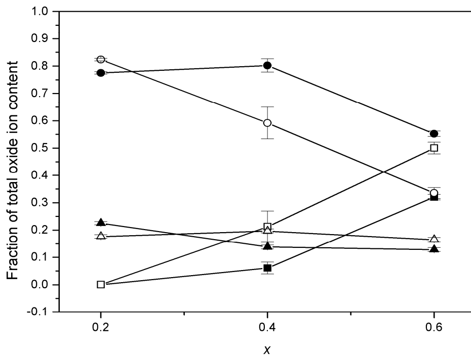
Fig. 5. Variation of oxide ion site occupancies in \text{Bi}_3\text{Nb}_{1-x}\text{Yb}_x\text{O}_{7-x} . Values presented as fraction of total oxide ion content. Filled and open symbols represent ambient and 800°C values respectively, with squares, circles and triangles representing 8c, 32f and 48i sites respectively. Error bars are indicated.
