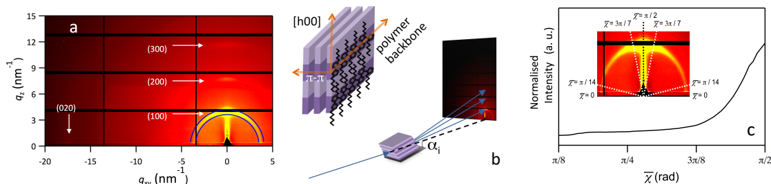
Fig. 3 GIWAXS spectra of a P3HT film on PEDOT:PSS. (a) The corrected 2-D spectrum with diffraction peaks labeled. The integration region is demarcated with solid blue lines (—). (b) Schematic of the chain packing for a single edge-on P3HT crystal in the GIWAXS geometry (c) Azimuthal integration of the (100) diffraction ring in (a). The inset details the polar coordinate system used.
