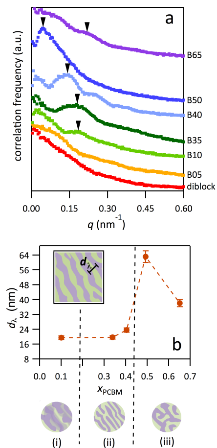
Fig. 6 Block copolymer length scales measured by AFM for P3HT- b -P3EHT:PCBM thin films. (a) Radial integrations of the phase image DFT's, arrows denote the peak used to calculate d_\lambda (b) The repeat domain spacing, d_\lambda (●). The schematics below the graph correspond to the distinct surface nano-morphologies observed: (i) disordered, (ii) fine, ordered lamellae, and (iii) large, disordered structures.
