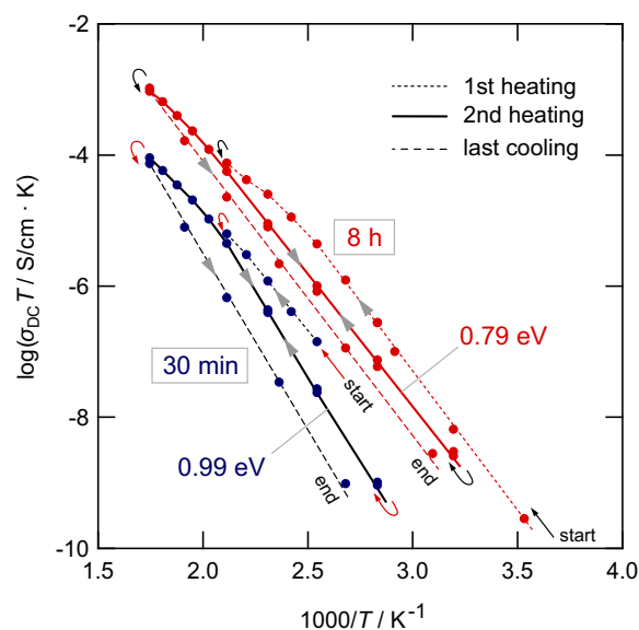
Fig. 11: Heating and cooling runs of the \text{LiAlO}_2 samples treated for 30 min and 8 h in a planetary mill. Data points have been recorded after the samples were dried at 373 K inside the impedance cell to remove any traces of moisture near the surface regions. The deviations from linear Arrhenius behavior at elevated T reflects healing of defects and points to re-organization of local structures. The 2 nd heating runs (see bold lines) are used for the comparison shown in Fig. 10.
