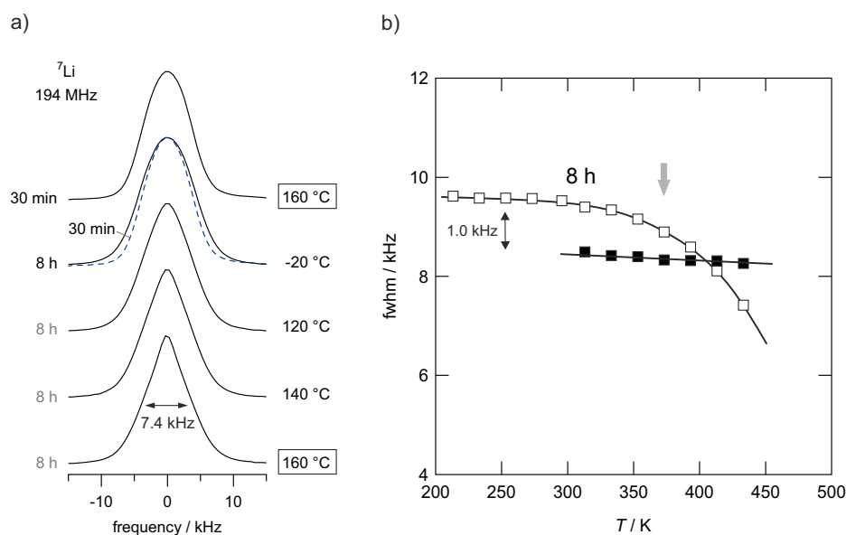
Fig. 12: a) Temperature-variable {}^7\text{Li} NMR spectra of \text{LiAlO}_2 milled for 8 h and 30 min, respectively. Spectra have been recorded under static conditions. The sample milled for 8 h shows significant motional narrowing at temperatures above 350 K. Starting from about 9.6 kHz the line width decreases to 7.4 kHz at 433 K. At this temperature, \text{LiAlO}_2 treated for only 30 min does not reveal any significant line narrowing (see also the spectrum shown by a dashed line). Thus, jump rates are still below 1 kHz in this T range. However, compared to the microcrystalline sample Li ion conductivity has increased drastically as shown in Fig. 9. b) {}^7\text{Li} NMR line widths of microcrystalline ( \blacksquare ) \gamma - \text{LiAlO}_2 in comparison with the line narrowing of the sample milled for 8 h ( \square ).
