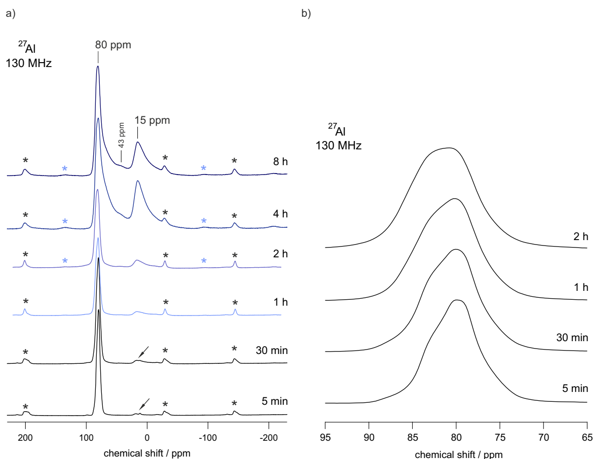
Fig. 4: a) 27 Al MAS NMR spectra of high-energy ball milled LiAlO 2 . The milling times are indicated; the spectra were recorded at a Larmor frequency of 130 MHz and a spinning speed of 15 kHz using 4-mm rotors. Asterisks mark spinning sidebands. While the spectrum of microcrystalline \gamma -LiAlO 2 as well as that of the sample milled for 5 min is composed of a single signal at 80 ppm representing Al tetrahedrally coordinated, additional intensities emerge if the milling time is increased to 1, 2, 4 and 8 h, respectively. Small arrows indicate a small amount of impurities with Al in four-fold coordination. b) Magnification of the NMR line located at 80 ppm.
