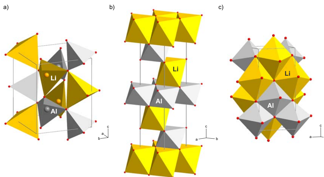
Fig. 3: Crystal structures of three different polymorphs of \text{LiAlO}_2 : a) \gamma - \text{LiAlO}_2 , the low-pressure modification, b) the high-pressure modification \alpha - \text{LiAlO}_2 and c) the high-pressure modification \delta - \text{LiAlO}_2 . In the latter two Al and Li reside on six-fold coordinated sites while in a) pairs of tetrahedrally coordinated \text{LiO}_4 and \text{AlO}_4 units build the crystal structure. In the case of \delta - \text{LiAlO}_2 the Li and Al ions share the common sites 4a and 4b; the occupancies are: 4a (Al:Li, 0.83:0.17) and 4b (Al:Li, 0.19:0.81).
