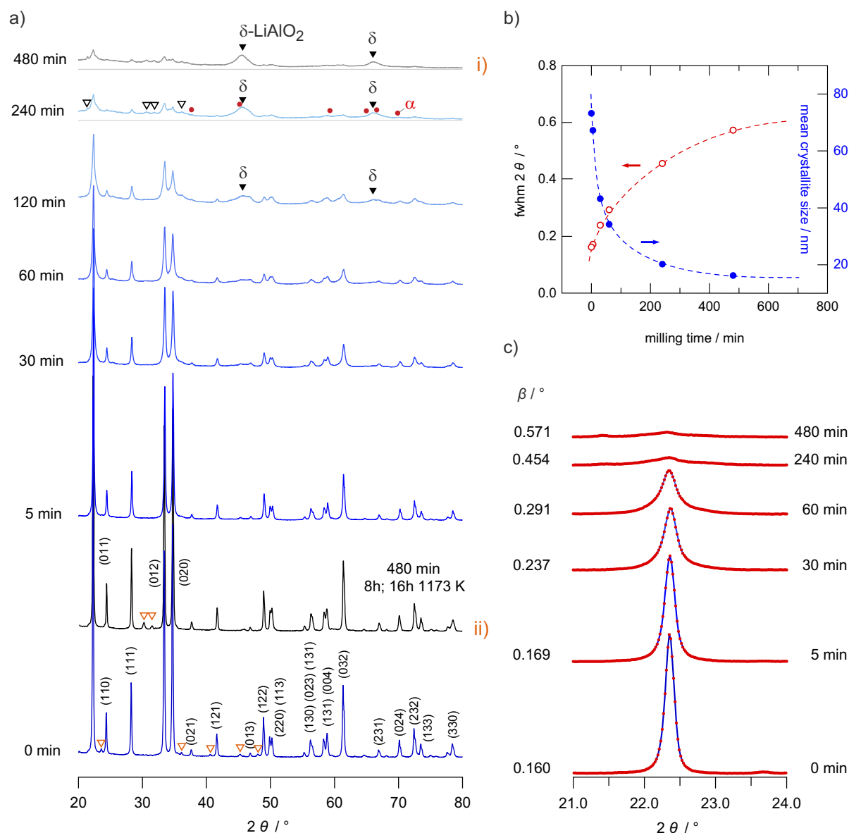
Fig. 1: XRD patterns of micro- and nanocrystalline \text{LiAlO}_2 obtained after different milling times ranging from 0 to 8 hours. With increasing milling times the XRD patterns are increasingly broadened. The broad reflections showing up after 120 min of milling ( \nabla ) most likely reflect the high pressure phase \delta\text{-LiAlO}_2 ; heat treatment at 1173 K for 16 h yields phase pure \gamma\text{-LiAlO}_2 (see pattern ii)) once again. b) Average XRD peak width (red, left ordinate) with increasing milling time. For comparison, the estimated crystallite sizes (blue, right ordinate) are shown vs milling time as well. c) Broadening of the (012) XRD peak. \beta denotes the relative broadening of the peak after correction taking into account instrumental effects.
