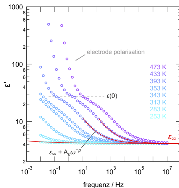
Fig. 9: Permittivity spectra of ball-milled \text{LiAlO}_2 (30 min) indicating electrical bulk response, \epsilon(0) turns out to be approximately 30 while the permittivity at infinite frequency is ca. 4. We refer to the text for further explanation and details.
