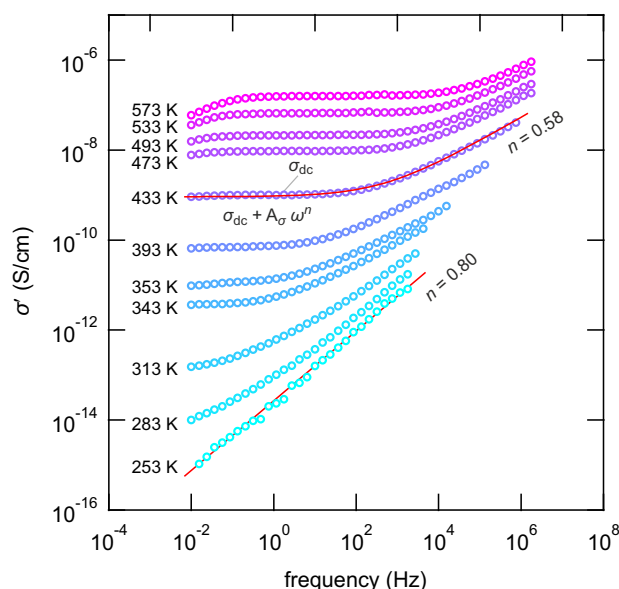
Fig. 8: Conductivity spectra of nanocrystalline LiAlO 2 measured in dry N 2 atmosphere; the source material has been milled for 30 min in a planetary mill at 400 rpm. The spectra are composed of distinct dc plateaus reflecting chiefly bulk Li ion conduction in LiAlO 2 . While dispersive regions show up at higher frequencies, in the low frequency region electrode polarization leads to deviations from the dc plateau at elevated temperature. Solid lines represent fits with appropriate power laws containing the Jonscher exponent n , see text for further explanation.
