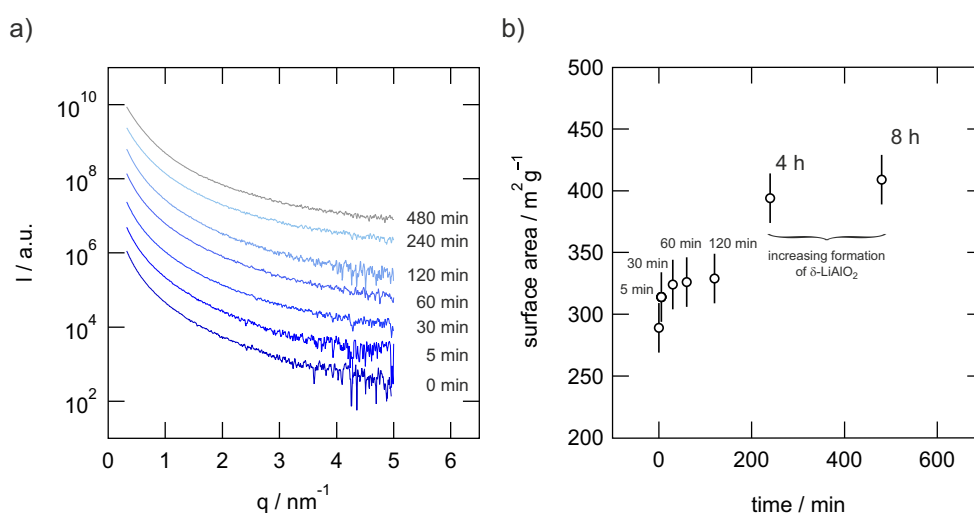
Fig. 7: a) SAXS pattern of microcrystalline and ball-milled \text{LiAlO}_2 . b) Inner surface area per mass plotted vs milling time as deduced from SAXS ( \rho = 2.615 \text{ g/cm}^3 , see Refs. [18, 32, 31]).
