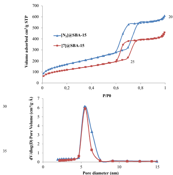
Fig.2 Nitrogen adsorption/desorption isotherms (top) and pore size distributions (bottom) of azide [N_3]@SBA-15 and clicked silica materials [7]@SBA-15 .
