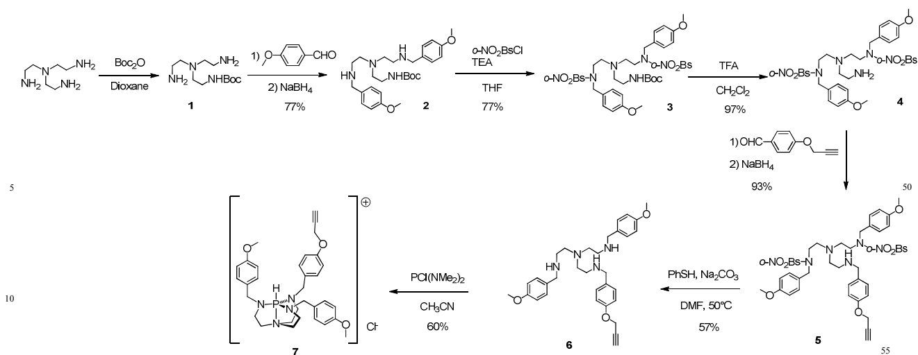
Scheme 1 Synthesis strategy to alkyne-containing azaphosphatrane.
