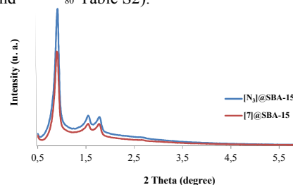
Fig. 1 X-ray powder diffraction patterns of azide functionalized SBA-15 silica material before and after click of 7 .
