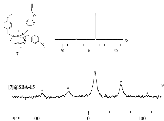
Fig. 4 Liquid ^{31}\text{P} NMR spectrum of molecular azaphosphatrane 7 and MAS ^{31}\text{P} NMR of [7]@SBA-15 . * denotes for spinning side bands.
