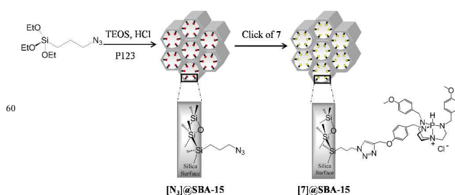
Scheme 2 Immobilization of azaphosphatrane through click chemistry.
