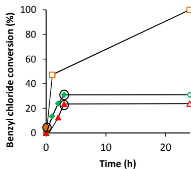
Fig. 12 Filtration tests in the benzylation of toluene for COE-4/Fe (▲/△), Al-COE-4/Fe (◆/◇) and Fe 2 O 3 -ZSM-5 (■/□). The last data points right before removing the catalysts are indicated with a circle. Open symbols represent the conversion after the catalyst was removed.
