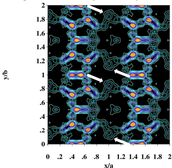
Fig. 5 The electron distribution map of COE-3/Fe showing isolines of electron density. This map was obtained from the experimental powder data set by applying a Fourier transform to the structure factors using signs from the structure model as reported. A projection of a segment of the unit cell is shown parallel to the channel axis. The colour code indicates high electron density in yellow as a result of superposition of two or more T- or O-framework atoms. The green colour indicating the linker site (white arrows) and the extra framework atoms (EFA) represents lower electron density due to single occupancies.
