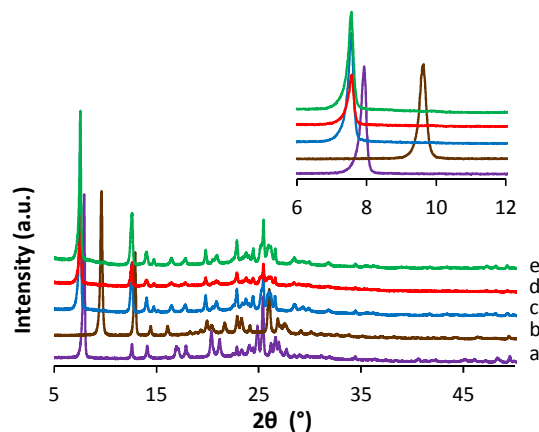
Fig. 1 Powder XRD patterns (Cu Kα 1 radiation, λ = 1.54056 Å) of RUB-36 (a), RUB-37 (b), Al-COE-4 (c), COE-4/Fe (d) and Al-COE-4/Fe (e). The inset shows a detail of the low angle region for the respective patterns.
