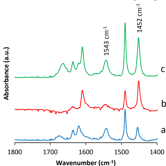
Fig. 8 Difference IR spectra (at 423 K) of adsorbed pyridine on Al-COE-4 (a), COE-4/Fe (b) and Al-COE-4/Fe (c) normalized to 10 mg cm -2 . The absorption bands at 1455-1450 cm -1 and 1550-1545 cm -1 correspond to pyridine adsorbed on Lewis resp. Brønsted acid sites.
