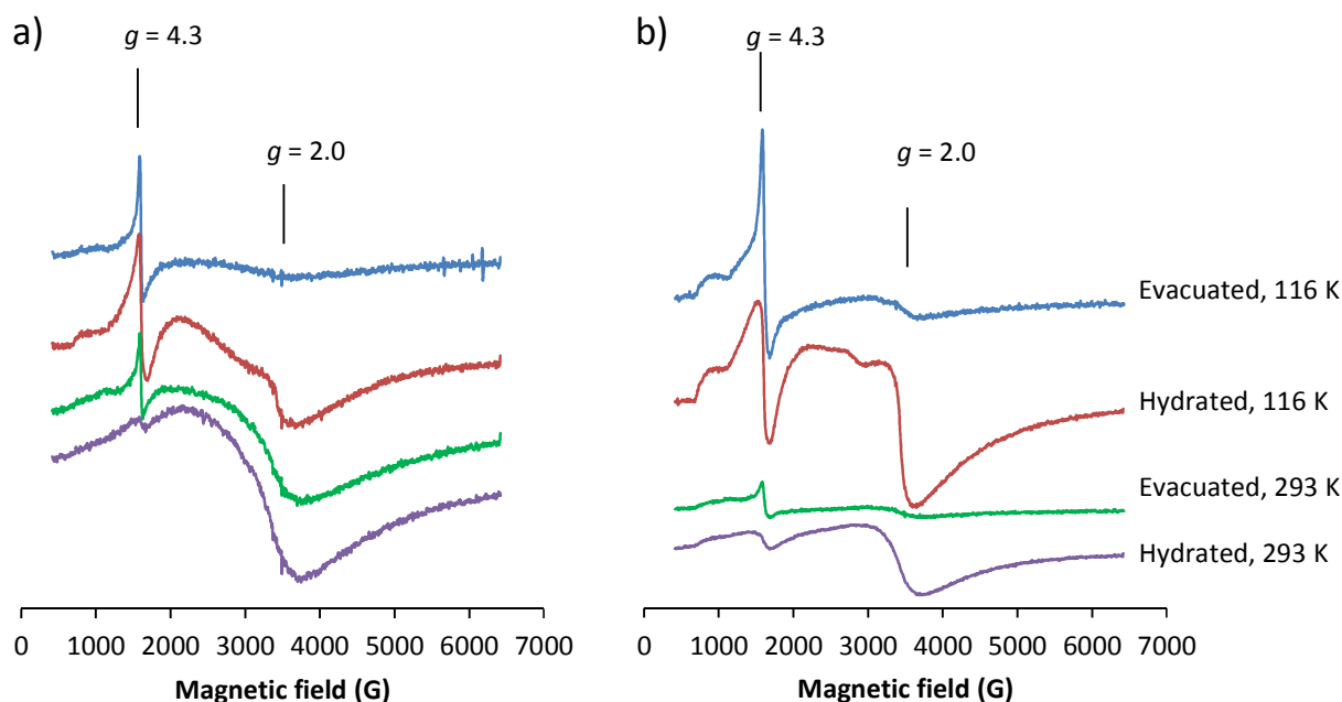
Fig. 7 EPR spectra of Fe 2 O 3 -ZSM-5 (a) and Al-COE-4/Fe (b) obtained at 116 K and 293 K (9.600 GHz). Spectra were collected before dehydration under ambient conditions and under N 2 atmosphere after evacuation.
