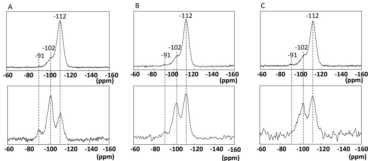
Fig. 3 Single pulse (top) and H-CP 29 Si MAS NMR spectra (bottom) of RUB-36 interlayer expanded without the use of a silylating agent or other salt (A), COE-4/Fe (B) and Al-COE-4 (C).
