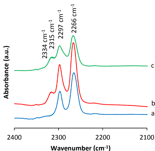
Fig. 9 C≡N stretching region of the difference IR spectra (at 298 K) of adsorbed acetonitrile on Al-COE-4 (a), COE-4/Fe (b) and Al-COE-4/Fe (c) normalized to 10 mg cm -2 .
