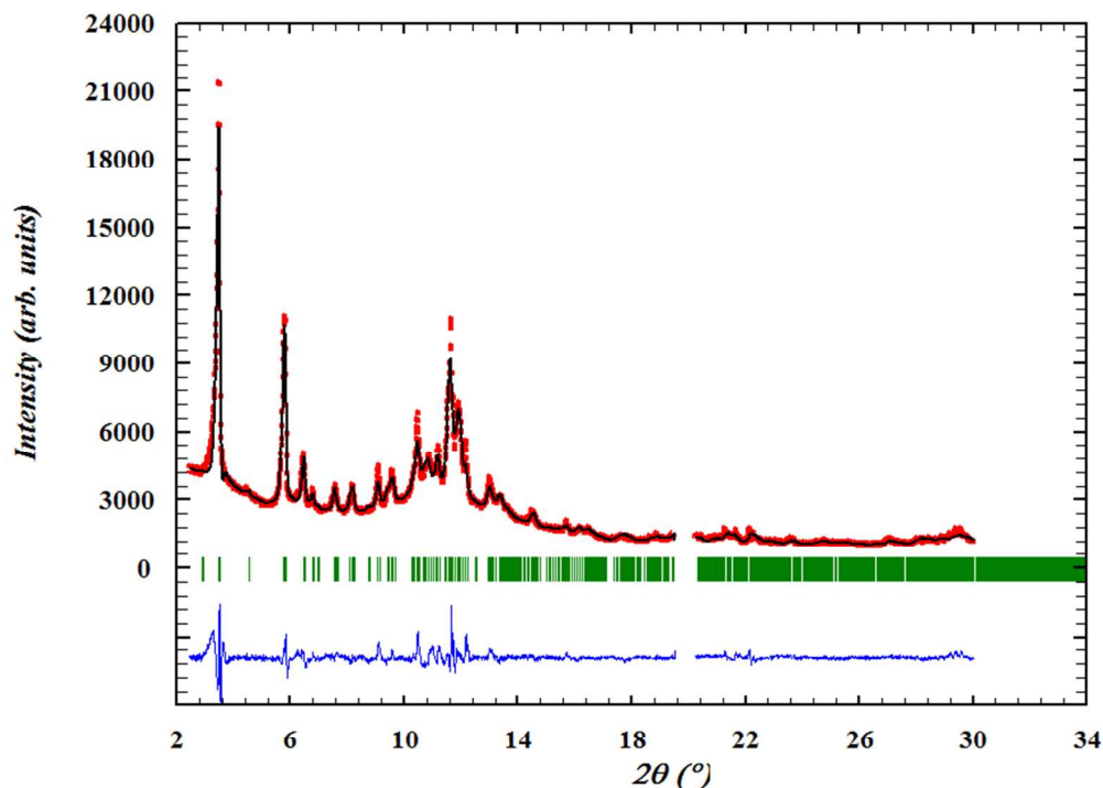
Fig. 4 Result of the Rietveld analysis of COE-3/Fe ( \chi^2 = 8.75 ). Experimental (red) and calculated (black) powder XRD pattern of COE-3/Fe (Mo K\alpha , \lambda = 0.7106 \text{ \AA} ) and the difference plot (blue) are shown.
