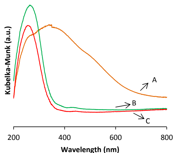
Fig. 6 UV-vis spectra of Fe 2 O 3 -ZSM-5 (A), Al-COE-4/Fe (B), and COE-4/Fe (C).
