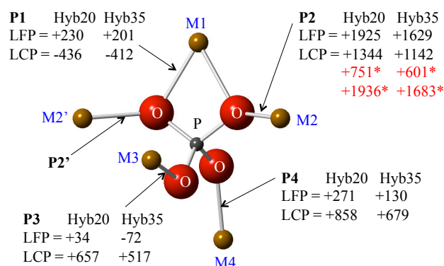
Fig. 1 The P environment in \text{LiMPO}_4 ( \text{M} = \text{Fe}, \text{Co} ) compounds. The first coordination shell of transition metals contains five M sites, leading to four distinct M-O-P pathways. The calculated FCS (ppm) are shown separately for LFP and LCP from ab initio hybrid DFT calculations using the Hyb20 (B3LYP) and Hyb35 exchange-correlation functionals. *First principles calculations on LCP at 0 K reveal a low energy ground state, which lifts the degeneracy of the P2 and P2' pathways. An average of the two pathway contributions is assumed in this room temperature study.
