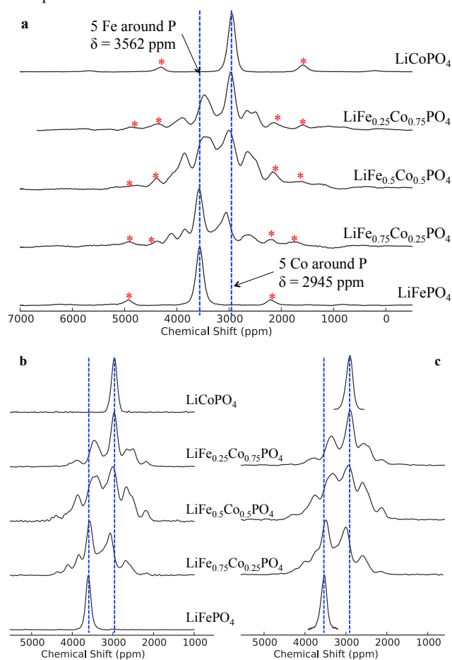
Fig. 3 The 31 P MAS NMR spectra of LiFe x Co 1-x PO 4 (where x = 1, 0.75, 0.5, 0.25, 0 ). In (a), the spectra were acquired using a MAS frequency, \nu_r , of 55 kHz and a 100 MHz magnetic field strength. Spinning sidebands are marked with asterisks. Most peaks in the mixed phases lie beyond those assigned to the all-Fe and all-Co P environments (i.e., outside the region contained within the two blue dashed lines). The 1D 31 P MAS NMR spectra of the isotropic resonances in LiFe x Co 1-x PO 4 ( x = 1, 0.75, 0.5, 0.25, 0 ) acquired at (b) \nu_r = 40 kHz extracted from the 2D MATPASS pulse sequence at a 200 MHz magnetic field and at (c) \nu_r = 60 kHz extracted from the 2D aMAT pulse sequence acquired at a 500 MHz magnetic field. The slight additional broadening in (c) is attributed to a temperature distribution in the rotor.
