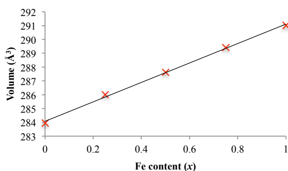
Fig. 2 Plot showing the dependence of the unit cell volume on Fe content across the LiFe x Co 1-x PO 4 series. The linear correlation ( R^2 = 0.9983 ) follows Vegard's law.
