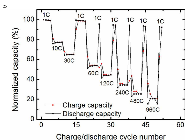
Fig 8 Rate performance test between 1 and 960 C for a sample prepared using 500 ALD-cycles, showing stable cycling at 960 C and recovery of the capacity after cycling at 1 C. The capacity is normalized to the capacity at 1 C (118 mAh/g).
