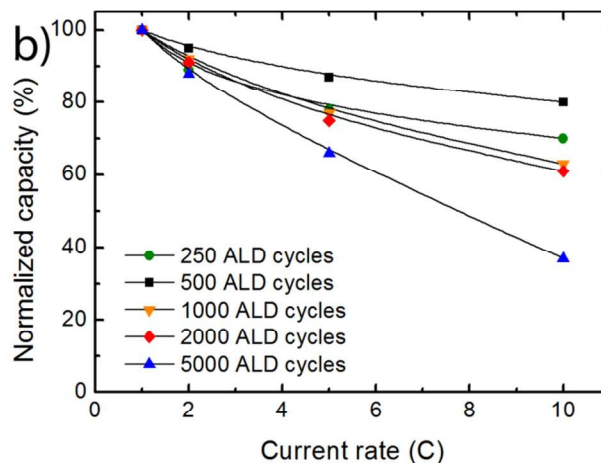
Fig 6 a) Rate performance of coin cells with V_2O_5 deposited during 250 to 5000 ALD cycles investigated over the voltage range 2.75 – 3.80 V. The cells were cycled six times at each C-rate. Charge and discharge data are represented by open and closed symbols, respectively. Note; open symbols overlap partly with filled symbols b) capacity retention after second discharge, normalized to 1 C capacity.
