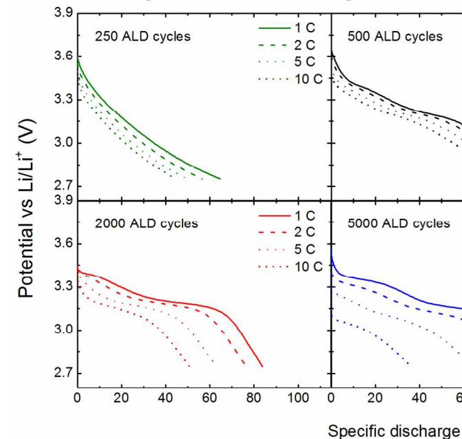
Fig 5 Voltage vs. capacity curves of coin cells with V_2O_5 as cathode deposited during 250 – 5000 ALD-cycles. Discharge rates 1 – 10 C, voltage window 2.75 – 3.80 V.
