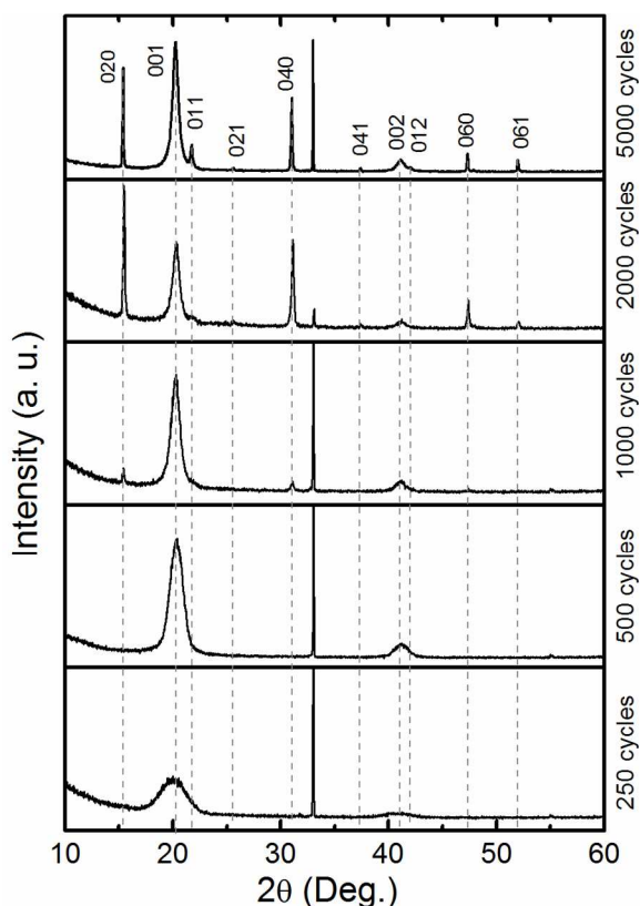
Fig 3 \theta - 2\theta x-ray diffractogram of samples deposited on silicon for different numbers of ALD-cycles. The samples are crystalline already at 250 cycles. The orientation of crystallites is predominantly along [001] for samples deposited using less than 1000 cycles, while along [001]/[010] at 2000 cycles and rather random orientations at 5000 cycles. The reflection at 32^\circ is Si(200) from the single crystalline Si-substrate.
