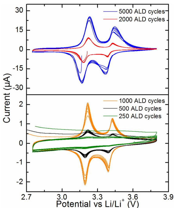
Fig 4 Cyclic voltammetry of V_2O_5 thin films in the voltage range 2.75 – 3.80 V at a scan rate of 0.1 \text{ mVs}^{-1} .
