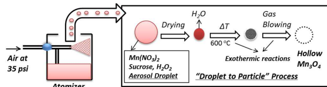
Figure 1. Schematic formation of hollow \text{Mn}_3\text{O}_4 spheres in a “droplet to particle” aerosol spray pyrolysis process.
