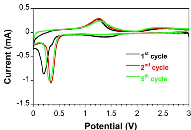
Figure 6. Cyclic voltammograms of the 1 st , 2 nd and 5 th cycles of hollow \text{Mn}_3\text{O}_4 spheres (scan rate 0.1 mV/s).
