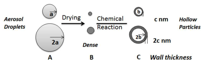
Figure 3. The ideal relationship of wall thickness of hollow particle with initial aerosol droplet size. Note: The process is based on an ideal gas blowing assumption that all gases produced in chemical reactions are used for blowing the particles.
