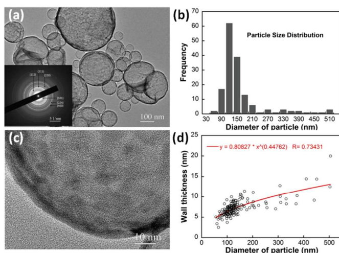
Figure 2. (a) TEM and SAED images of as collected hollow \text{Mn}_3\text{O}_4 spheres; (b) Particle size distribution of hollow \text{Mn}_3\text{O}_4 spheres based on TEM measurement; (c) High resolution TEM image of hollow \text{Mn}_3\text{O}_4 sphere; (d) The relationship of wall thickness of hollow \text{Mn}_3\text{O}_4 with particle size. Notes: the total counts are 158 in (b, d)
