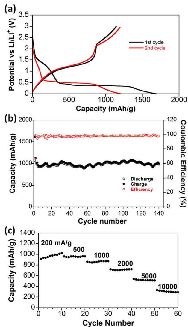
Figure 7. Electrochemical performance of hollow \text{Mn}_3\text{O}_4 spheres as electrode materials. (a) Charge/discharge profiles for the initial two cycles at a current density of 200 mA/g; (b) Cycling performance at a current density of 200 mA/g; (c) Rate performance at different current densities.
