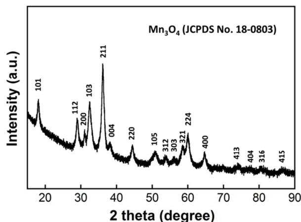
Figure 4. X-ray diffraction pattern of hollow \text{Mn}_3\text{O}_4 spheres.
