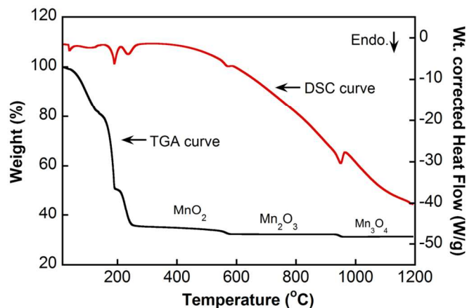
Figure 5. TGA-DSC curves of \text{Mn}(\text{NO}_3)_2 \cdot 4\text{H}_2\text{O} decomposition in air. (Heating rate: 10 °C/min, air flow: 100 ml/cm 3 )
