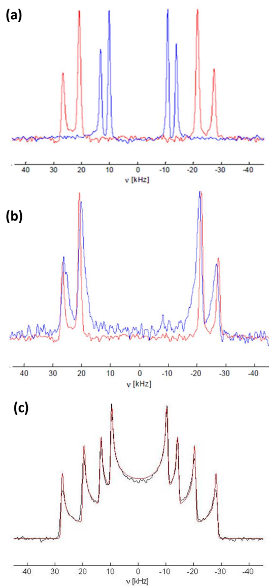
Figure 2. (a) ^2\text{H} NMR spectra of the aligned sample (red) and after a flip by 90^\circ with respect to the magnetic field (Blue) in the N_X phase at 90^\circ\text{C} . (b) ^2\text{H} NMR spectrum 10s after the 90^\circ flip
