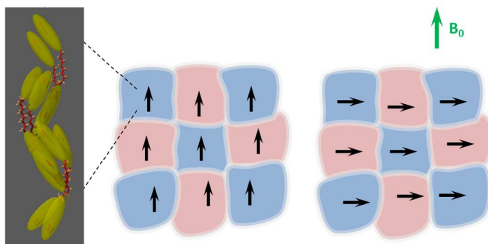
Figure 4. Proposed chiral domain structure of the N_x phase. The different domain colors indicate opposite chiralities (sense of molecular twisting). The inset (left) shows a possible disposition of the mesogenic units within each domain, stressing the lack of full alignment of all the units parallel to a unique direction. The internal orientational order of each domain is represented by a domain director. The magnetic field aligns the domain directors (middle). On rotating the sample (right), the mutual alignment of the domain directors persists sufficiently long on the NMR measurement time-scale.
