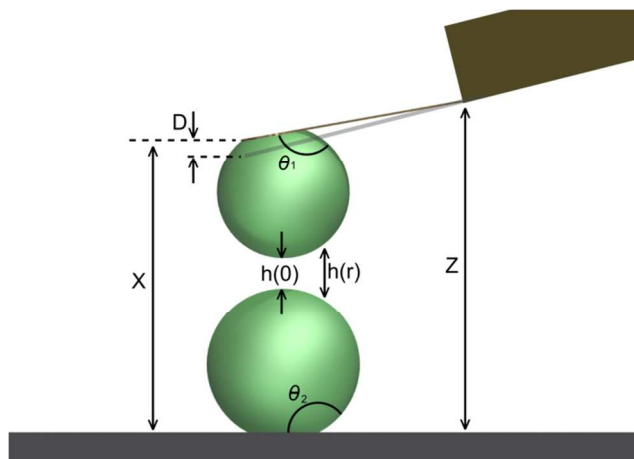
Fig. 1 Diagram of experimental setup during an AFM experiment between two drops. Z is piezo position, D is cantilever deflection, X is effective end to end drop separation, h(r) is drop separation at radial position r , and \theta is contact angle.
