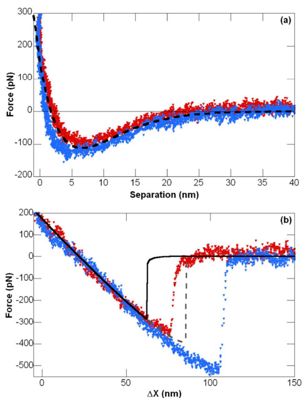
Fig. 5 a) Force versus separation data between a rigid silica particle (radius 4 \mu\text{m} ) and a silica surface in 80 mM CTAB with 24 mM NaSal at 25°C. Symbols are AFM data for approach (red) and retract (blue). The dashed black line is a fit using the semi-empirical equation described previously. b) Modelling results using the fit to the rigid data calculated by the Chan-Dagastine-White model overlaid onto AFM data from figure 2 with considerations for jump ins and jump outs taken from data. The solid lines are the expected behaviour for approach (solid black) and retract (dashed grey).
