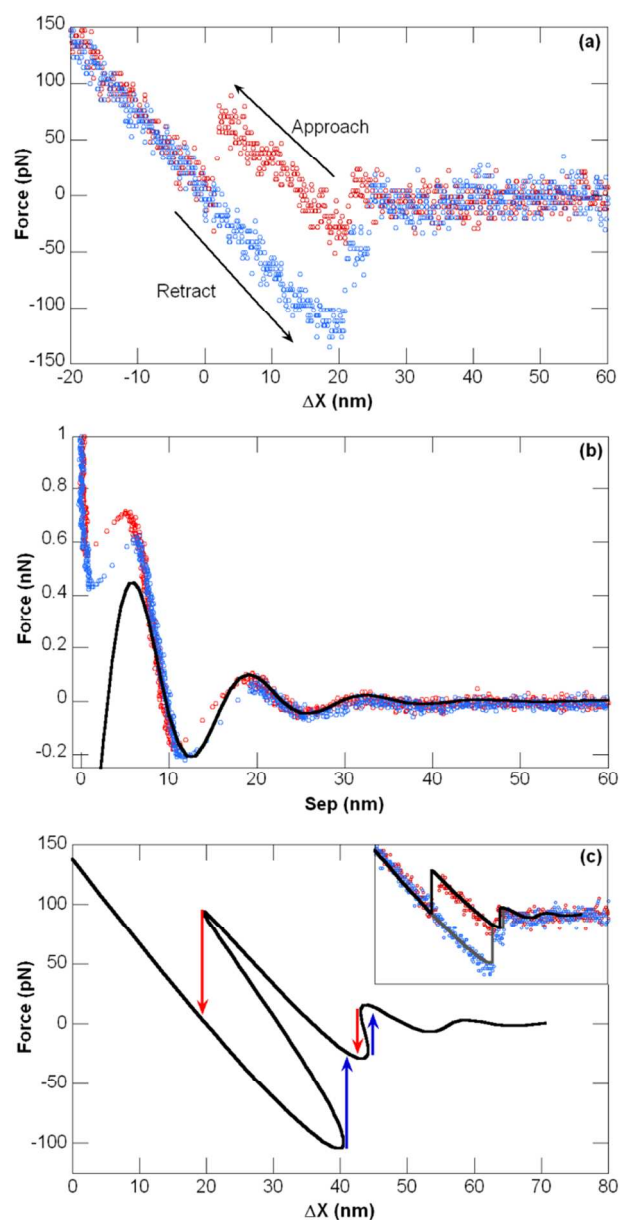
Fig. 2 a) Interaction forces between two perfluorooctane droplets (diameters 61 and 63 \mu\text{m} ) in solution of 80 mM CTAB at 27°C. Symbols are experimental AFM data for approach (red) and retract (blue). b) Interaction forces for 80 mM CTAB at 27°C between a rigid silica particle (radius 7 \mu\text{m} ) and a silica surface. The solid black line is a fit using the semi-empirical equation described previously. c) Modelling results for two perfluorooctane droplets (diameters 61 and 63 \mu\text{m} ) calculated by the Chan-Dagastine-White model using the fit to the solution forces in b). Inset: Model overlayed onto AFM data from a) with considerations for jump ins and jump outs taken from data.
