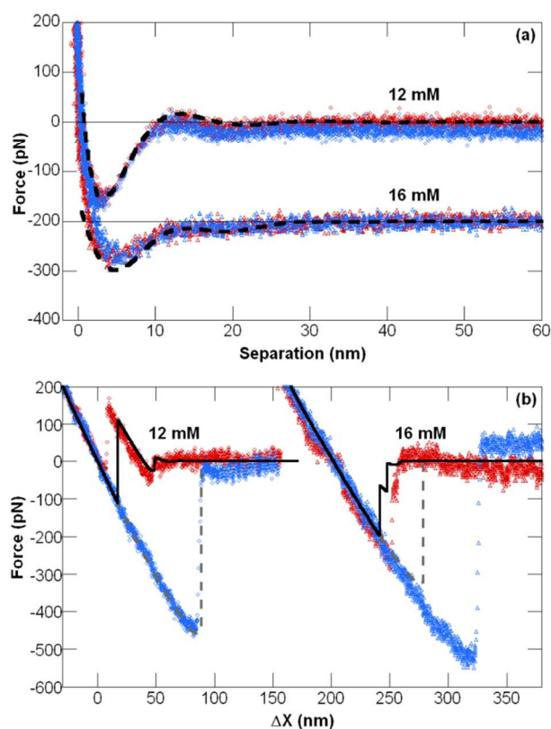
Fig. 4 a) Force versus separation data between a rigid silica particle (radius 4 \mu\text{m} ) and a silica surface in 80 mM CTAB with 12 mM NaSal at 25°C and 16 mM NaSal at 25°C. Symbols are AFM data for approach (red) and retract (blue). The dashed black lines are fits using the semi-empirical equation described previously. b) Modelling results using the fits to the rigid data calculated by the Chan-Dagastine-White model overlaid onto AFM data from figure 2 with considerations for jump ins and jump outs taken from data. The solid lines are the expected behaviour for approach (solid black) and retract (dashed grey).
