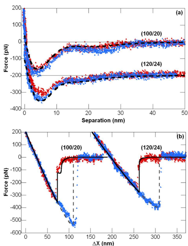
Fig. 6 a) Force versus separation data between a rigid silica particle (radius 4 \mu\text{m} ) and a silica surface in 100 mM CTAB with 20 mM NaSal at 25°C and 120 mM CTAB with 24 mM NaSal at 25°C. Symbols are AFM data for approach (red) and retract (blue). The dashed black lines are fits using the semi-empirical equation described previously. b) Force versus separation data between PFO droplets in 100 mM CTAB 20 mM NaSal, droplet diameters are 72 and 66 \mu\text{m} , 25°C and 120 mM CTAB 24 mM NaSal, droplet diameters are 69 and 72 \mu\text{m} , 25°C. Modelling results using the fits to the rigid data calculated by the Chan-Dagastine-White model are overlaid with considerations for jump ins and jump outs taken from data. The solid lines are the expected behaviour for approach (solid black) and retract (dashed grey).
