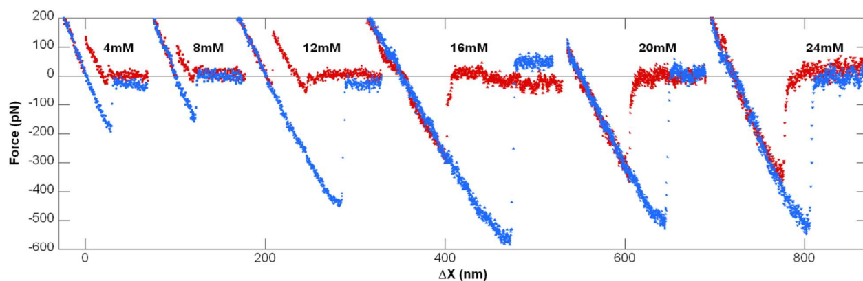
Fig. 3 Interaction forces between two perfluorooctane droplets in 80 mM CTAB solutions with increasing amounts of NaSal at 26°C. Plots offset horizontally for convenience. From left to right the solutions are: 4mM NaSal, droplet diameters are 71 and 72 \mu\text{m} , 26°C; 8 mM NaSal, Droplet diameters are 75 and 78 \mu\text{m} ; 12 mM NaSal, Droplet diameters are 72 and 83 \mu\text{m} ; 16 mM NaSal, Droplet diameters are 72 and 75 \mu\text{m} ; 20 mM NaSal, Droplet diameters are 72 and 82 \mu\text{m} ; 24 mM NaSal, Droplet diameters are 71 and 69 \mu\text{m} .
