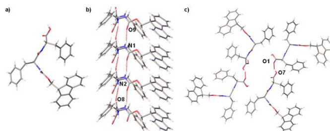
Figure 4 Single crystal structure of FmocFF( \text{H}_2\text{O} ) _{0.875} showing four FmocFF molecules stacked parallel along the crystallographic b axis, perspective view [010] (a), these are hydrogen bonded together (b). Crystal packing showing four parallel stacks of FmocFF molecules, these are centred around a twofold rotation axis, perspective view [010] (c). Hydrogen bonding interactions shown as dotted line, diffuse solvent omitted for clarity.
