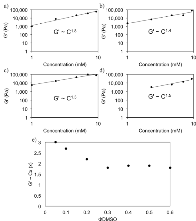
Figure 7 Comparison of the relationship between G' and gelator concentration for FmocFF gels prepared using a) DMSO b) ethanol c) acetone and d) HFIP. All gels were prepared with \Phi_{\text{solvent}} of 0.3. In all cases, data were taken from the LVE region at a frequency of 10 rad/s. All data were collected on gels which had been aged for 24 hours. e) Shows the exponents determined for FmocFF gels with different \Phi_{DMSO} . All gels in (e) have a final gelator concentration of 5 mg/mL.
