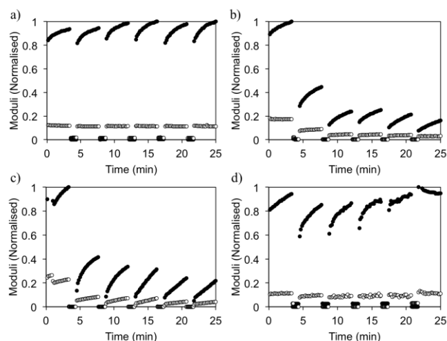
Figure 6 Rheological measurements showing recovery after shear of FmocFF gels with \phi_{\text{solvent}} of 0.3 for the solvents a) DMSO b) ethanol c) acetone and d) HFIP. G' and G'' are represented by ● and ○, respectively. Data has been normalised.
