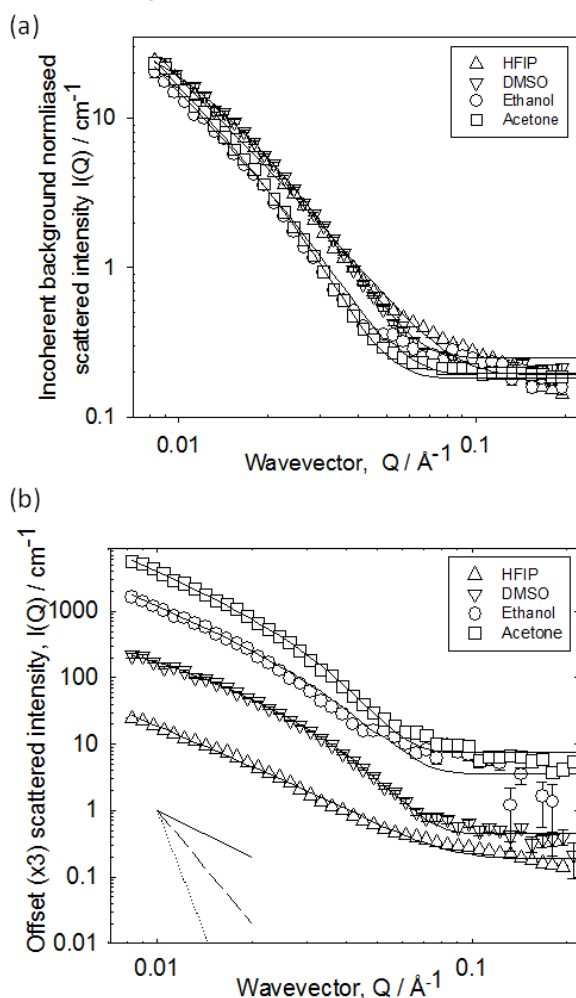
Figure 2 (a) SANS data for gels formed at a \phi_{\text{solvent}} of 0.3. The data are normalised for subtle differences in incoherent background. (b) Data offset by factors of three for clarity. In both cases, fits to the Kholodenko-Dirac worm model are shown. In (b), the inset demonstrates the decays for Q^{-1} , Q^{-2} , and Q^{-4} .
