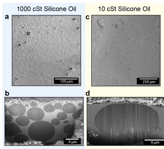
Figure 3 | Visualization of submerged droplets (a) 1000 cSt silicone oil surface with condensed droplets as observed in SEM. The sample was prepared using Cryo-FIB-SEM technique where condensed water micro-droplets and the liquid surface are cryopreserved in vitreous state and subsequently milled using an ion beam and imaged using an electron-beam. (b) Cross-sectional view of cryo-FIB sectioned surface of 1000 cSt oil showing presence of droplets within the oil in different depths. (c) 10 cSt Silicone oil surface as observed in SEM before sectioning. (d) Cross-sectional view of cryo-FIB sectioned surface of 10cst oil showing presence of a single droplet near the oil-air interface. The droplet appears ellipsoidal because the sample is inclined by 52^\circ .
