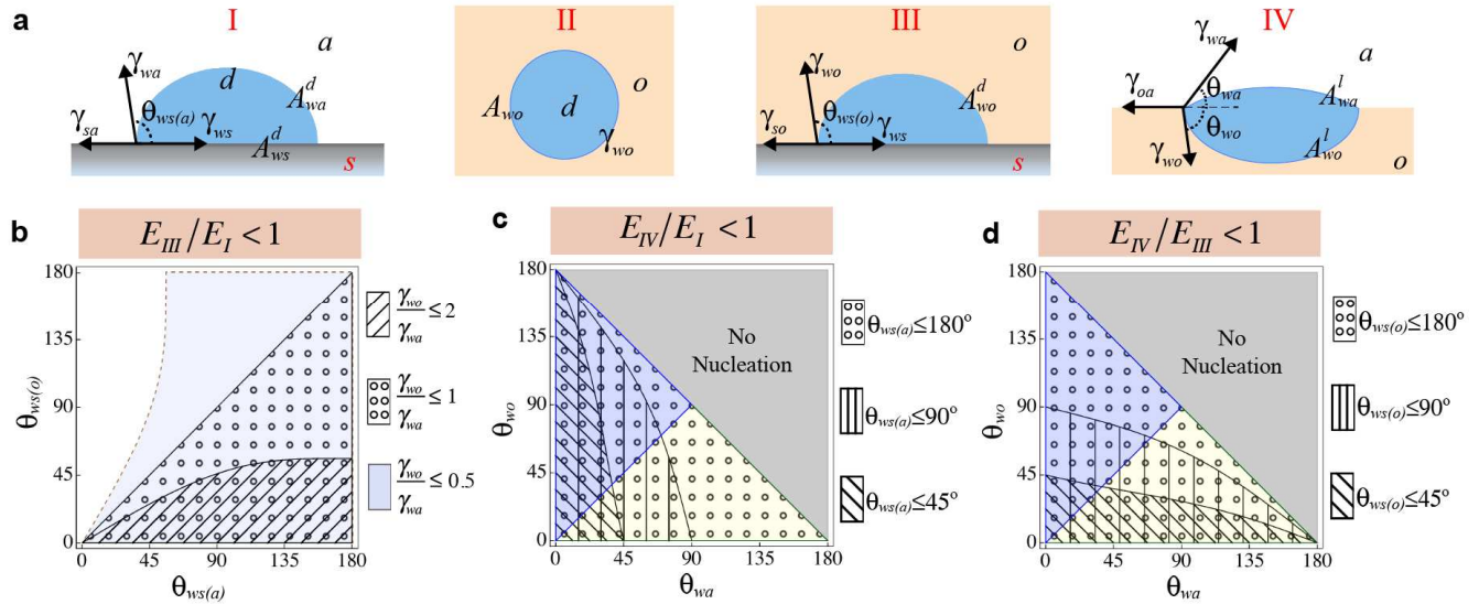
Figure 1 | Nucleation states and regime maps of nucleation preference. (a) Possible pathways of nucleation between a condensing drop and its environment. The subscripts w , a , o and s denote droplet, air, oil and solid interfaces respectively. The superscripts d and l denote droplet and lens. In State I and III, A_{ws}^d and A_{wa}^d corresponds to droplet-solid and droplet-air interfacial areas. In State II, A_{wo} corresponds to droplet-oil interfacial area. In State IV, A_{wo}^l and A_{wa}^l correspond to lens-oil and lens-air interfacial areas. (b) The regime map showing conditions where nucleation within the oil is preferred over nucleation in vapor for different ratios of \gamma_{wo}/\gamma_{wa} . (c) Regime map showing conditions where nucleation at the oil-air interface is preferred over nucleation at solid-air interface for different solid surface wettabilities ( \theta_{ws(a)} ). (d) Regime map showing conditions where nucleation at the oil-air interface is preferred over nucleation within the oil for different surface wettability in oil ( \theta_{ws(o)} ). In (c) and (d), the region with blue background corresponds to oils that satisfy the criterion \gamma_{wo} \leq \gamma_{wa} while the region with green background corresponds to oils with \gamma_{wo} \geq \gamma_{wa} .
