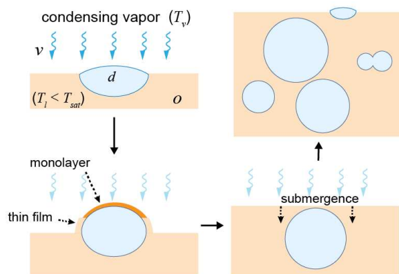
Figure 4 | Schematic of the droplet nucleation and submergence mechanism on cloaking liquids
