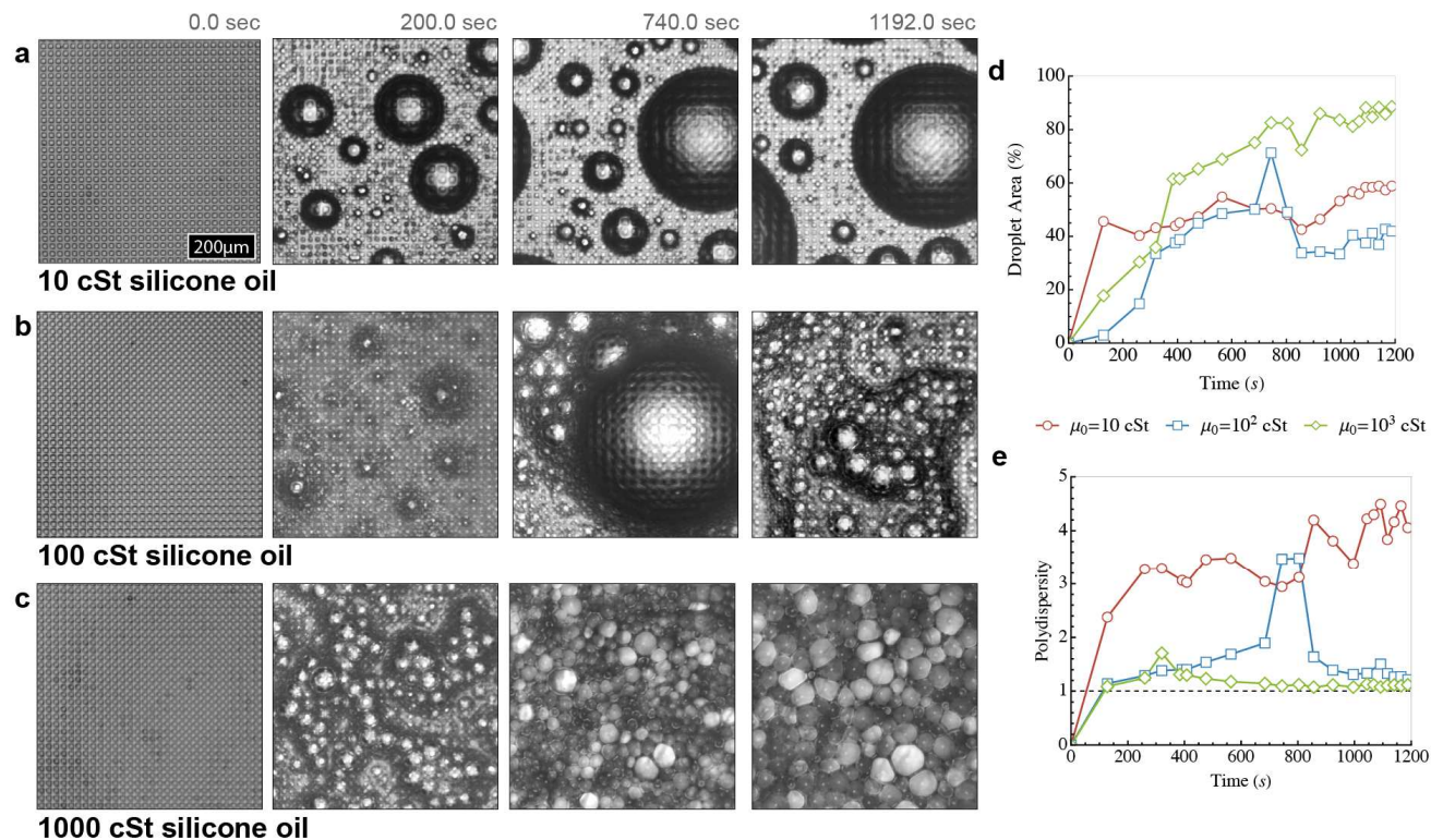
Figure 6 | Effect of liquid viscosity during condensation on LIS. (a) Time sequence showing growth of condensed droplets as observed under microscope on micropost surface (identical surface as used for Fig. 5) impregnated with Silicone oil of viscosity (a) 10 cSt, (b) 100 cSt and (c) 1000 cSt. The experiments were performed in an open environment under the same conditions (Peltier temperature= 3 \pm 1 °C, dew point= 12 \pm 1 °C). Even on 100 cSt, significant resistance to coalescence is observed. On 1000 cSt Silicone oil surface, there is significant inhibition against coalescence and condensed droplets are separated through a thin oil film that takes orders of magnitude larger time to collapse as compared to droplets cloaked with 10 and 100 cSt viscosity silicone oil. (d) Plot comparing the variation of droplet occupied area fraction versus time on 10, 100 and 1000 cSt silicone oil impregnated surfaces. On 10 cSt surface, the droplet coverage reaches \sim 55\% as is normally observed on condensation on solid surfaces. On 100 cSt surface, there is an initial delay in forming of large droplets within the observed frame, but large size
