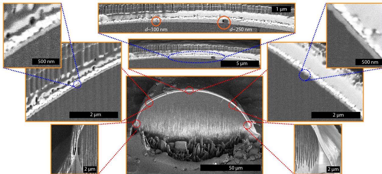
Figure 5 | Nanofilm profile around a condensed droplet suspended on LIS. Liquid film profile around the droplet (droplet size > micropost spacing) on 10 cSt silicone oil obtained through Cryo-FIB-SEM process. The micropost surface was OTS coated silicon samples with micropost arrays ( a=b=h=10\ \mu\text{m} , where a is the post width, b is the edge- to-edge spacing between posts). The light grey color in the images sandwiched between the dark grey (water) and white (platinum) signifies Silicone oil of viscosity 10 cSt. Different sections around the droplet were imaged separately after milling the droplet. The higher magnification images are overlapped on the image of the entire droplet as aid for visualization. Within the liquid cloak, presence of two separate nano-droplets is noticeable. Because of the sample tilt, and its position with respect to the detector, different sections of the droplet are located at different depths of focus, thus giving different contrast. For this reason, the left section of the droplet profile looks darker while the right section of the droplet profile looks evenly bright, even though the entire surface is coated with the same chemical (Platinum). The image content beyond edge of the cross-section (above edge of Pt coating) is out-of-focus with each pixel signal coming from a broad volume and is meaningless. A full-scale image of the nano-droplets within the cloak can also be visualized through Supplementary Image S11.
