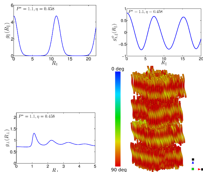
Fig. 8 The functions g_{\parallel}(R_{\parallel}) (top left) and g_{1,\parallel}^{\widehat{w}}(R_{\parallel}) (top right) at P^* = 1.1 , for helices with r = 0.2 and p = 8 ( Sm_{A,S}^* phase). Also depicted is g_{\perp}(R_{\perp}) (bottom left) and a corresponding snapshot colour coded according to the local tangent to helices (bottom right).
