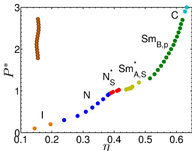
Fig. 5 Equation of state for helices having r = 0.2 and p = 8 . Different colours indicate different phases: I=isotropic; N=nematic; N_S^* =screw-nematic; Sm_{A,S}^* =screw-smectic A; Sm_{B,p} = smectic B polar.
