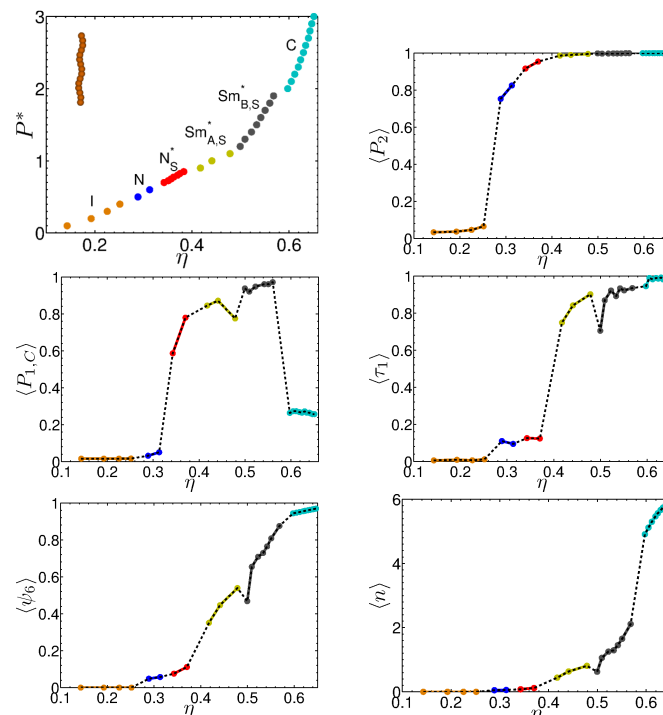
Fig. 11 Equation of state and order parameters \langle P_2 \rangle , \langle P_{1,c} \rangle , \langle \tau_1 \rangle , \langle \psi_6 \rangle and average nearest-neighbors \langle n \rangle , (in typewriter order) in the case r = 0.2 and p = 4 . Note that in the plot for the equation of state (top, left), additional points between the two extrema, have been included in the N_S^* phase, for completeness.
