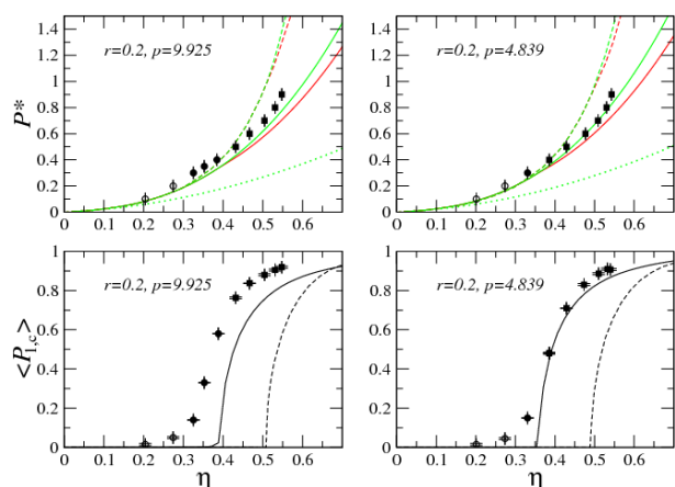
Fig. 17 Equation of state (top) and screw-nematic order parameter as a function of the volume fraction \eta (bottom), for perfectly aligned hard helices with r = 0.2 and p = 9.925 (left) and p = 4.839 (right). Results from Onsager theory (dotted), from modified PL theory (dashed) and from third-virial theory (solid). Top panels: green is for the N phase and red for the N_S^* phase. Symbols are results from MC simulations: N (empty circles), N_S^* (full circles) and Sm_S^* (full squares).
