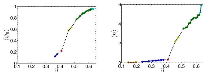
Fig. 10 Hexatic order parameter \langle \psi_6 \rangle and average nearest-neighbour number \langle n \rangle , both indicative of in-plane hexatic ordering, for helices with r = 0.2 and p = 8 . State points belonging to different phases are colour as in Fig. 5.
