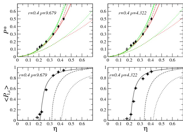
Fig. 18 Equation of state (top) and screw-nematic order parameter as a function of the volume fraction \eta (bottom), for perfectly aligned hard helices with r = 0.4 and p = 9.679 (left) and p = 4.322 (right). Results from Onsager theory (dotted), from modified PL theory (dashed) and from third-virial theory (solid). Top panels: green is for the N phase and red for the N_S^* phase. Symbols are results from MC simulations: N (empty circles), N_S^* (full circles) and Sm_S^* (full squares).
