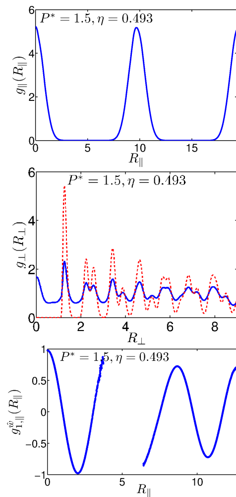
Fig. 13 Top panel. Plot of g_{\parallel}(R_{\parallel}) in the case of r = 0.4, = 4 , at reduced pressure P^* = 1.5 ( \text{Sm}_{B,S}^* phase). Central panel. Profile of g_{\perp}(R_{\perp}) calculated by averaging over all layers (solid line) and over a single layer (red dotted line). Bottom panel. Behavior of g_{1,\parallel}^{\hat{w}}(R_{\parallel}) .
