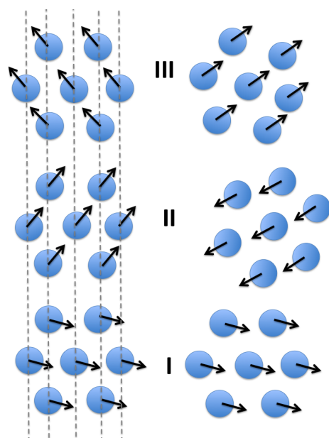
Fig. 14 Cartoon of the smectic B phases discussed in the text. Circles represent transversal sections through the center of helices and arrows the corresponding \hat{w} vectors. I,II, III indicate adjacent layers. Left: \text{Sm}_{B,S}^* phase, with through-layers positional correlation (AAA structure, highlighted by the dashed lines) and screw-like (orientational) correlation of \hat{w} vectors. Right: \text{Sm}_{B,p} phase, with in-layer correlation of \hat{w} vectors and neither positional nor orientational correlation between layers.
