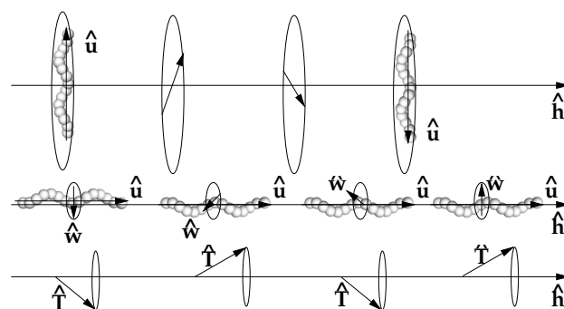
Fig. 20 Cartoon of the cholesteric (top), and of the screw-nematic (middle) organization. Here \hat{h} is a unit vector parallel to the axis around which either the molecular axis \hat{u} (cholesteric) or \hat{w} (screw-nematic) spirals, respectively. In the latter case, the tip of the tangent to the helices \hat{T} forms a conical path (bottom).
