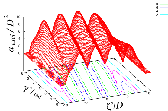
Fig. 16 The function a_{excl}(\zeta', \gamma') (see Eq. 22), calculated for helices with r = 0.4 and p = 4.322 .
