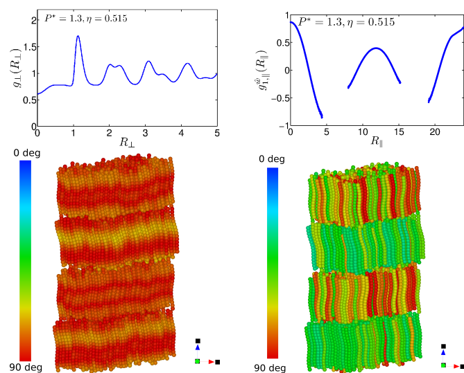
Fig. 9 Behaviour of g_{\perp}(R_{\perp}) (top left) and g_{\parallel}(R_{\parallel}) (top right) and relative snapshot, colour coded according to the local tangent (bottom left) and to the C_2 axis (bottom right) at P^* = 1.3 , in the case r = 0.2 and p = 8 . This state point belongs to the Sm_{B,p} phase. Note that in the case of the C_2 axis, azimuthal rotations of angles in the range [90^\circ, 180^\circ] are colour coded in the same way as in the case [0^\circ, 90^\circ] because of the limitations in the QMGA software 41 . For this reason, this color coding will not be further exploited in the remaining of the paper.
