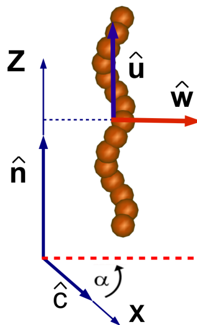
Fig. 4 Helix with arrows showing the unit vectors \hat{\mathbf{u}} and \hat{\mathbf{w}} defined in the molecular frame, and the unit vectors ( \hat{\mathbf{n}}, \hat{\mathbf{c}} ) defined in the laboratory frame. X, Z are the axes of the laboratory frame, with \alpha the angle between \hat{\mathbf{w}} and the X axis.
