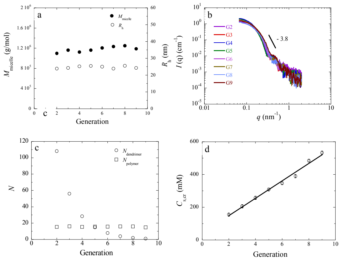
Figure 2 Micellar mass, M_{\text{micelle}} and hydrodynamic radius, R_h (a), SAXS profiles (b), aggregation number N (c), and critical salt concentration C_{s,\text{cr}} (d) of Gn-C3Ms incorporating PAMAM dendrimers of different generations in the range G2-G9. Micelles are prepared in \text{NaHCO}_3/\text{Na}_2\text{CO}_3 buffer (20 mM, pH 10) at the PMC.
