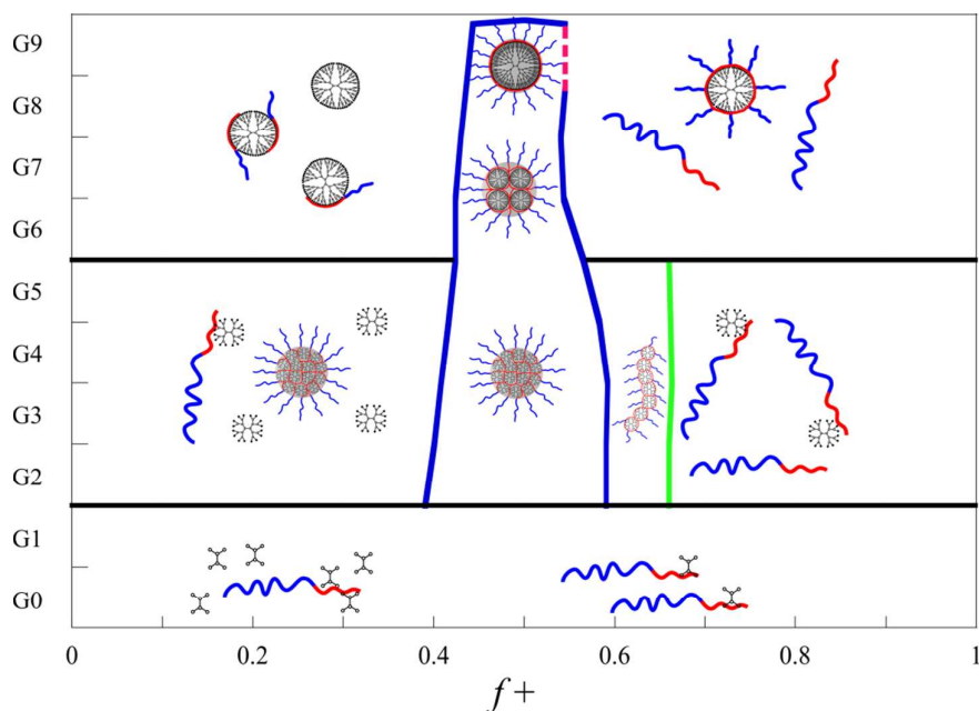
Figure 5 General state diagram of the dominant structures formed by PAMAM dendrimer and P2MVP 128 -b-PEO 477 polymers upon varying mixing charge fraction and dendrimer generation. For micelles around PMC, the dendrimer numbers are not scaled to real aggregation number and only highlight the decay trends with increasing dendrimer generation.
