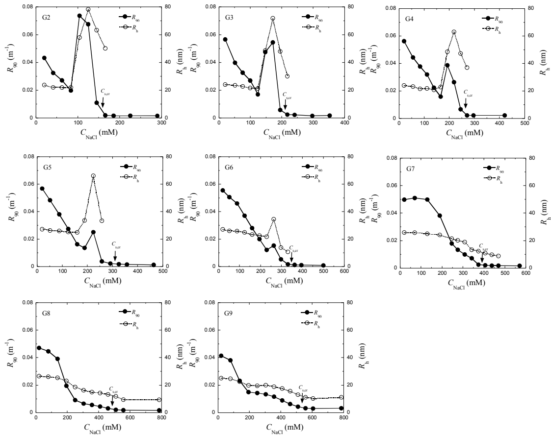
Figure 3 Variation of light scattering intensity R_{90} and hydrodynamic radius R_h of Gn-C3Ms with increasing salt concentration, which is the sum of added NaCl concentration and the concentration of buffer viewed as 1-1 type electrolyte.
