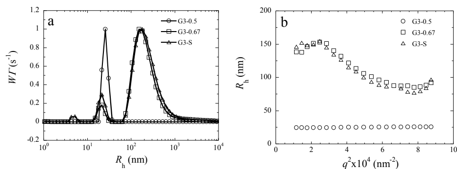
Figure 4 Size distribution (a, \theta = 90^\circ ) and angular dependence of the average hydrodynamic radius (b, 40^\circ \leq \theta \leq 140^\circ ) of G3-C3Ms at f + 0.5 , 0.67 and at f + 0.5 with 160 mM NaCl in buffer solution.
