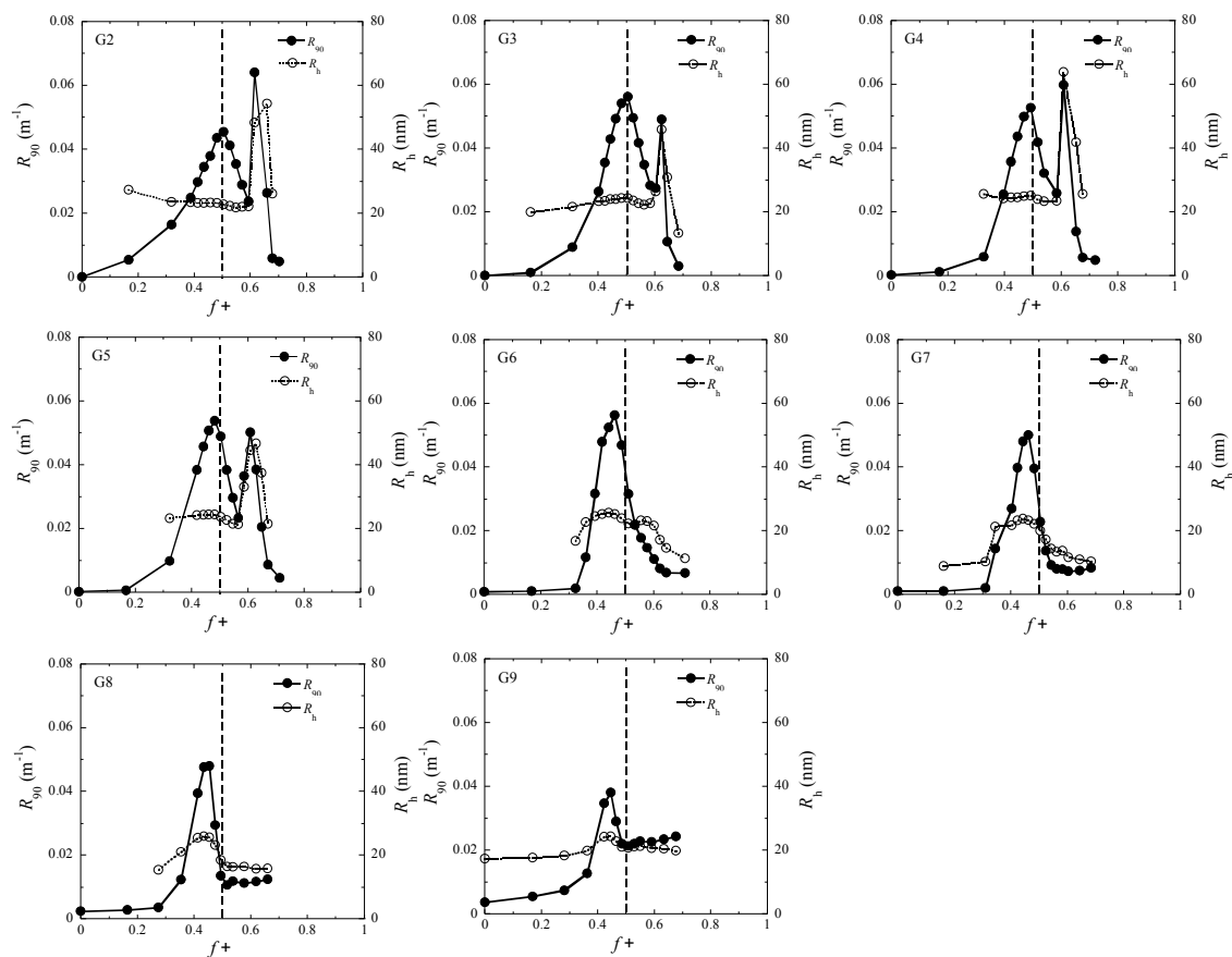
Figure 1 Light scattering titration of PAMAM dendrimers at different generations with P2MVP 128 - b -PEO 477 . The light scattering intensity R_{90} and hydrodynamic radius R_h are plotted as a function of positive charge fraction f^+ . The dashed line shows the position of the theoretical f^+ = 0.5 , and deviations from that line reflect the presence of defects and impurities in the dendrimer batch.
