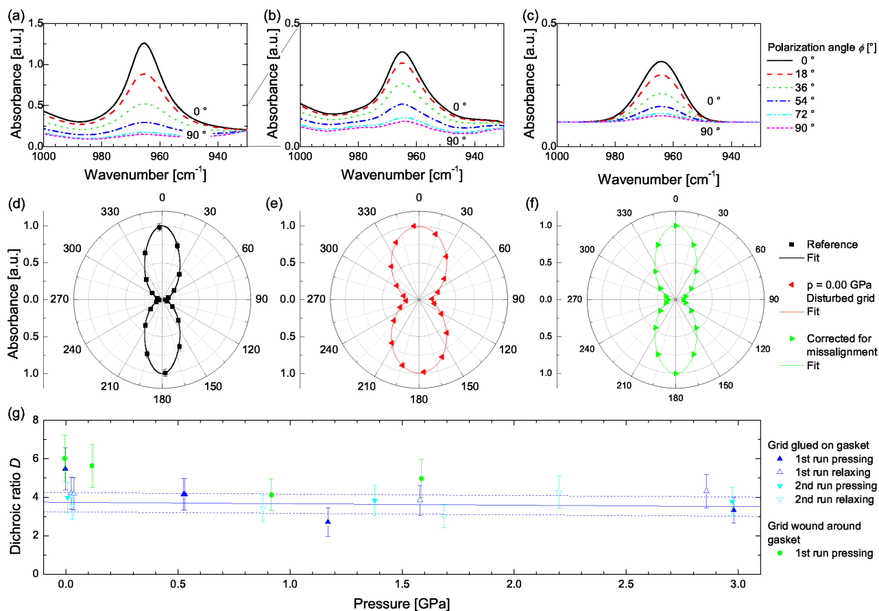
Fig. 3 Polarization-dependent spectra showing IR-dichroism of the band located at 965 cm -1 representing the alanine moiety (a) for a fresh, native reference sample (wound around rods), (b) after closing the DAC at 0.00 GPa, and (c) recalculated by correcting for the geometrical distortion of the grating. (d - f) Polar representation of (a), (b), and (c) normalized to 1 along with fits according to Equation 1. (g) Apparent dichroic ratio D depending on the applied hydrostatic pressure. The blue line represents a linear fit, while the dashed lines correspond to D \pm 0.5 .
